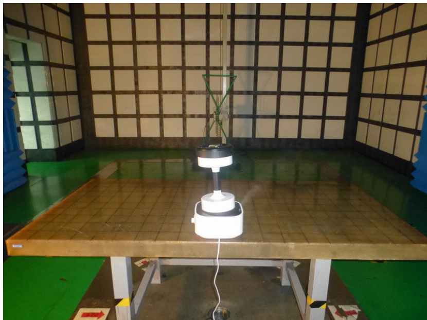
Radiated Emission (30MHz -1GHz) Setup photo Back
