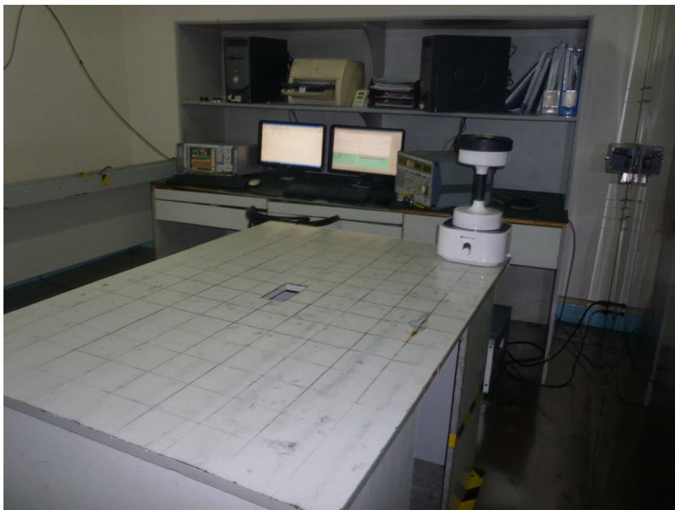
Conducted Emission Setup photo back
