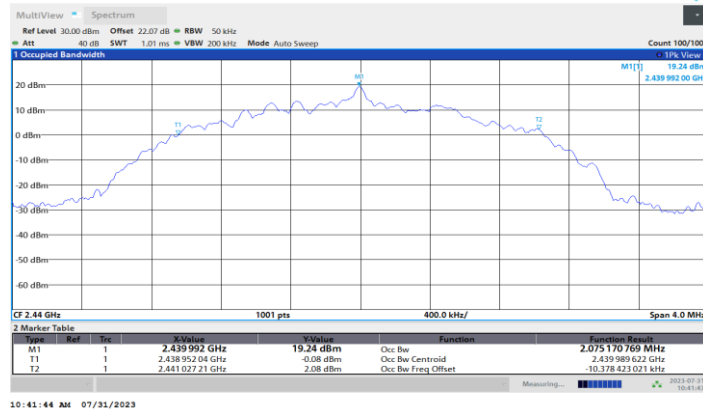
BLE_2M_Ant1_2440
