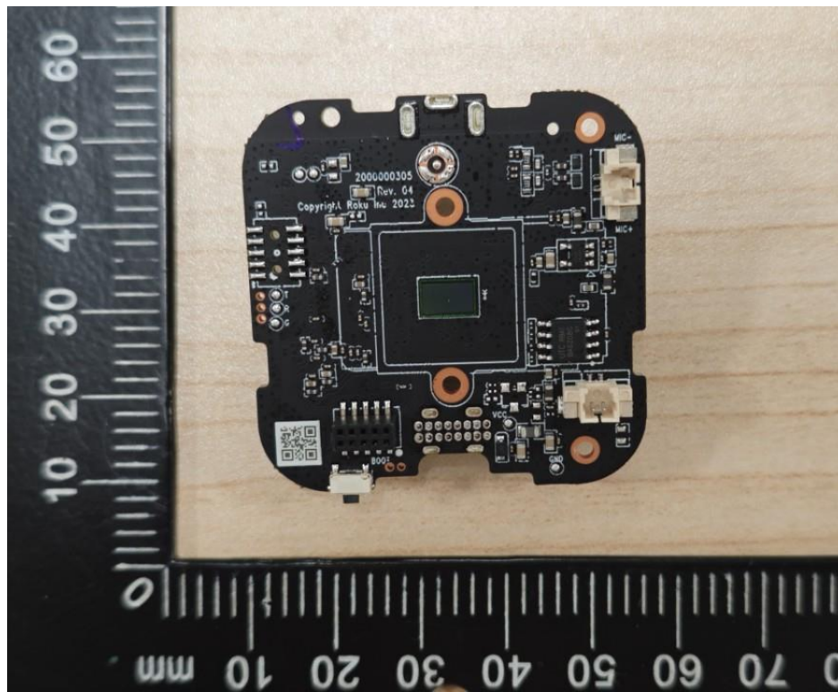
Internal View of EUT-8
