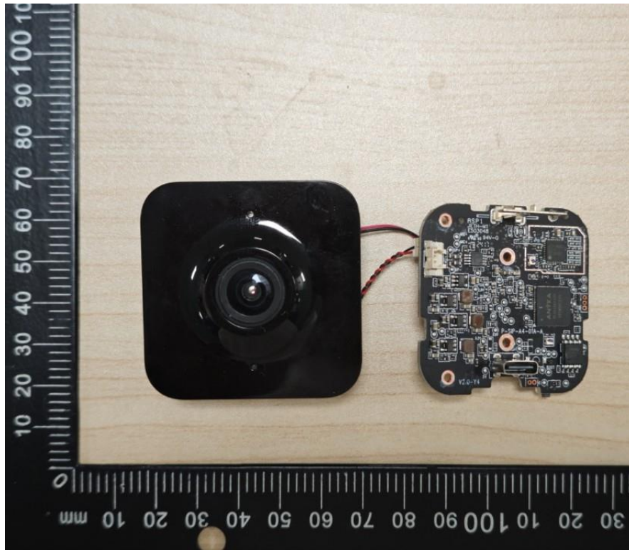
Internal View of EUT-4
