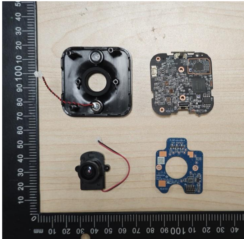
Internal View of EUT-6
