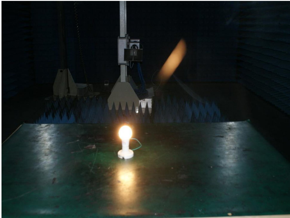
Photograph 8: Set-up for Radiated Emission (1GHz ~ 6GHz)
