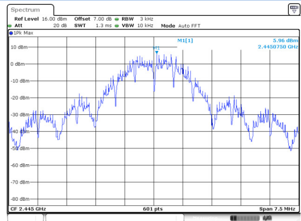
O-QPSK MIDDLE CHANNEL
