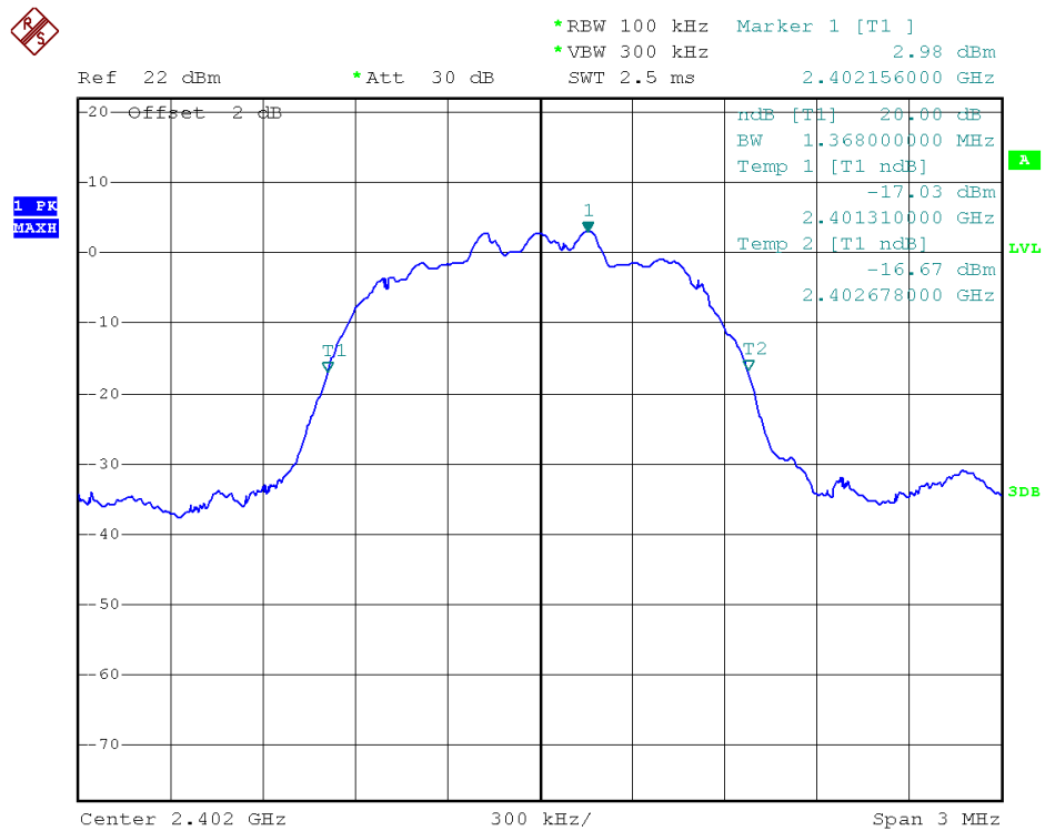
0 Channel @ 8-DPSK
