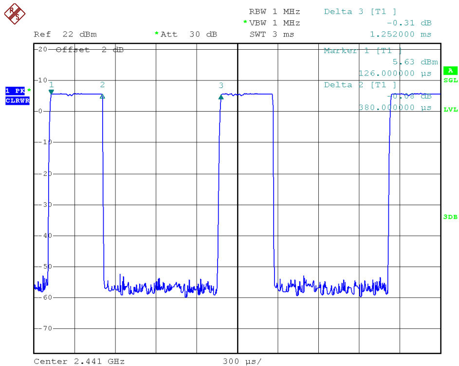
39 Channel @ 2DH1
