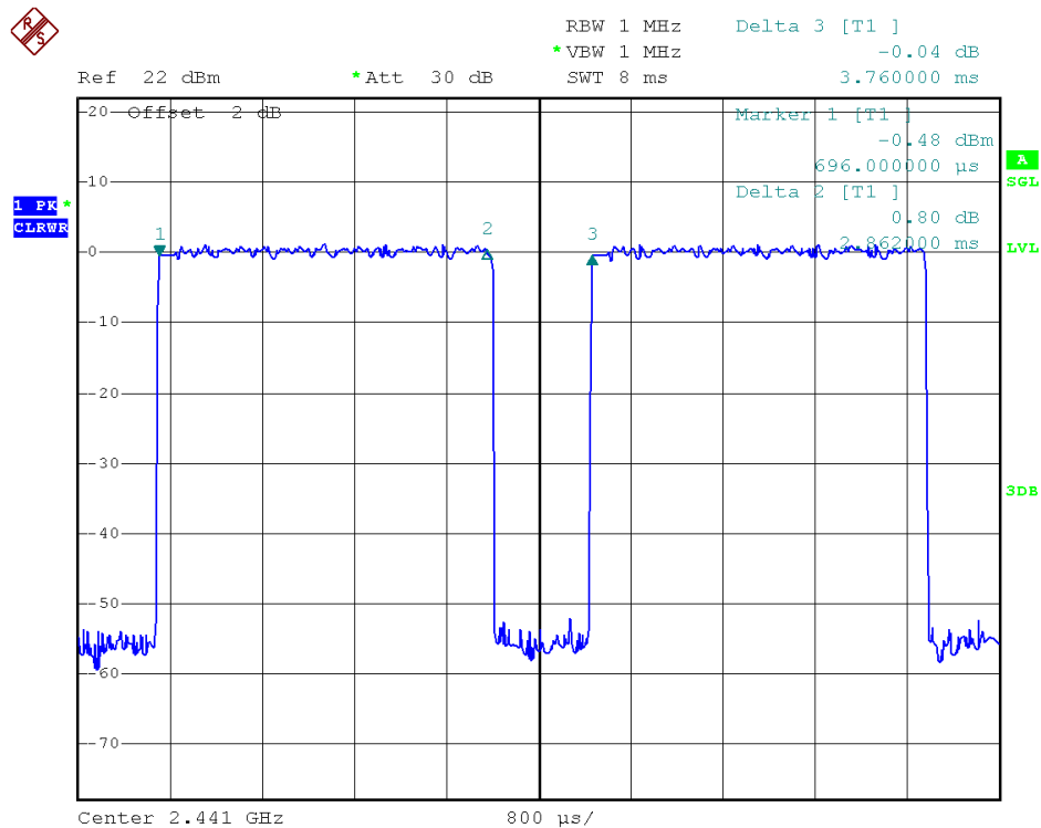
39 Channel @ 2DH5
