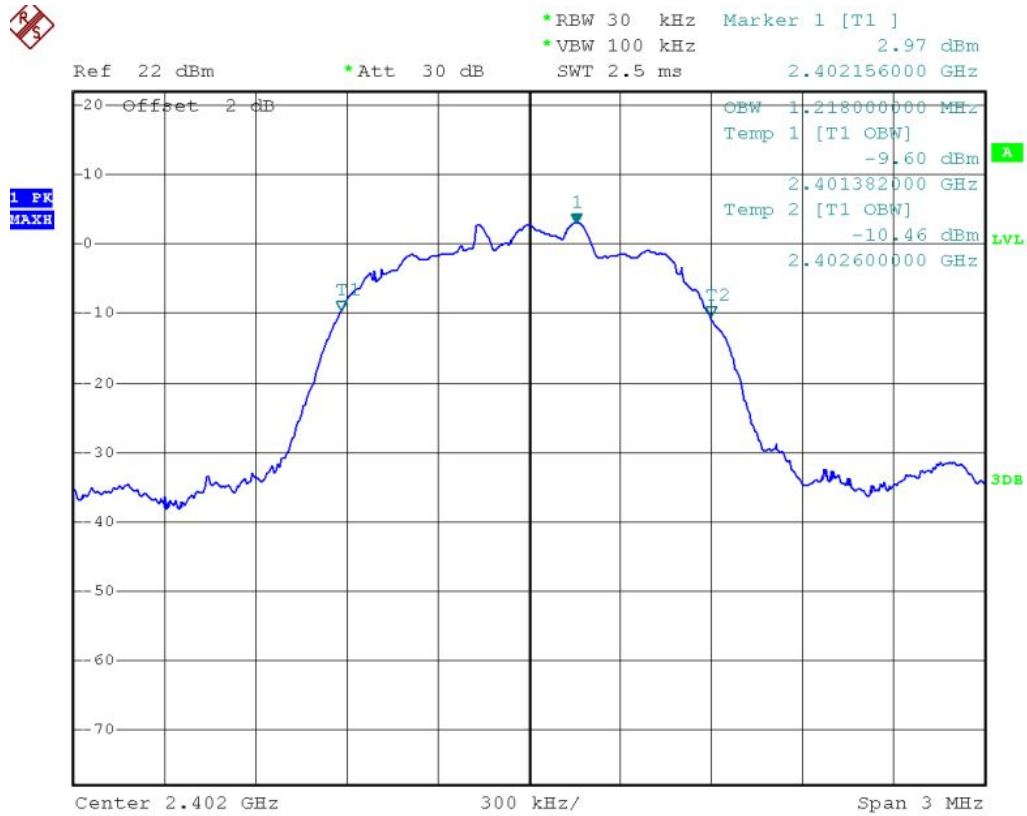
0 Channel @ 8-DPSK
