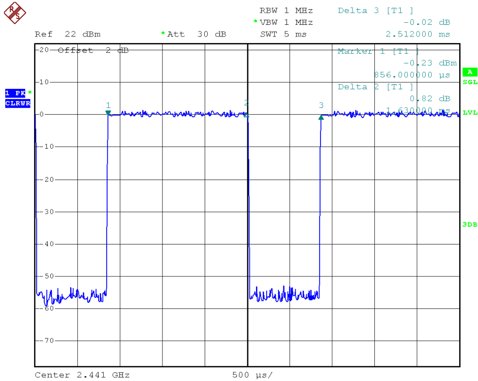
39 Channel @ 2DH3
