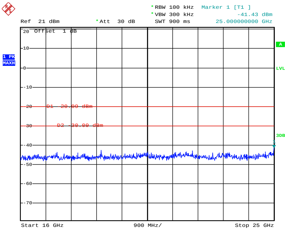
(Plot 4.6.1 A3: Channel 1: 2412MHz @ 802.11b)
