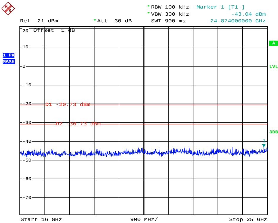
(Plot 4.6.1 C3: Channel 11: 2462MHz @ 802.11b)
