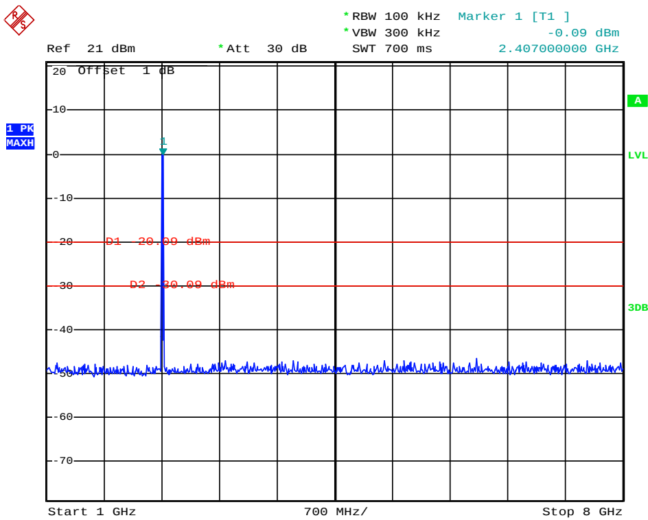
(Plot 4.6.1 A1: Channel 1: 2412MHz @ 802.11b)
