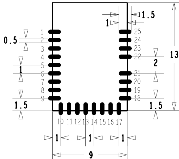
Figure 2 Physical dimensions and pinout (mm)
