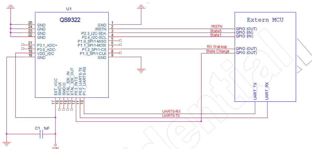
Figure 6 Reference circuit schematic
