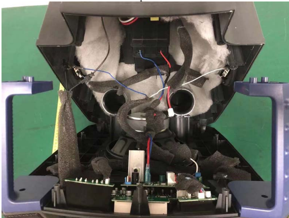
Internal Photos M/N: Explorer™ XL
