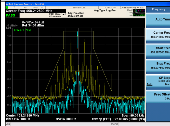
Emission Mask D@406.125MHz-5W-4FSK
