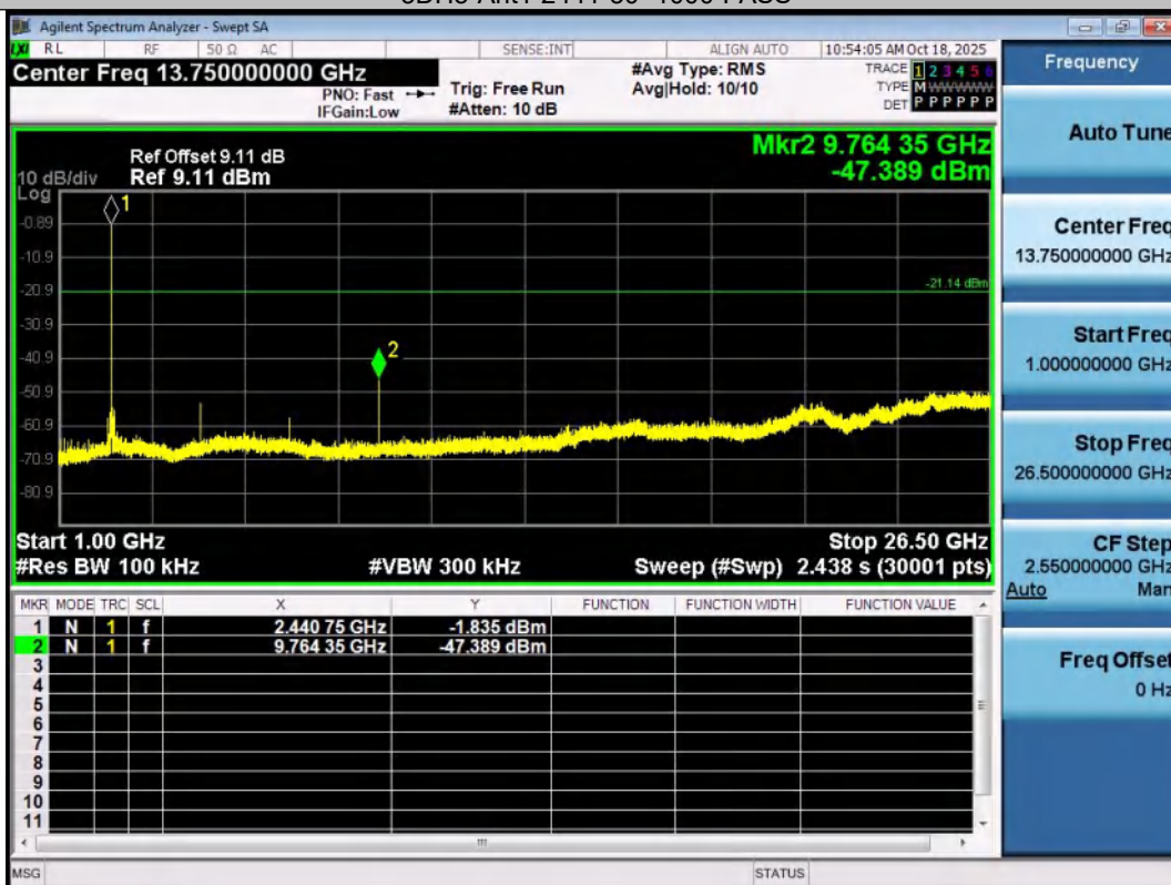
3DH5-Ant1-2441-1000~26500-PASS
