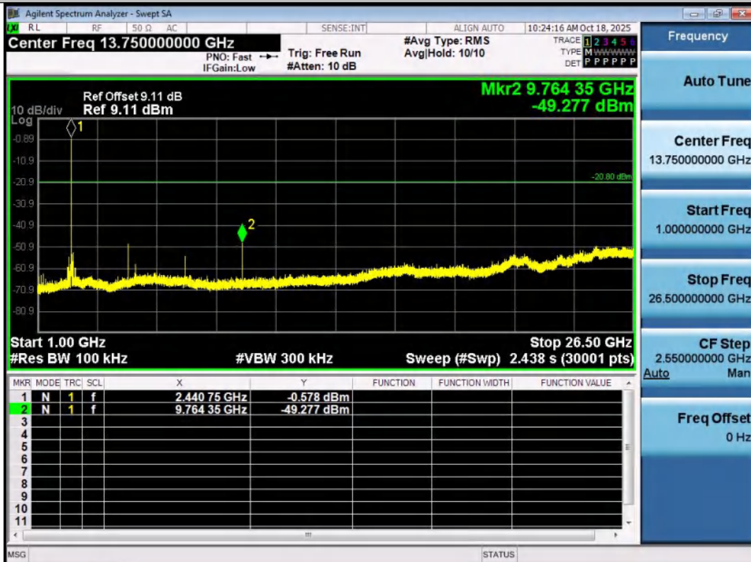
DH5-Ant1-2441-1000~26500-PASS
