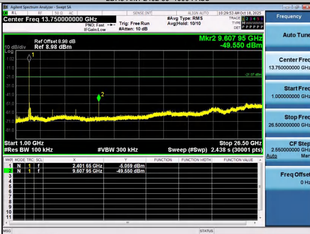
2DH5-Ant1-2402-1000~26500-PASS
