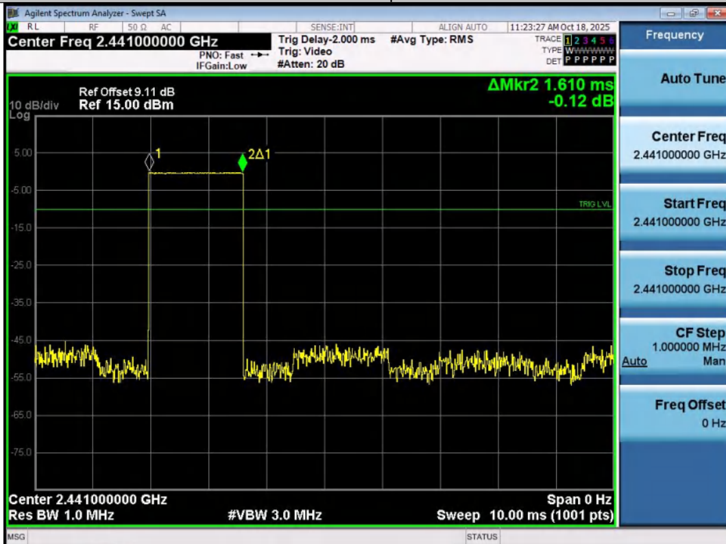
DH3-Ant1-Hop-PASS
