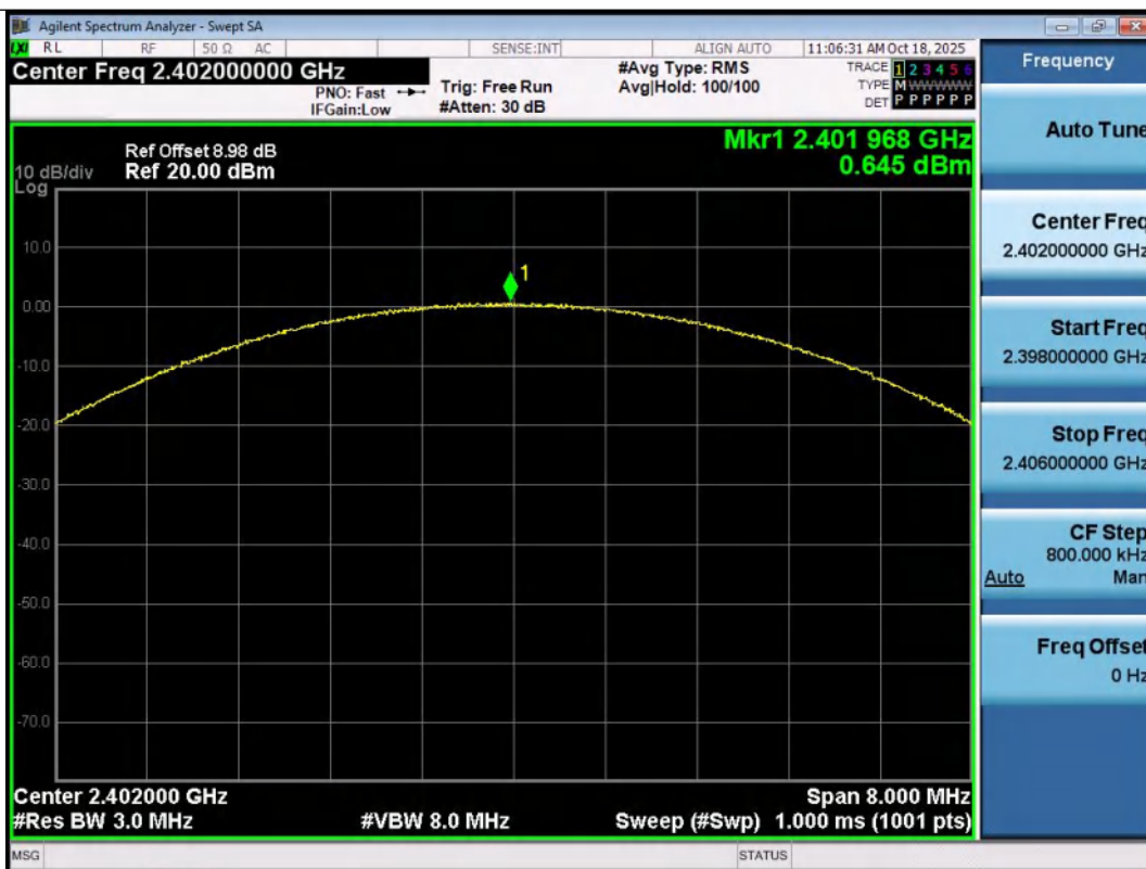
3DH5-Ant1-2402-PASS
