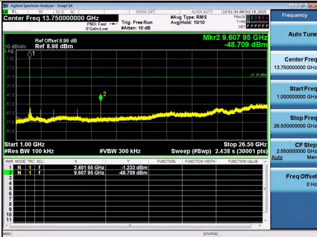
3DH5-Ant1-2402-1000~26500-PASS
