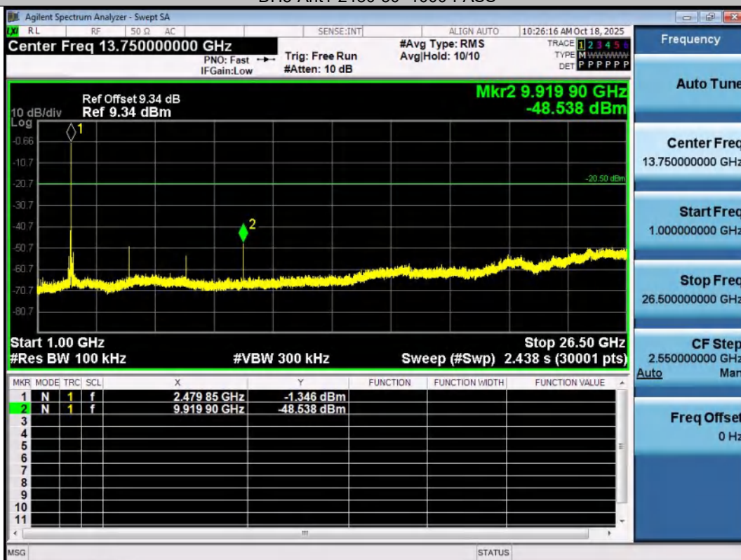
DH5-Ant1-2480-1000~26500-PASS
