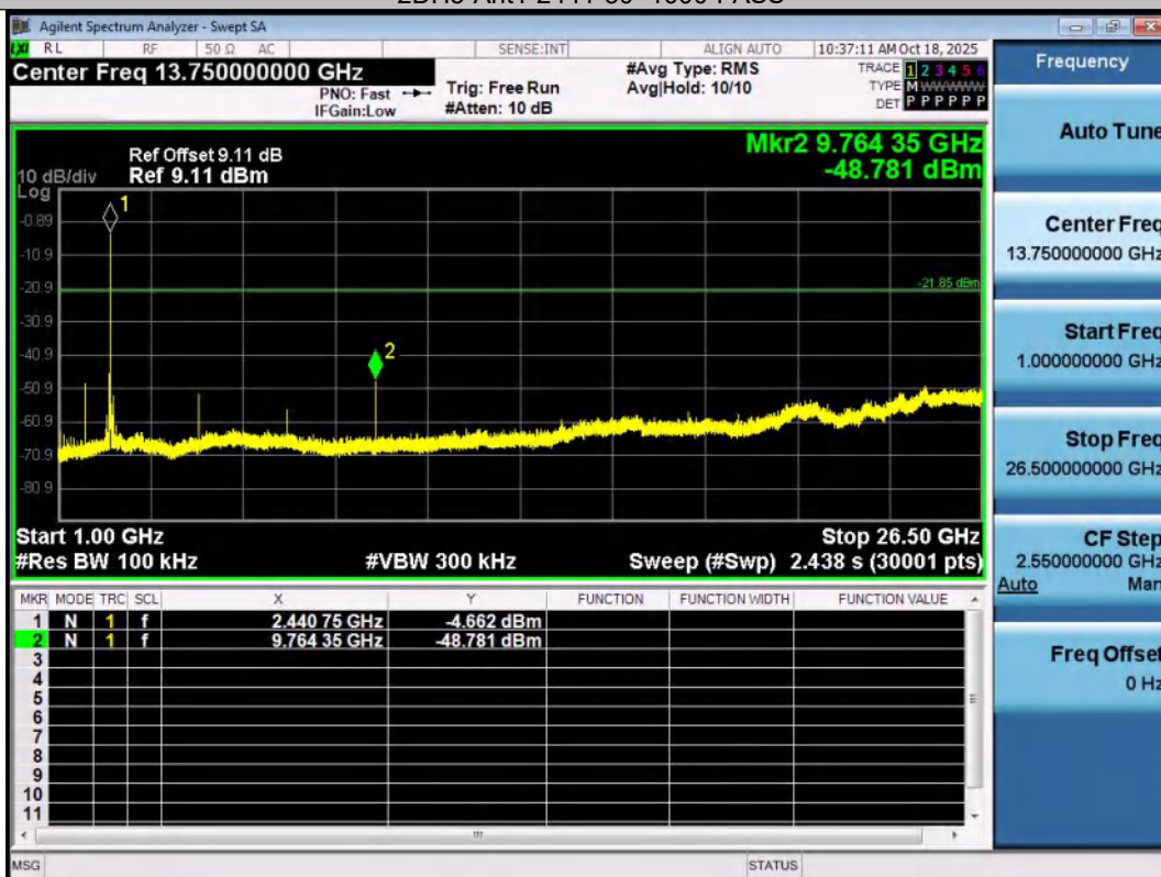
2DH5-Ant1-2441-1000~26500-PASS
