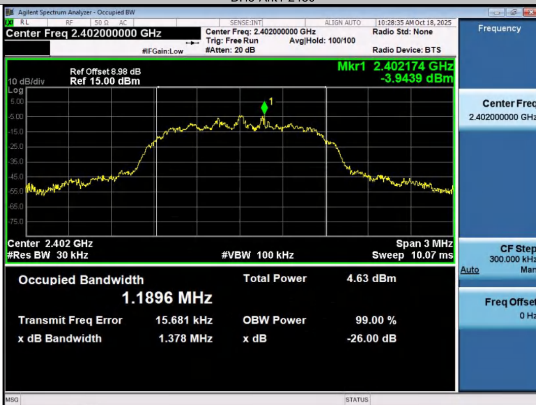
2DH5-Ant1-2402
