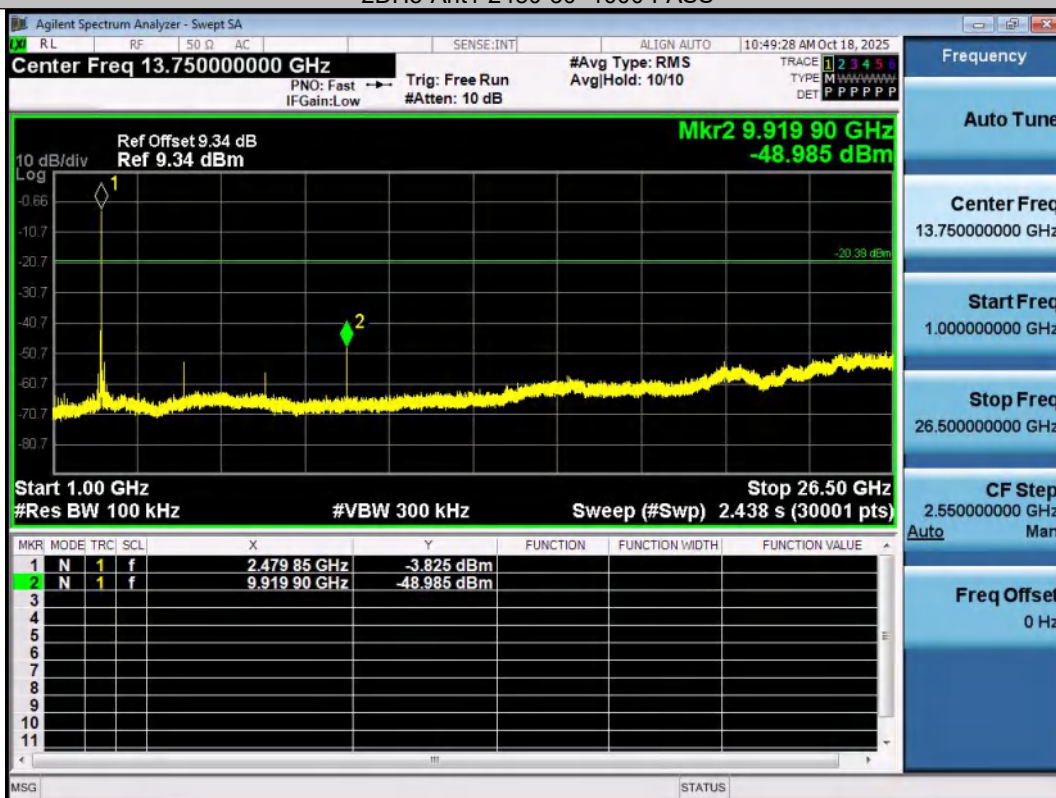
2DH5-Ant1-2480-1000~26500-PASS
