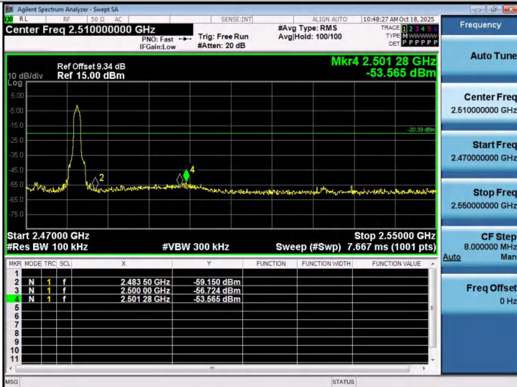
2DH5-Ant1-2480-PASS
