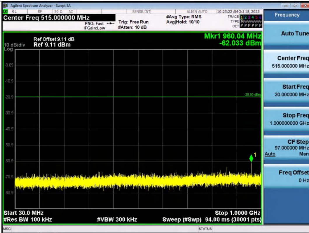
DH5-Ant1-2441-30~1000-PASS
