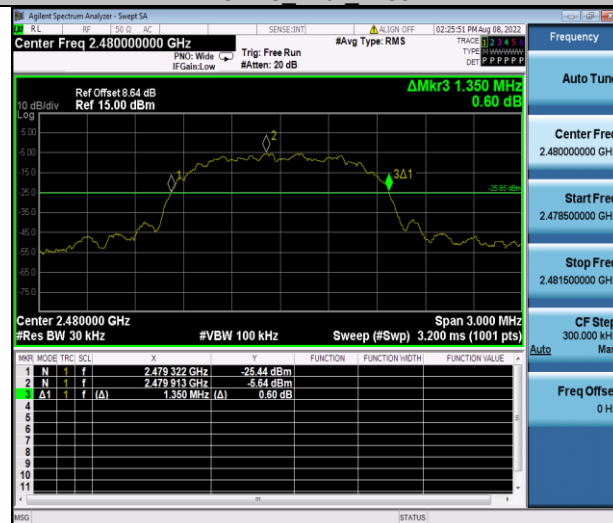
3DH5 Ant1_2480
