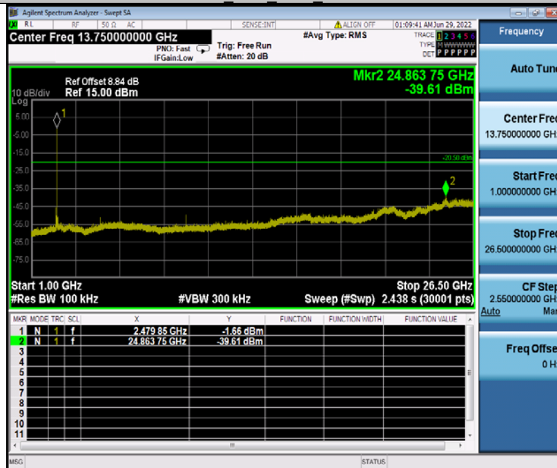
3DH5_Ant1_2480_1000~26500
