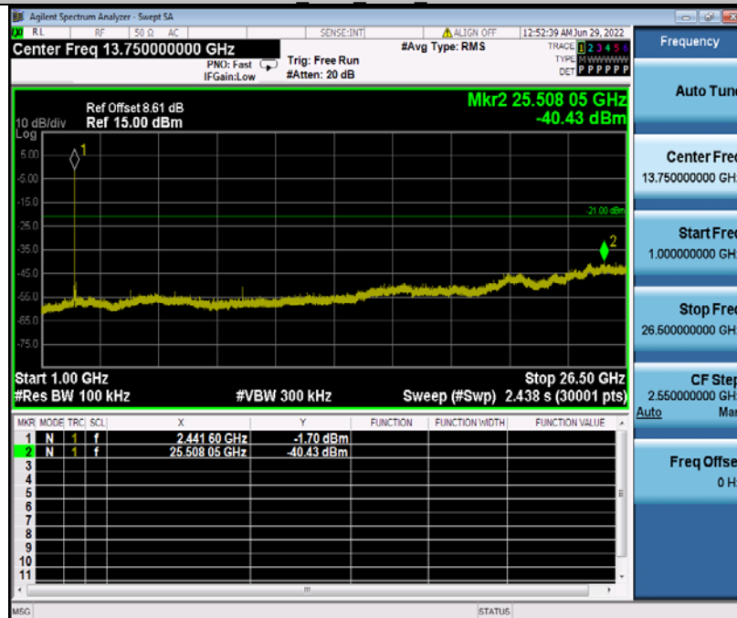
2DH5_Ant1_2441_1000~26500
