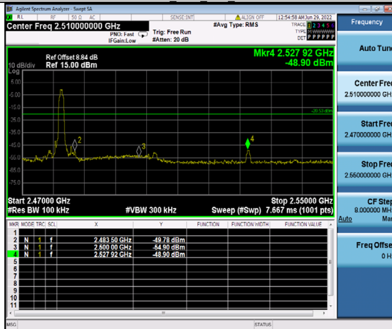
2DH5 Ant1_High 2480
