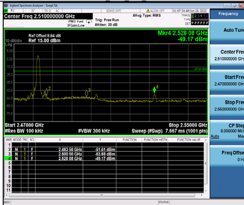
3DH5 Ant1_High 2480
