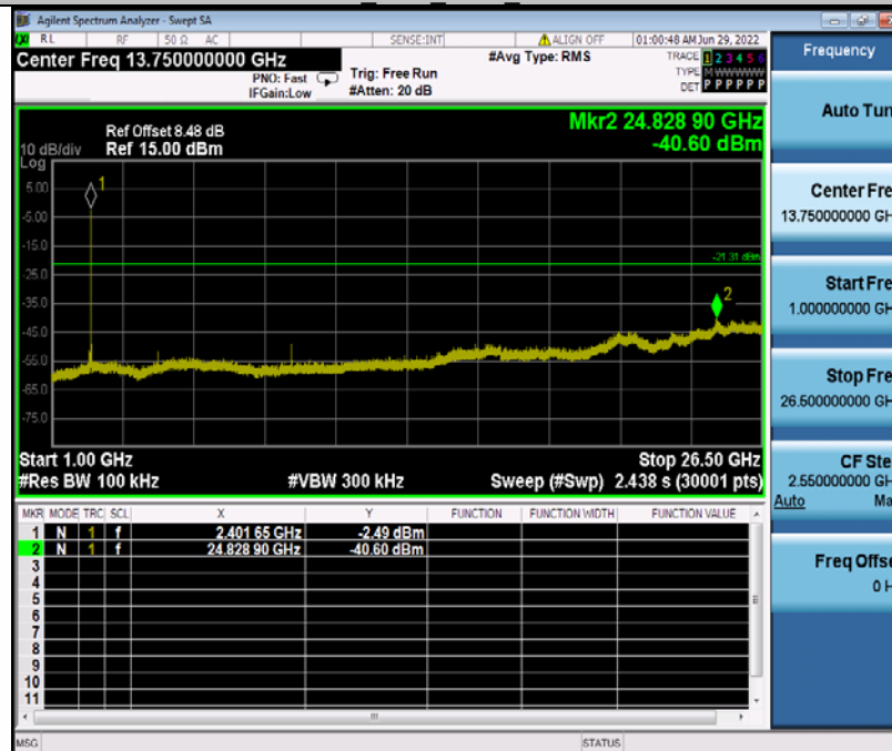
3DH5_Ant1_2402_1000~26500
