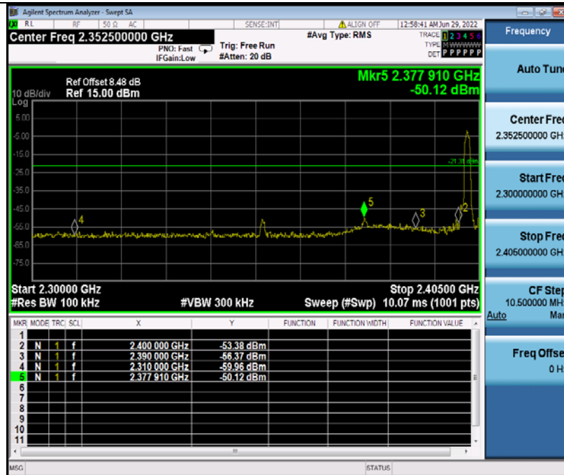
3DH5 Ant1_Low 2402
