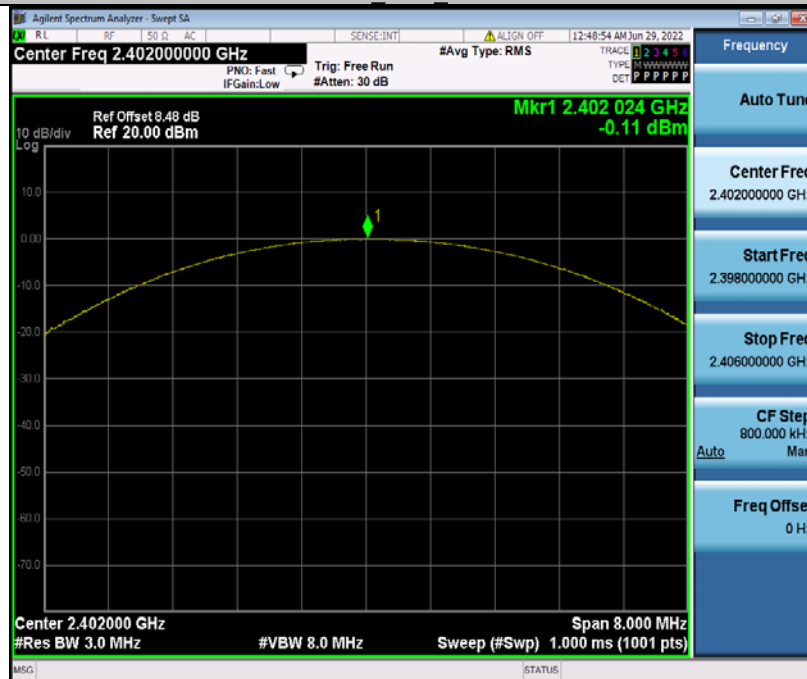
2DH5_Ant1_2402
