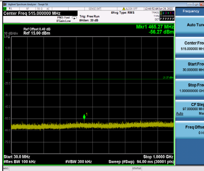
2DH5_Ant1_2402_30~1000
