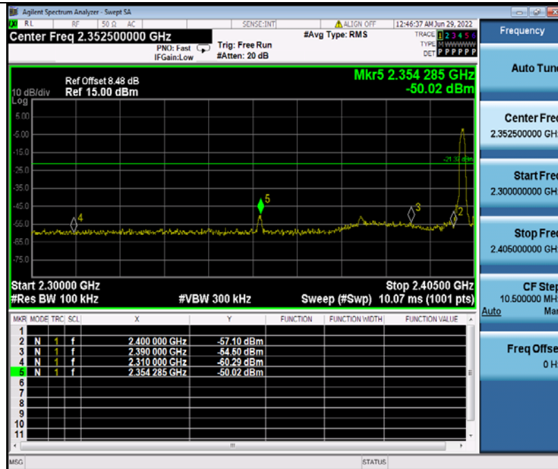
2DH5 Ant1_Low 2402
