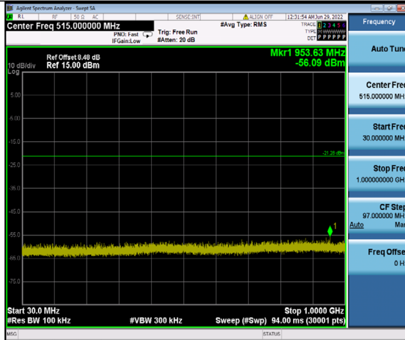
DH5 Ant1_2402_30~1000
