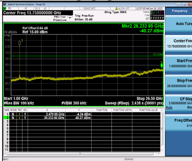
2DH5_Ant1_2480_1000~26500
