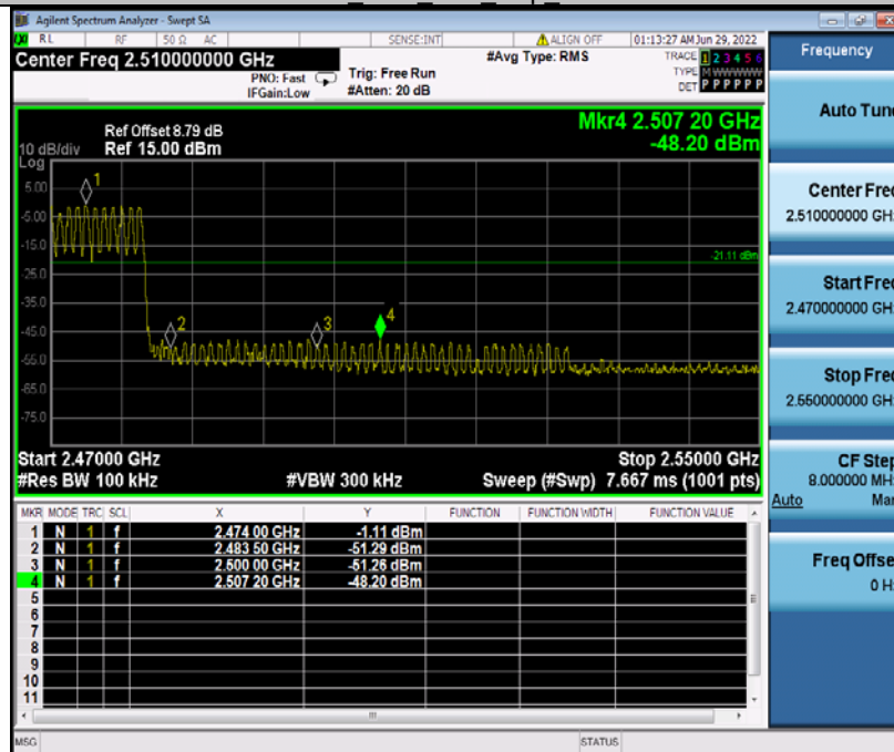
DH5_Ant1_High_Hop_2480
