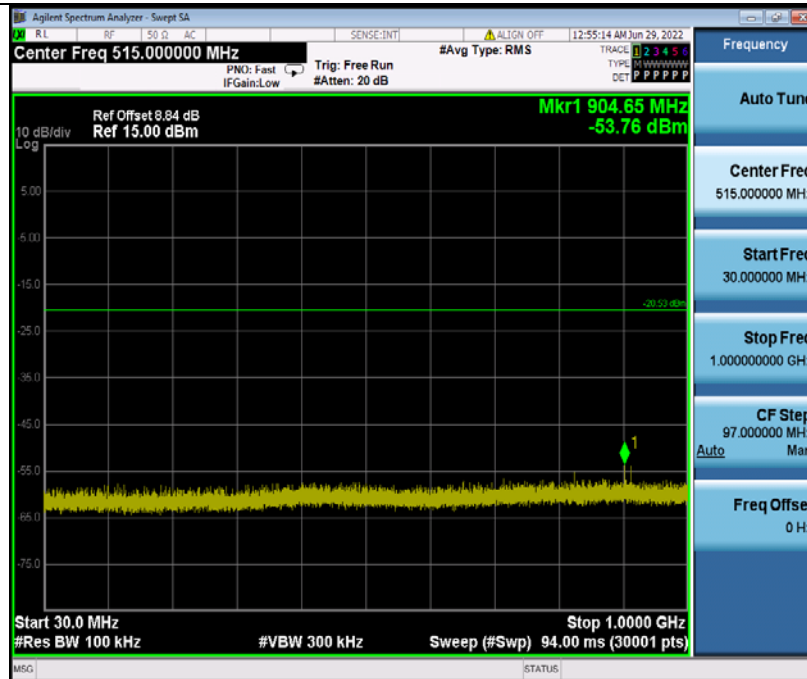
2DH5_Ant1_2480_30~1000
