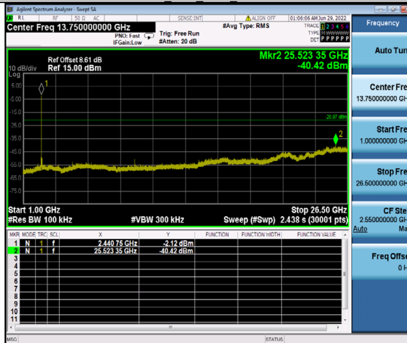
3DH5_Ant1_2441_1000~26500
