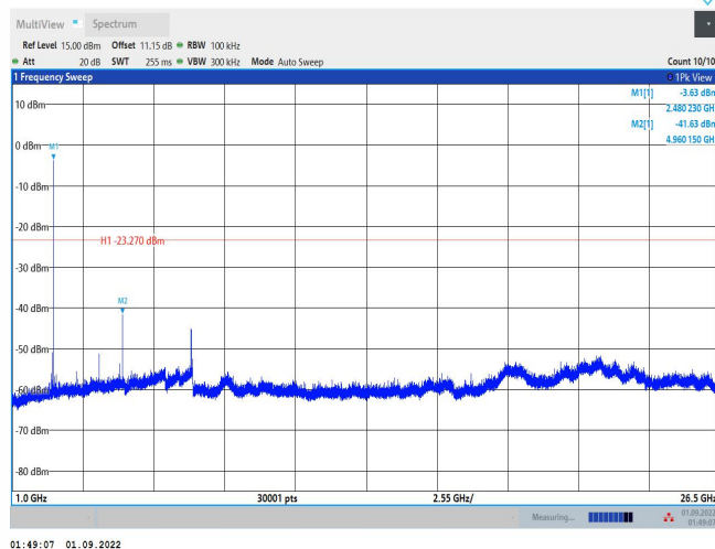
3DH5_Ant1_2480_1000~26500
