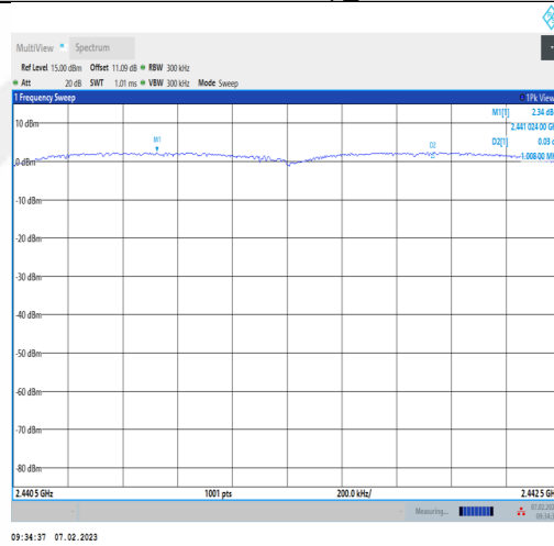
3DH5-Ant1-Hop_2441
