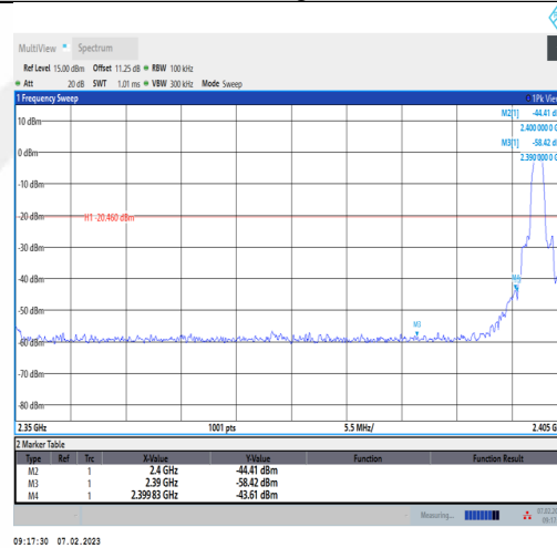
3DH5-Ant1-Low-2402--0.46
