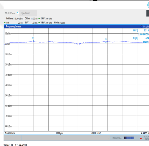
2DH5-Ant1-Hop_2441
