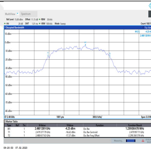
3DH5-Ant1-2480
