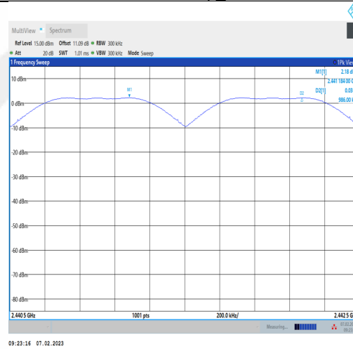
DH5-Ant1-Hop_2441
