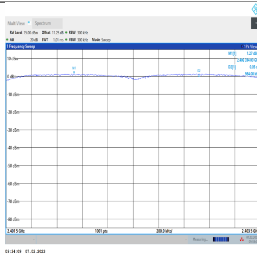
3DH5-Ant1-Hop_2402
