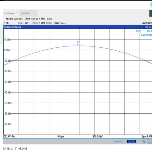
3DH5-Ant1-2441
