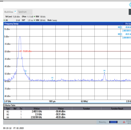
2DH5-Ant1-High-2480-0.31
