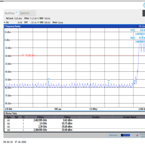
DH5-Ant1-Low-Hop_2402-0.42
