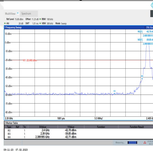
2DH5-Ant1-Low-2402--0.44
