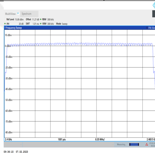
3DH5-Ant1-Hop
