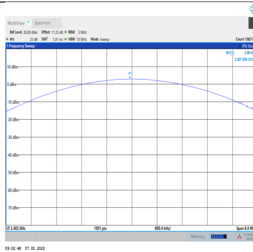
3DH5-Ant1-2402
