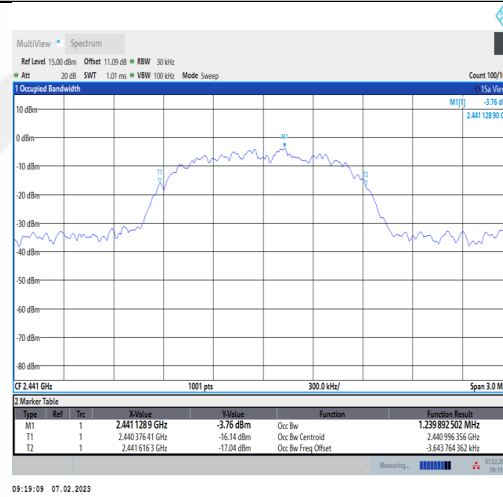
3DH5-Ant1-2441
