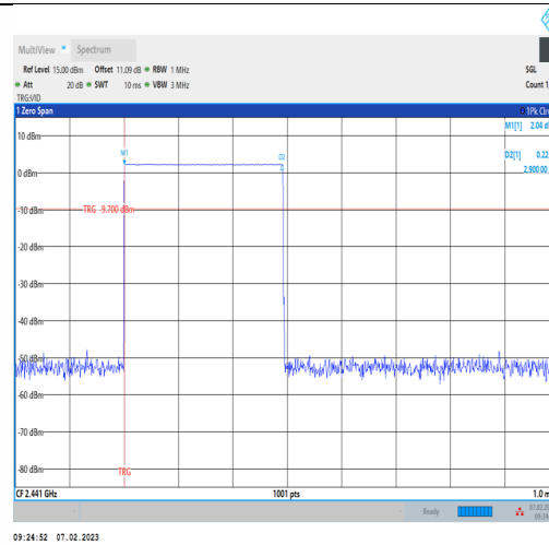
DH5-Ant1-Hop-2.900-106.67
