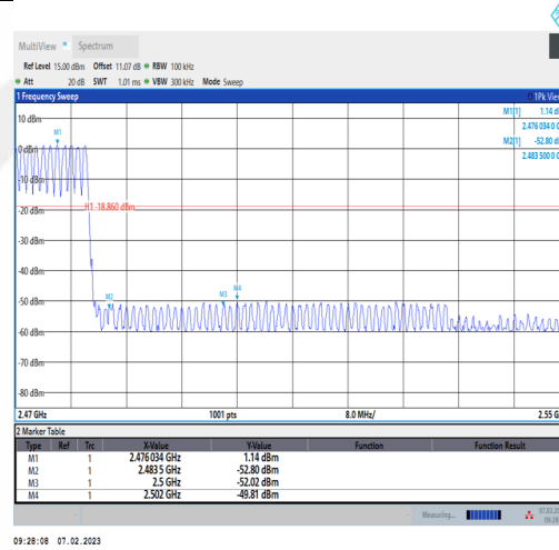
DH5-Ant1-High-Hop_2480-1.14
