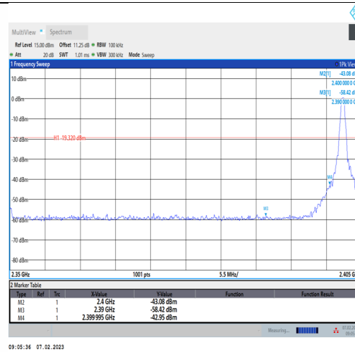
DH5-Ant1-Low-2402-0.68
