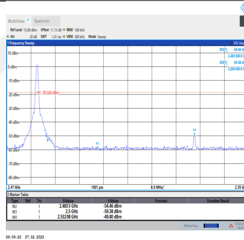
DH5-Ant1-High-2480-1.44
