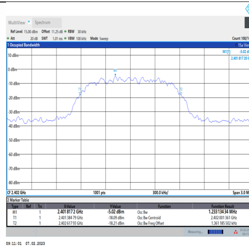
2DH5-Ant1-2402
