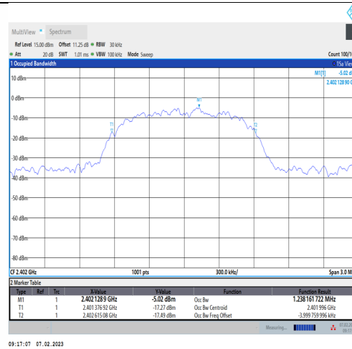
3DH5-Ant1-2402
