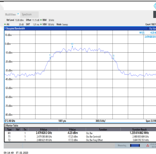
2DH5-Ant1-2480
