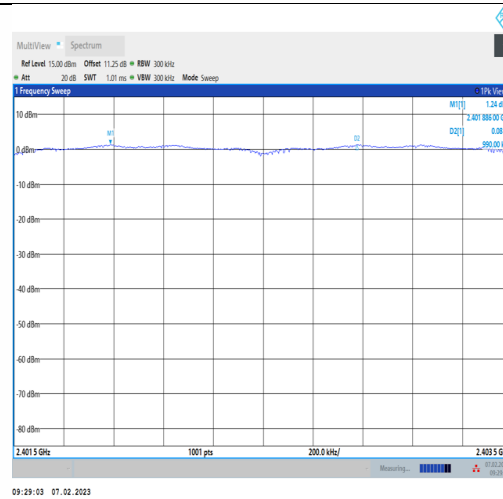
2DH5-Ant1-Hop_2402
