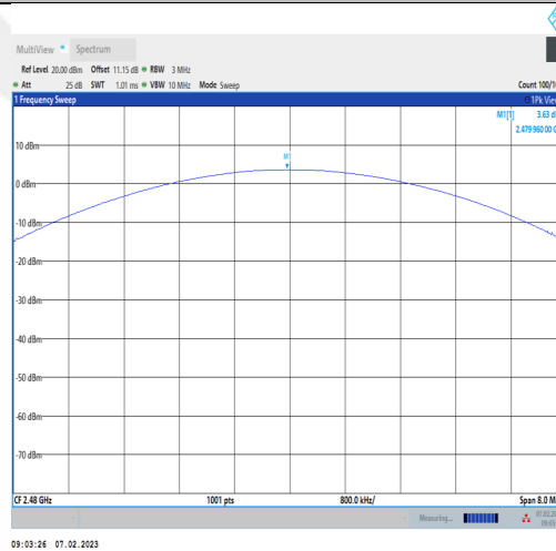
3DH5-Ant1-2480
