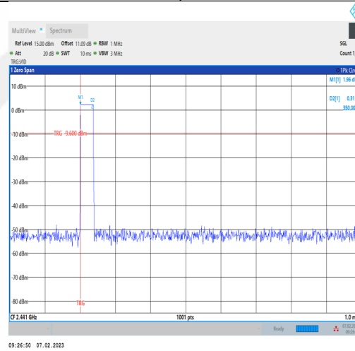
DH1-Ant1-Hop-0.350-320
