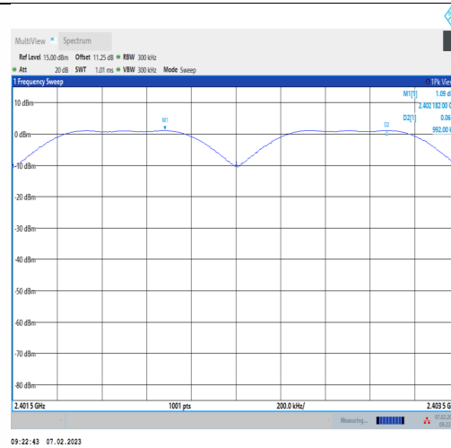
DH5-Ant1-Hop_2402
