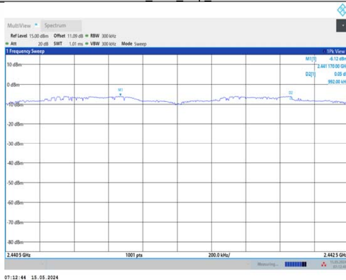
2DH5_Ant1_Hop_2441
