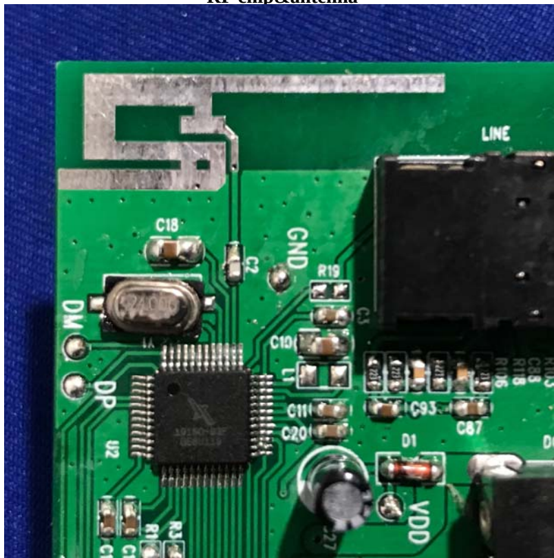
RF chip
