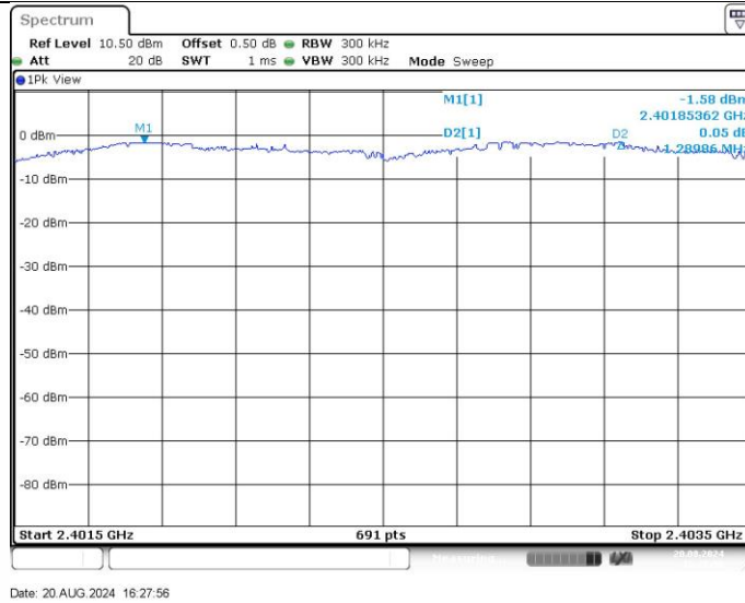
3DH5_Ant1_Hop_2402
