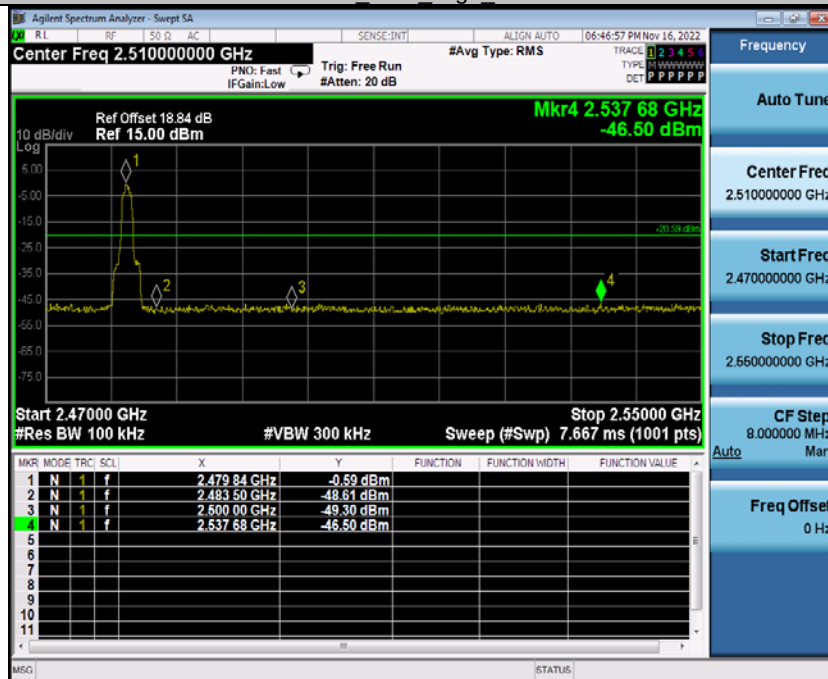
3DH5_Ant1_High_2480
