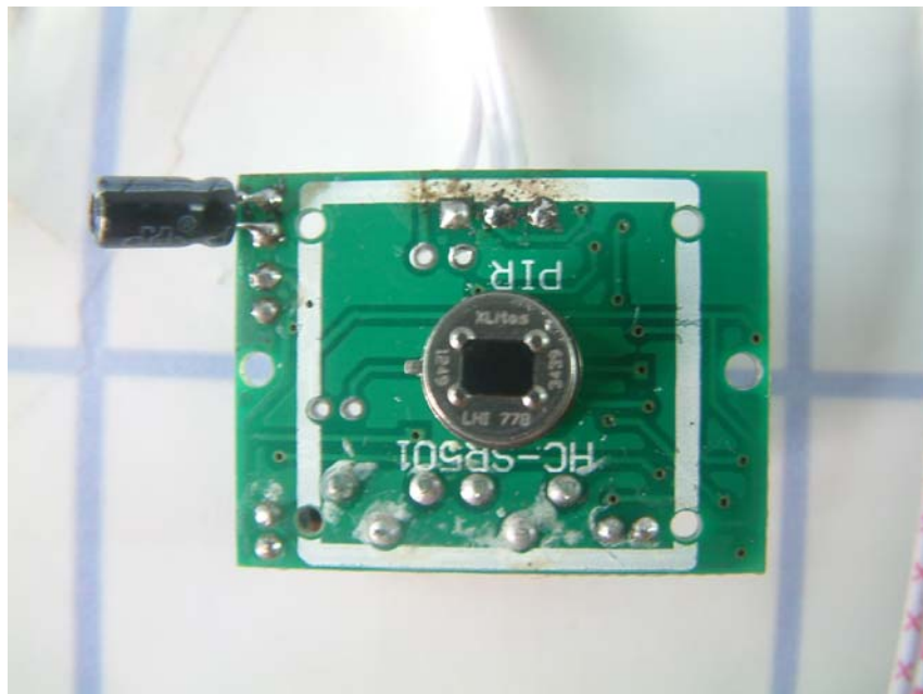
PCB 4 side 2
