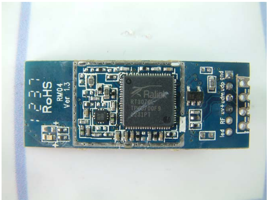
Module view 3
