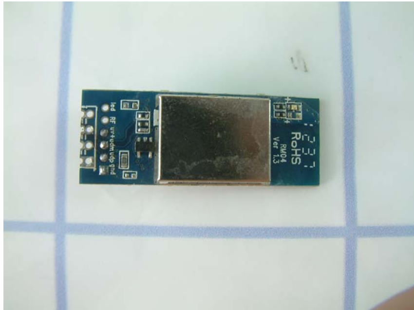
Module view 1
