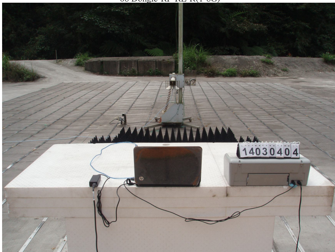
06 Dongle-RF-RE-R(1-6G)
