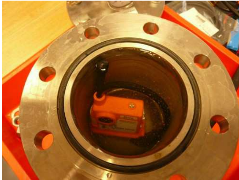
Figure A.3 – EUT in the pressure test vessel
