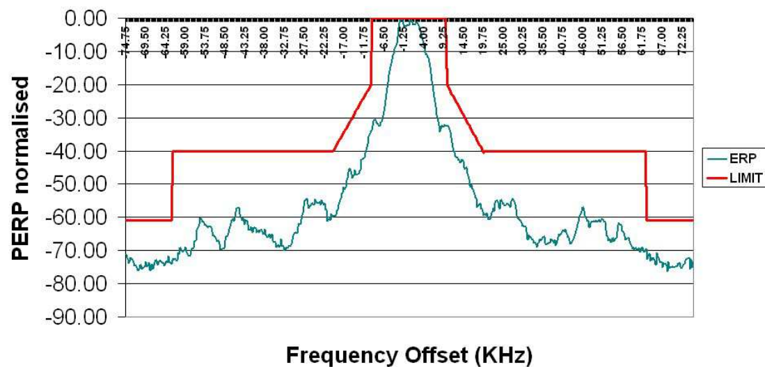
Figure C.2 – Spectrum AIS2 @ -20°C
