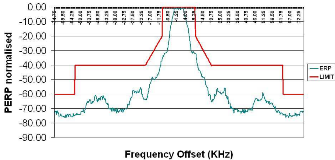
Figure C.1 – Spectrum AIS1 @ -20°C
