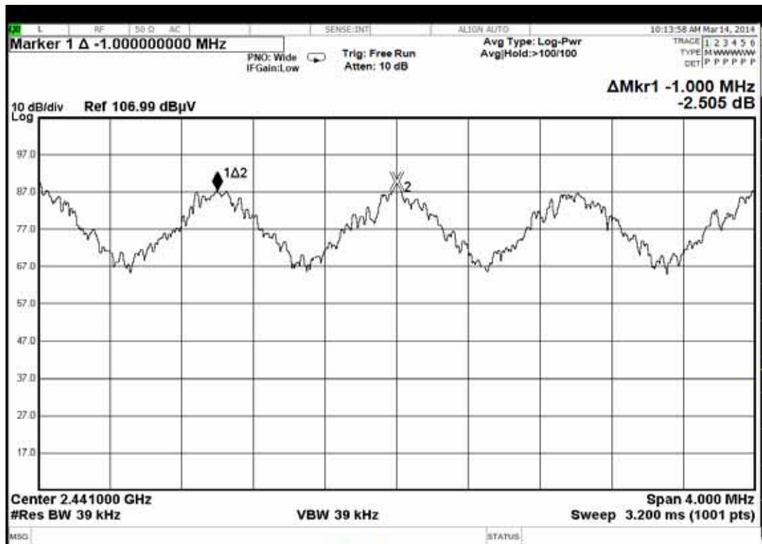
Figure 2: GFSK, 2441MHz adjacent channel of right carrier frequency separation
