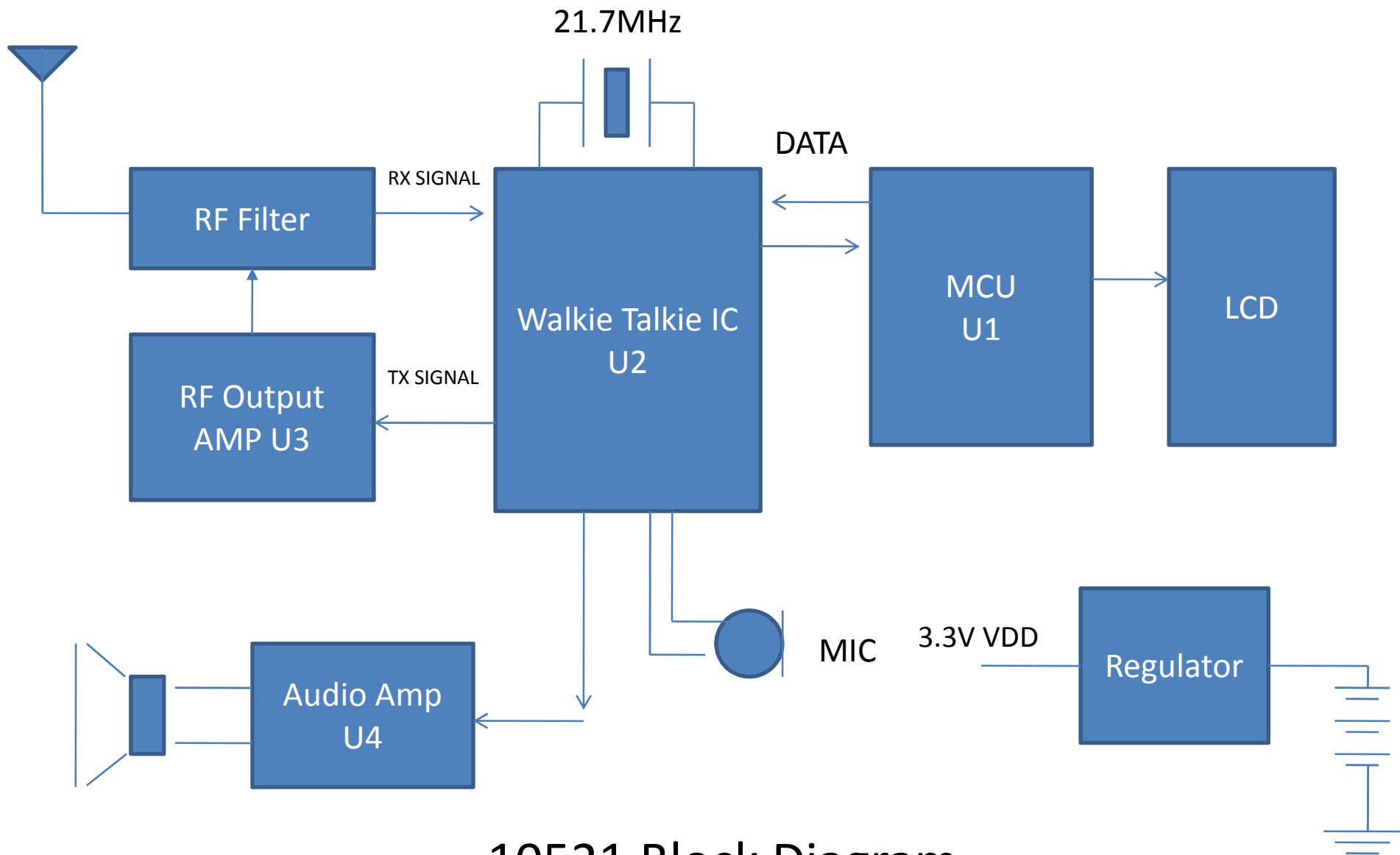
10521 Block Diagram
