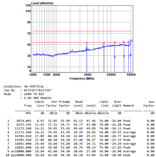
2.4G_SRD_TX_MID_Vertical
