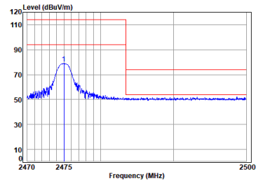
2.4G_SRD_TX_HIGH_Vertical
