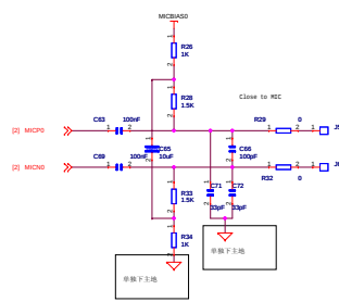
HANDSET MICROPHONE
