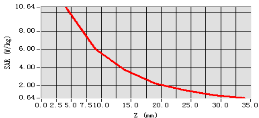
SAR, Z Axis Scan (X = 6, Y = 0)
