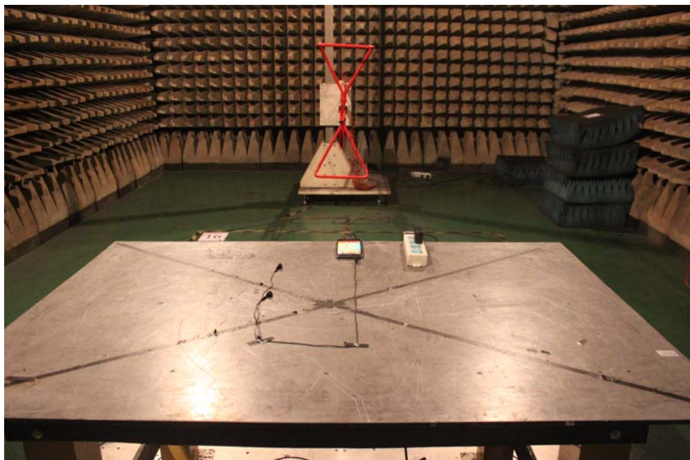
Radiated Emission Test
