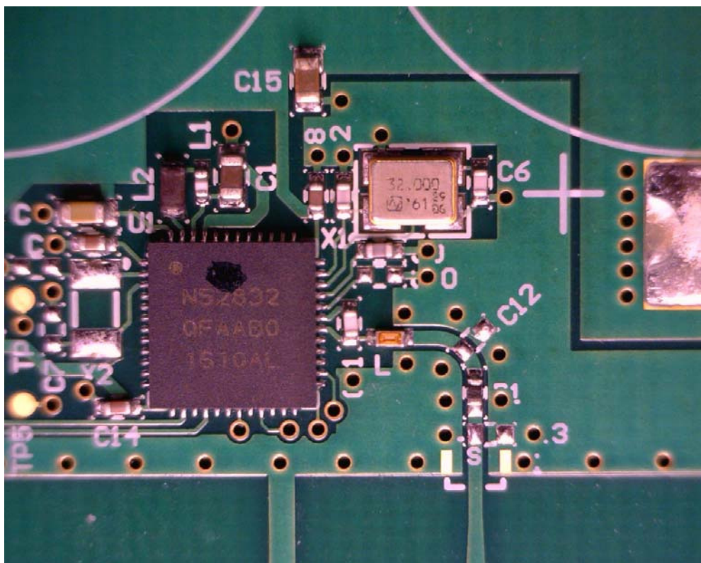
Figure 5 - SwipeSense Badge RF Section
