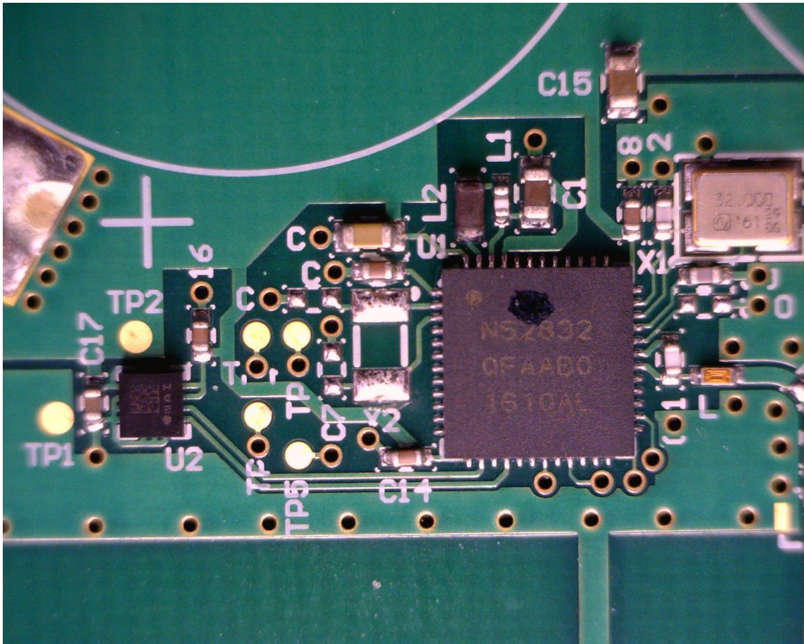
Figure 6 - SwipeSense Badge RF Section
