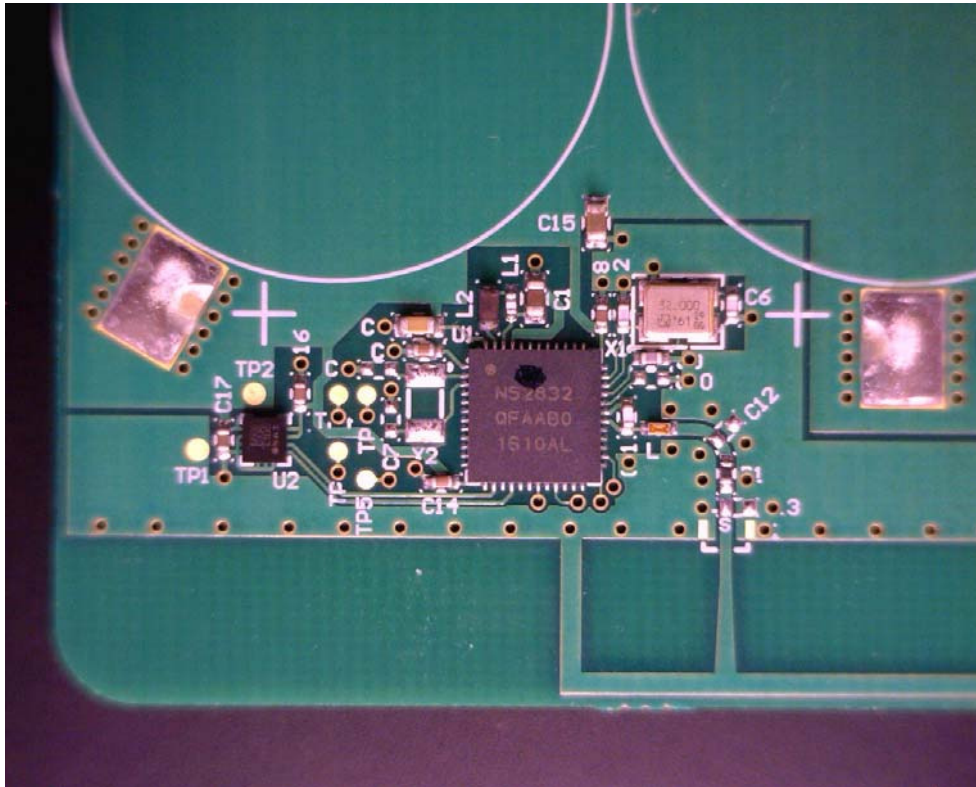
Figure 4 - SwipeSense Badge RF Section
