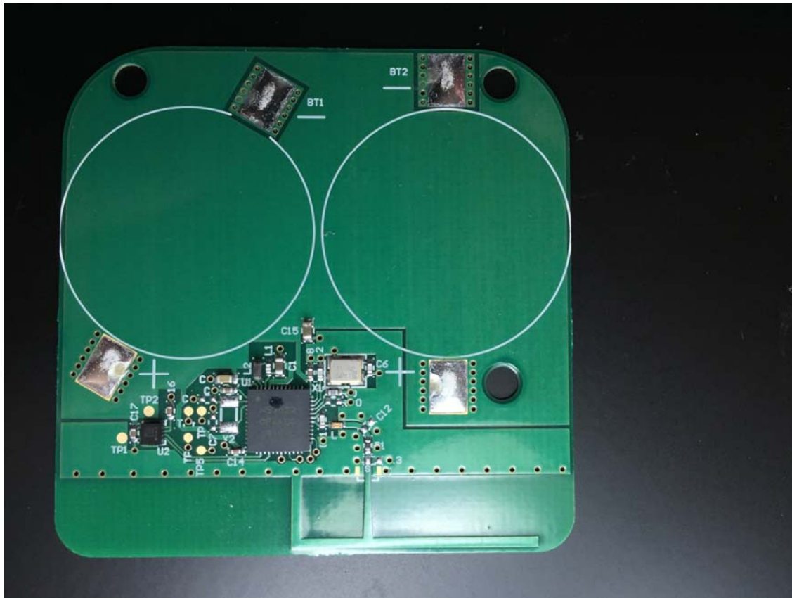
Figure 2 - SwipeSense Badge PWB front side
