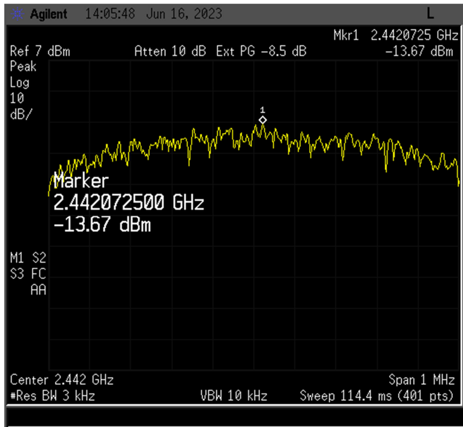
Figure 21. Power Spectral Density, Mid Channel
