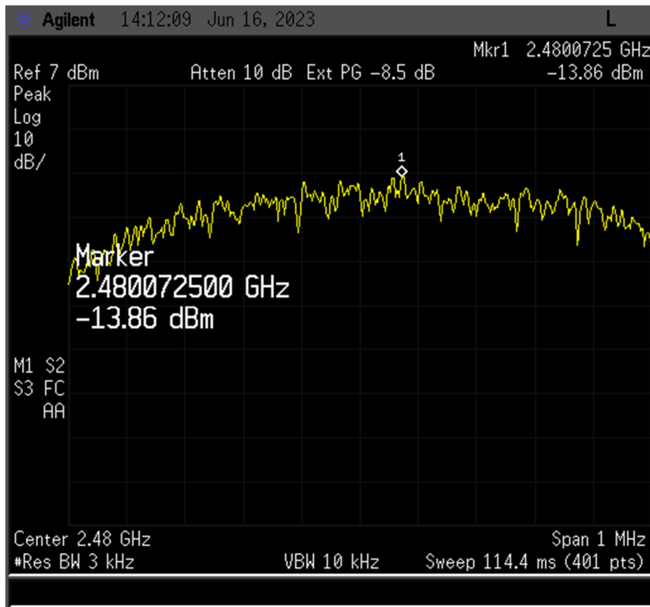
Figure 22. Power Spectral Density, High Channel
