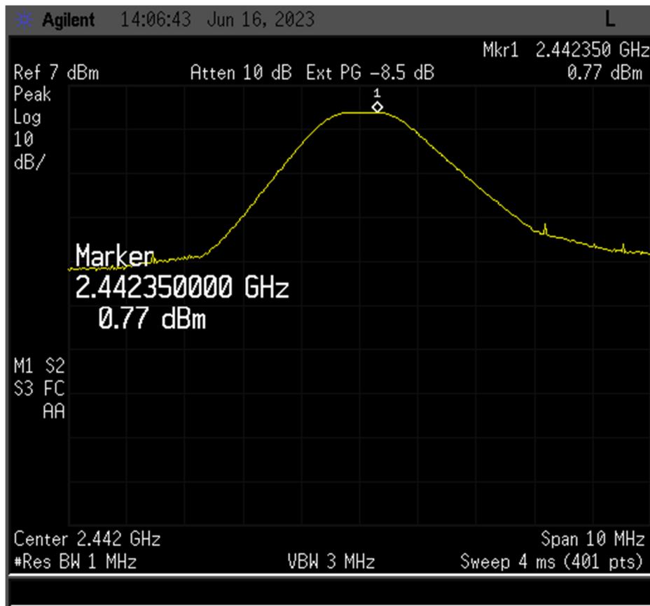
Figure 18. Peak Antenna Conducted Output Power, Mid Channel
