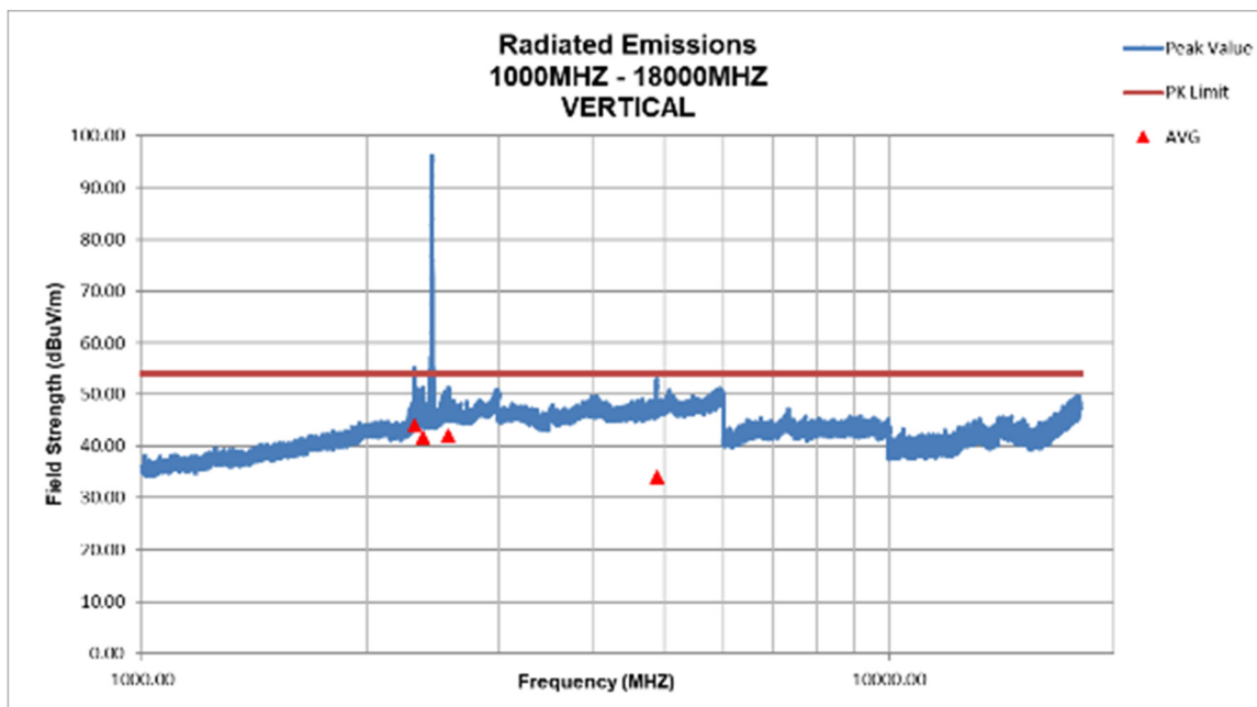
Figure 24. Radiated Emissions, Vertical Above 1000 MHz
