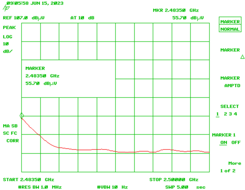
Figure 13. High Channel Restricted Band – Average
