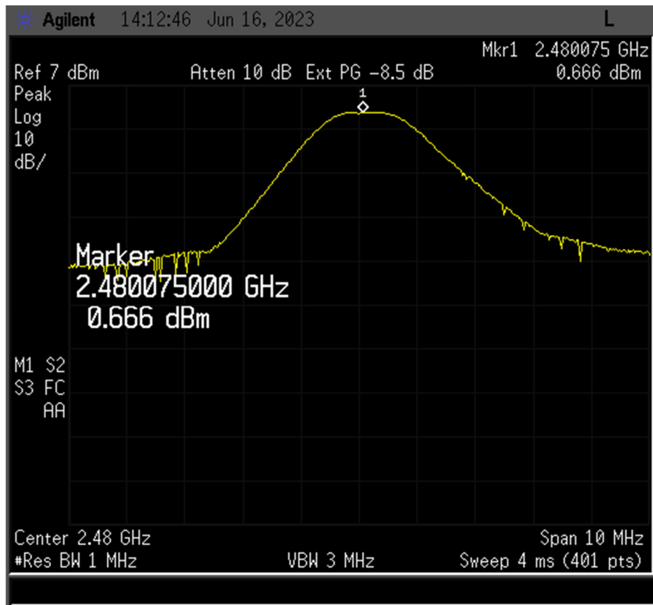
Figure 19. Peak Antenna Conducted Output Power, High Channel
