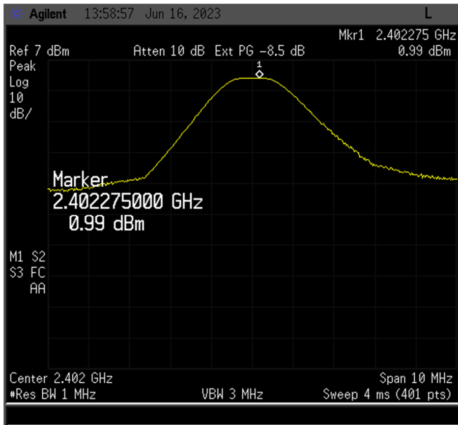
Figure 17. Peak Antenna Conducted Output Power, Low Channel
