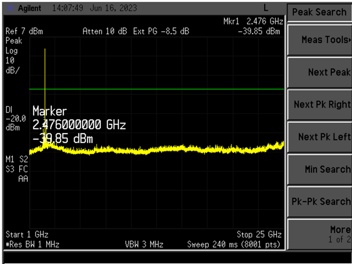
Figure 5. Channel 20, 1 – 25 GHz
