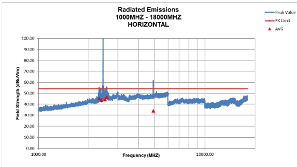
Figure 23. Radiated Emissions, Horizontal Above 1000 MHz
