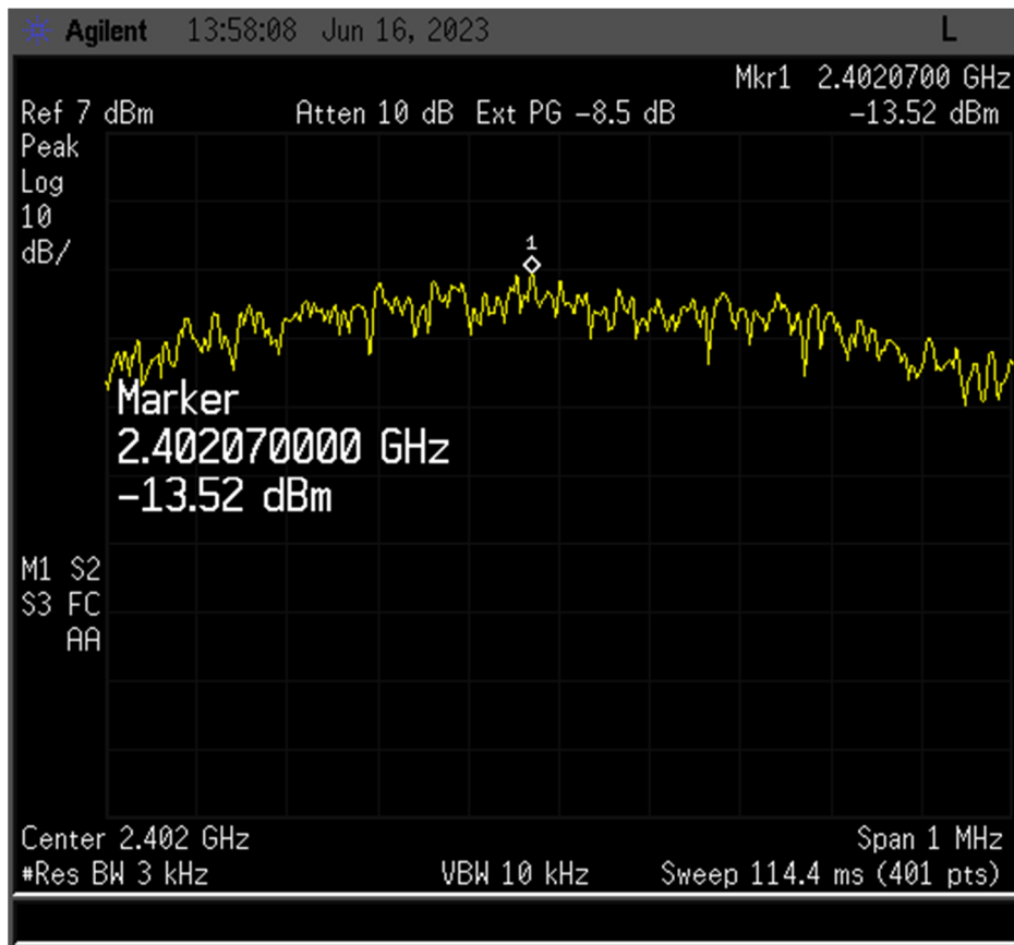
Figure 20. Power Spectral Density, Low Channel
