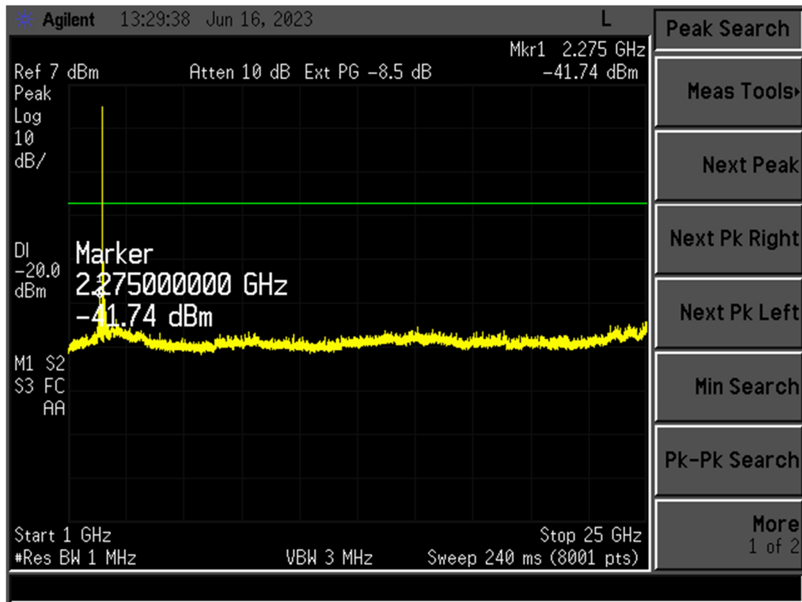
Figure 3. Channel 0, 1 – 25 GHz
