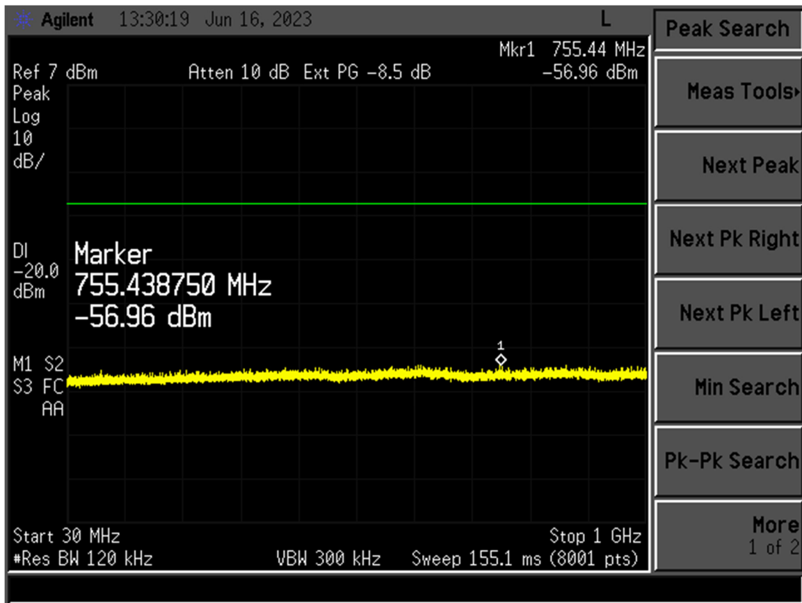
Figure 2. Channel 0, 30-1000 MHz
