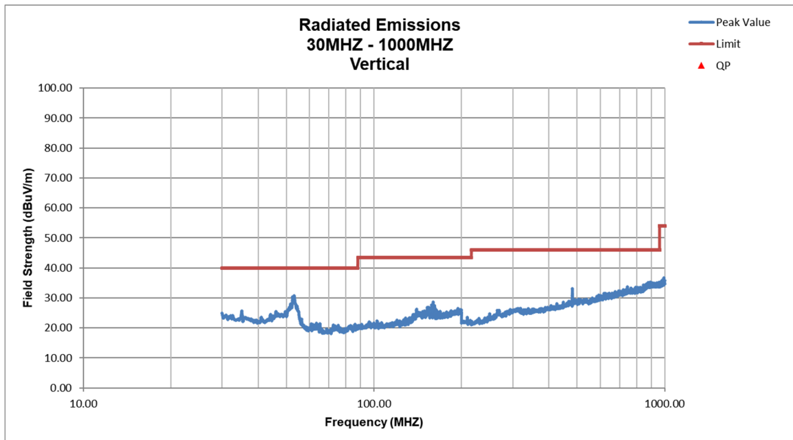
Figure 24. Radiated Emissions, Vertical 30 – 1000 MHz
