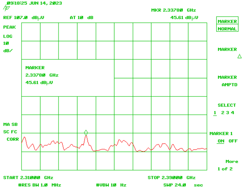
Figure 10. Low Channel Restricted Band - Average
