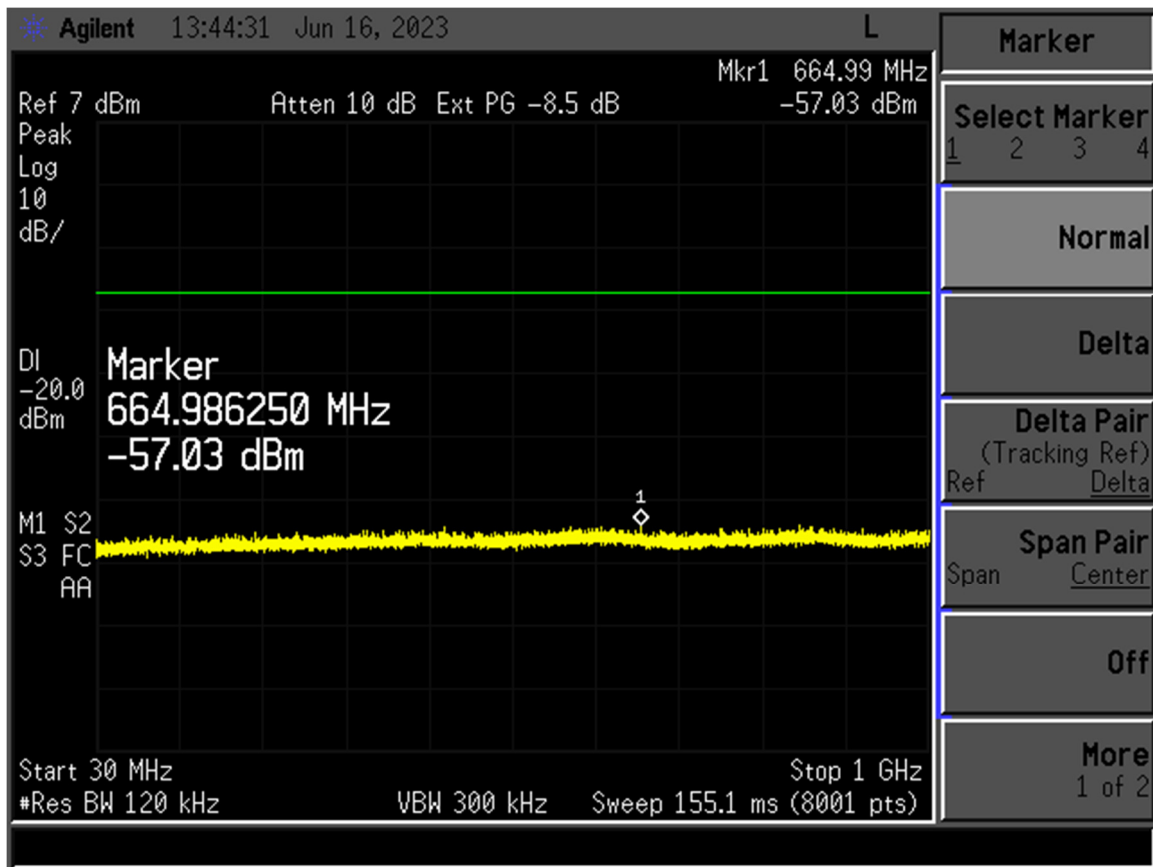
Figure 6. Channel 39, 30-1000 MHz
