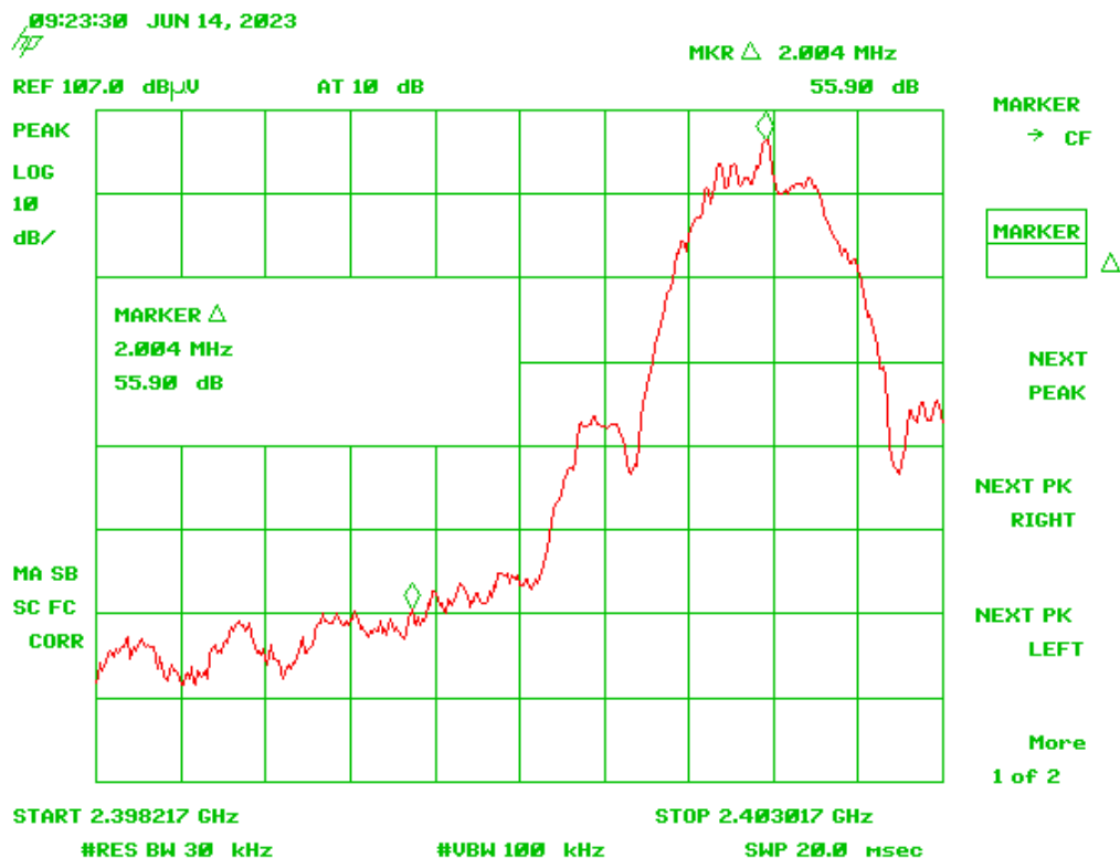
Figure 8. Band Edge Compliance – Low Channel Delta - Peak
