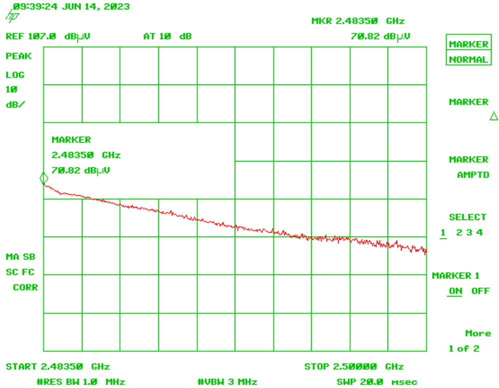
Figure 12. High Channel Restricted Band – Peak
