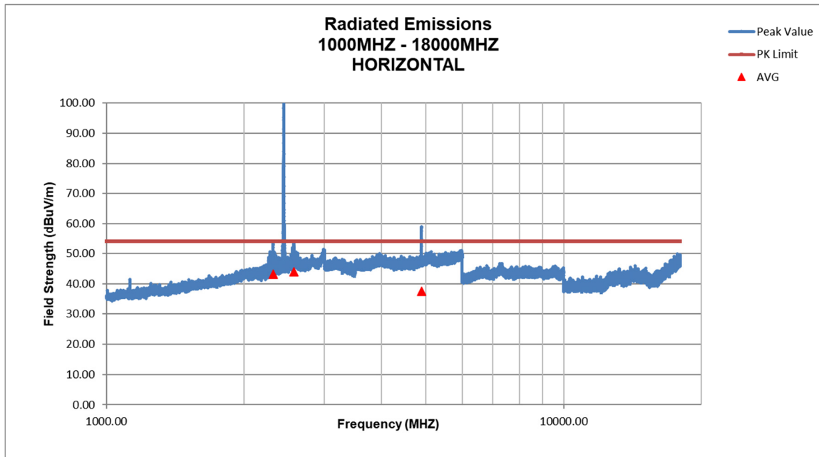
Figure 25. Radiated Emissions, Horizontal Above 1000 MHz
