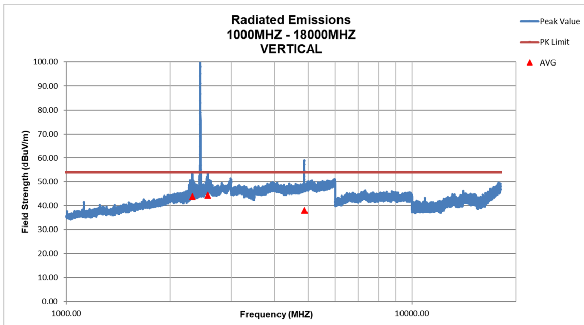
Figure 26. Radiated Emissions, Vertical Above 1000 MHz
