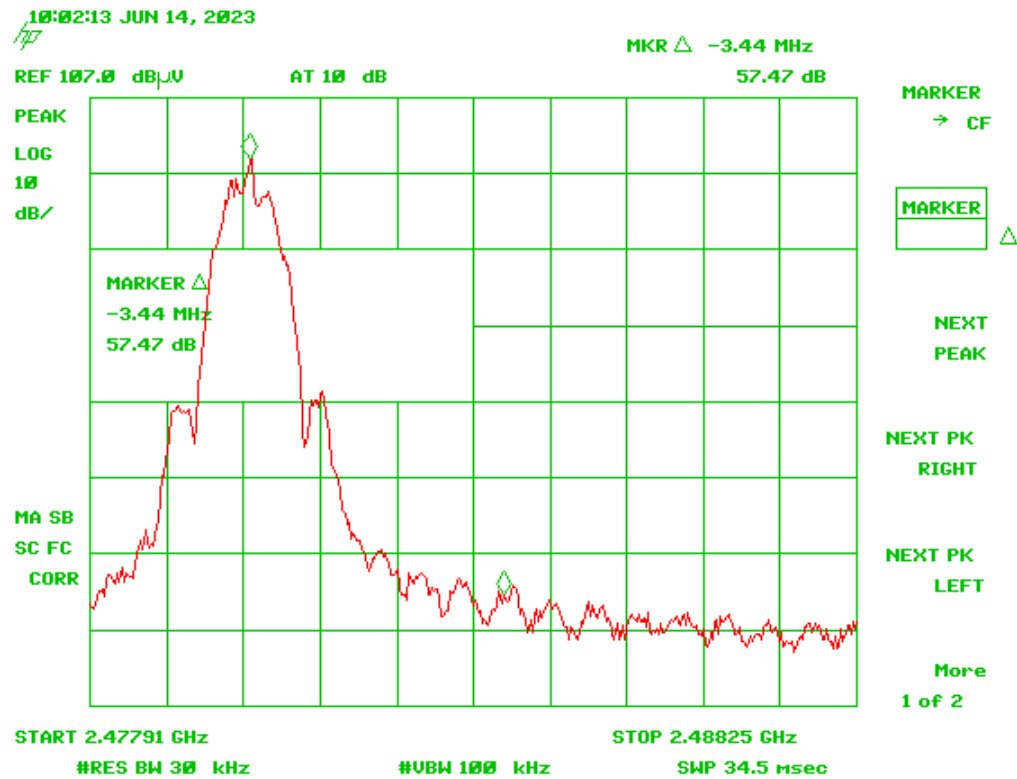
Figure 11. Band Edge Compliance – High Channel Delta - Peak
