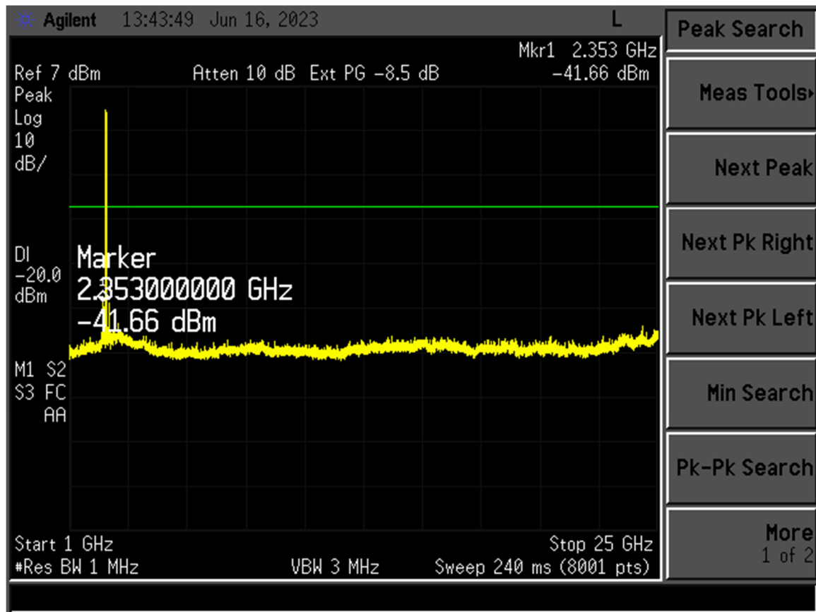
Figure 7. Channel 39, 1 - 25 GHz
