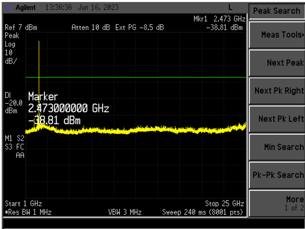
Figure 5. Channel 20, 1 – 25 GHz
