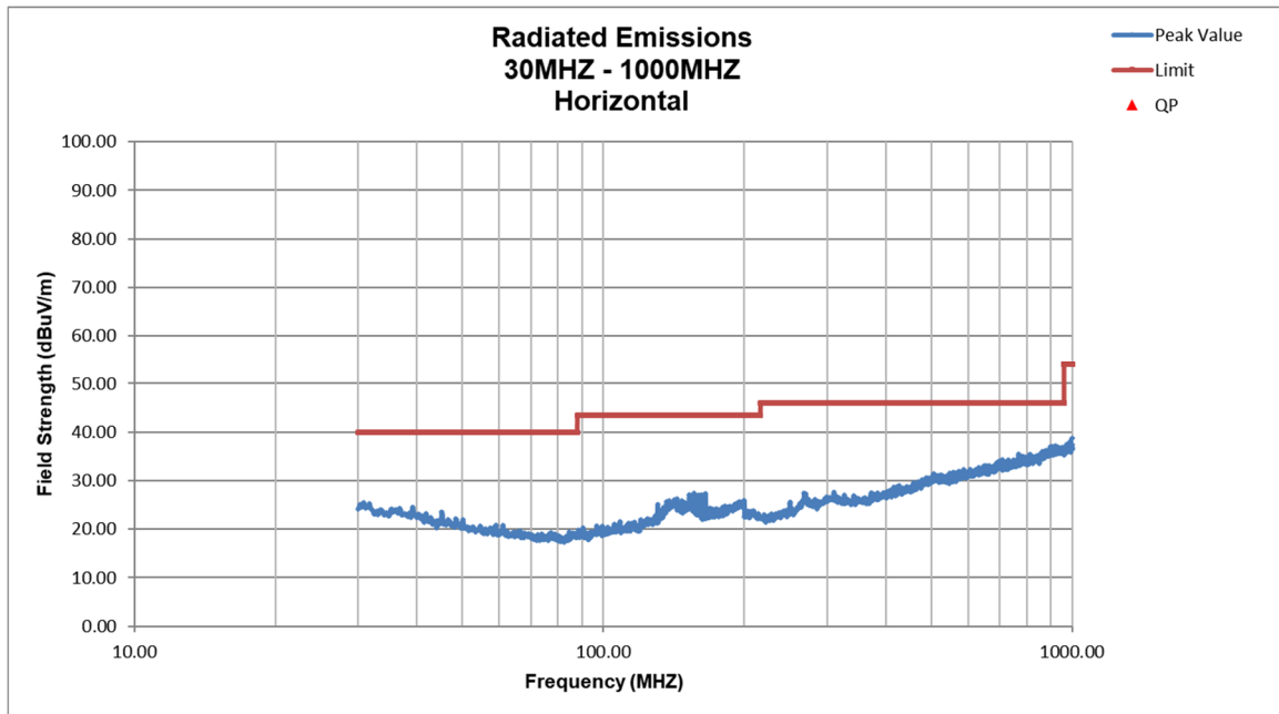
Figure 23. Radiated Emissions, Horizontal 30 – 1000 MHz
