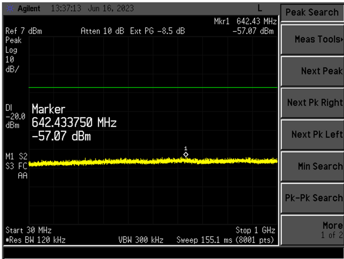
Figure 4. Channel 20, 30-1000 MHz
