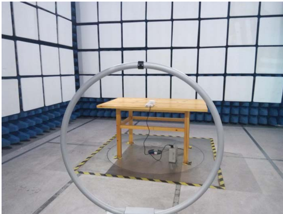
EUT with Ceramic Antenna
