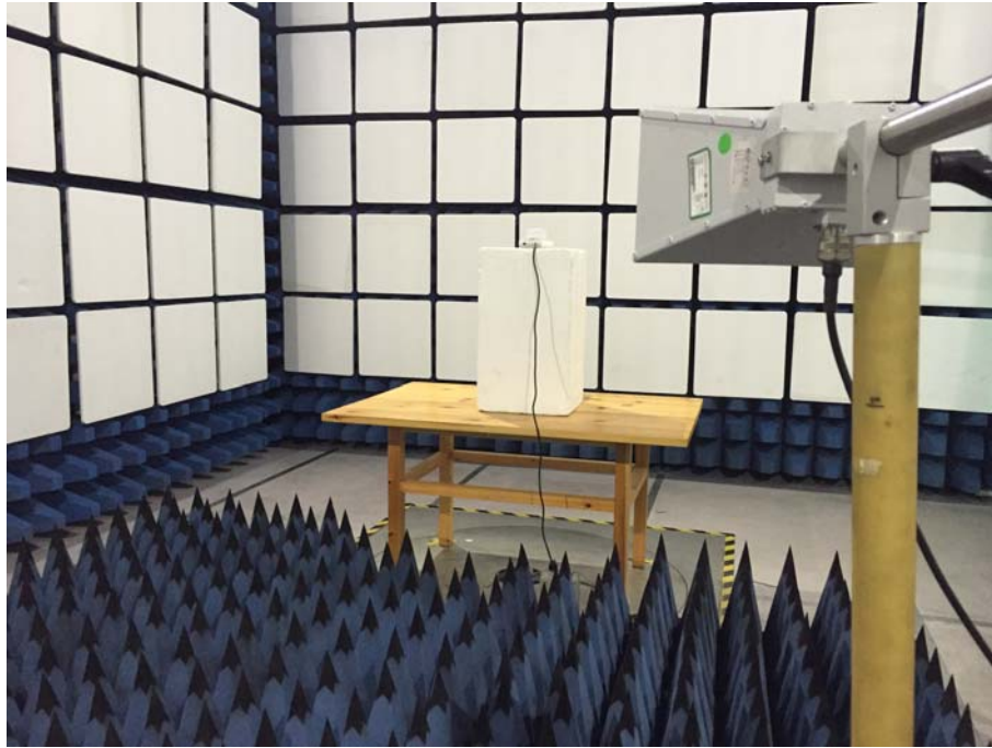
EUT with PIFA Antenna-1
