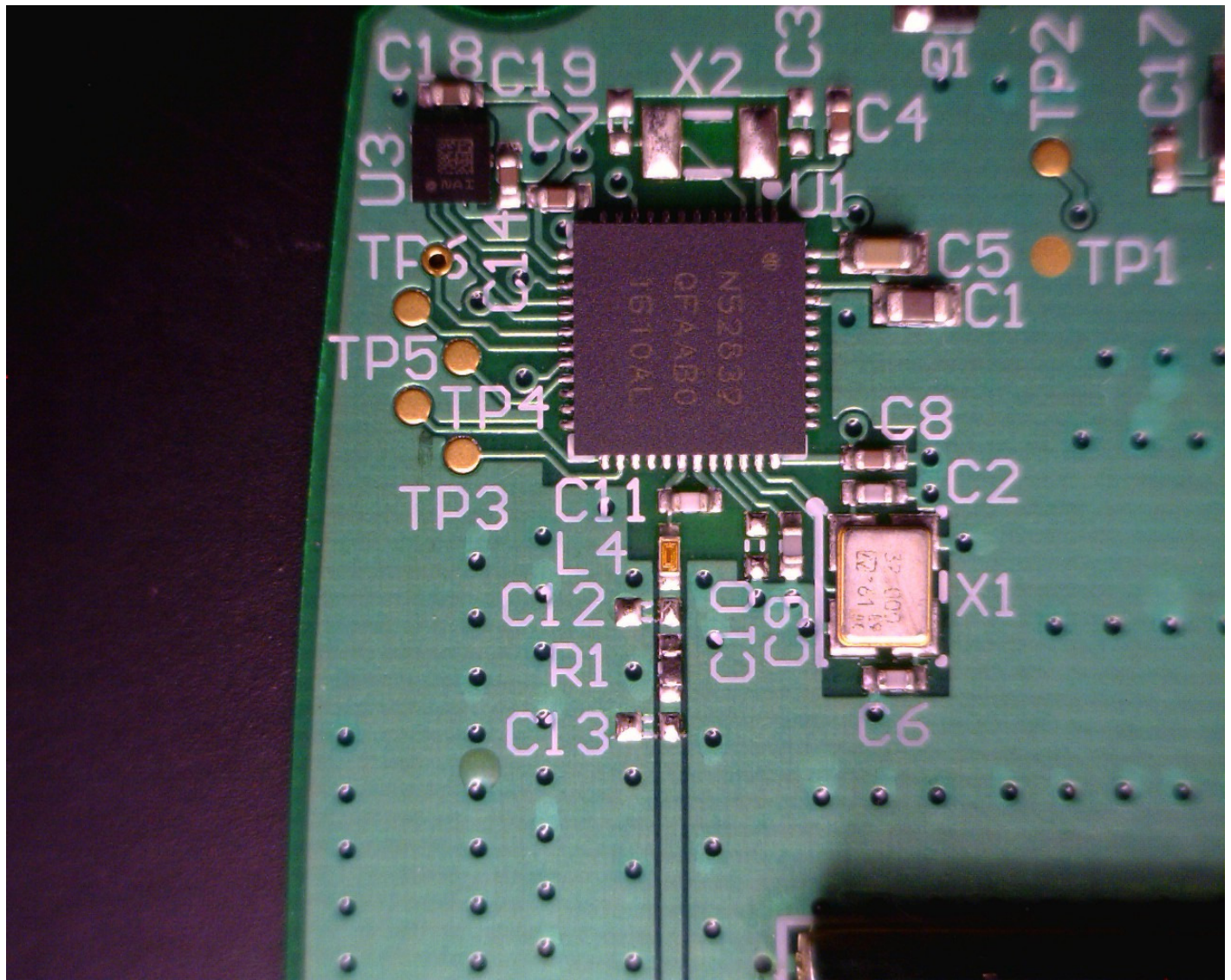
Figure 5 - SwipeSense Location Hub top view of RF Section
