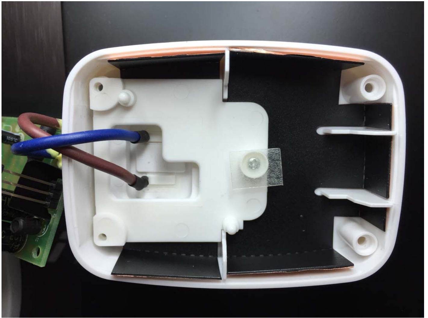
Figure 1 - SwipeSense Location Hub top view of AC wiring
