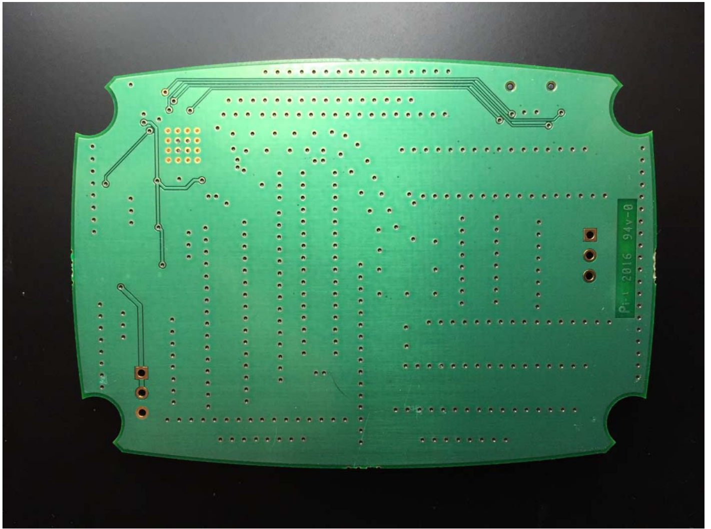
Figure 7 - SwipeSense Location Hub bottom view of digital PWB
