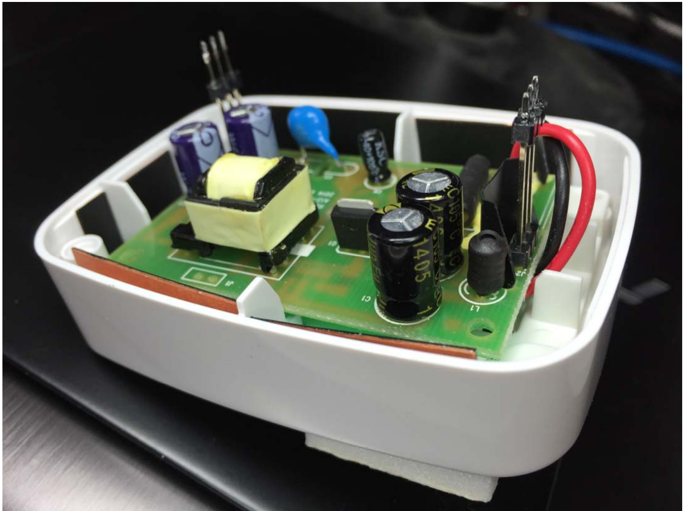
Figure 3 - SwipeSense Location Hub side view of power supply PWB
