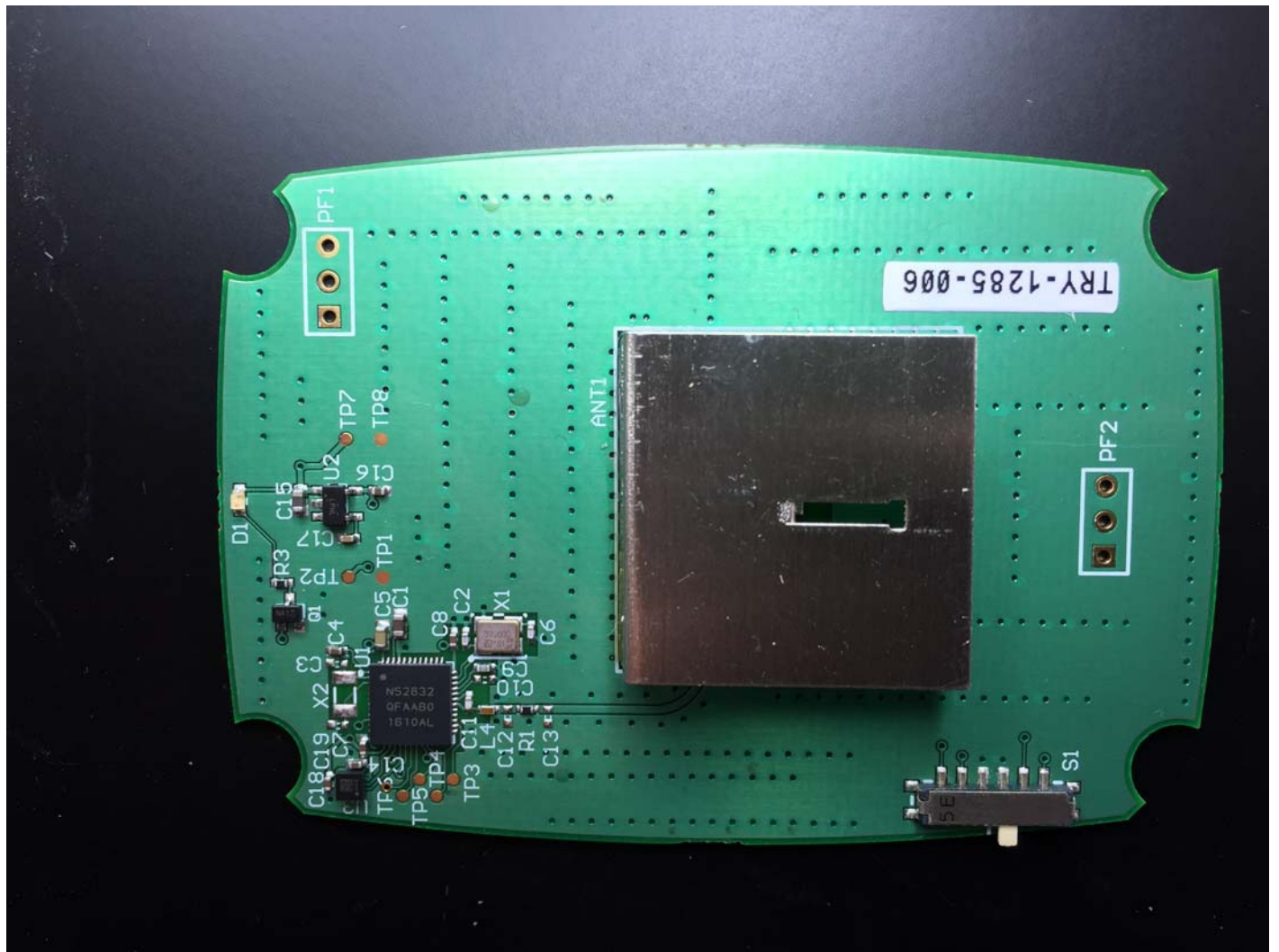
Figure 6 - SwipeSense Location Hub top view of digital PWB with antenna located in the middle of the PWB
