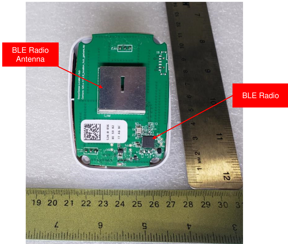
Figure 3. Front of Main PCB
