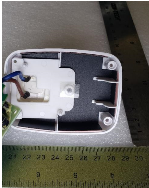
Figure 4. Enclosure with Main PCB Removed
