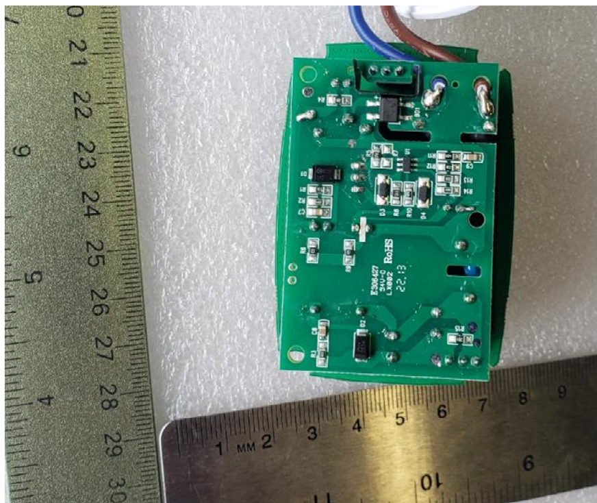
Figure 2. Back of Main PCB
