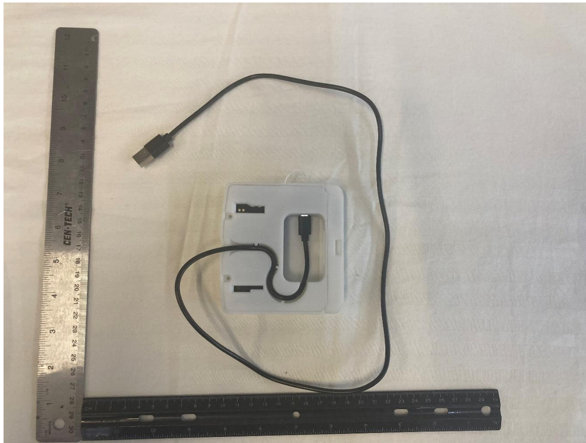
Figure 11. EUT with USB-C cable attached
