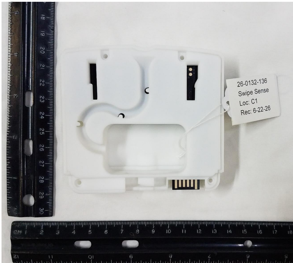
Figure 4. Back of EUT with removable cover removed
