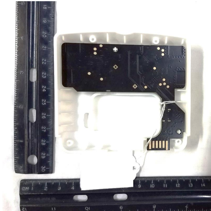
Figure 1. EUT, Front Cover Removed
