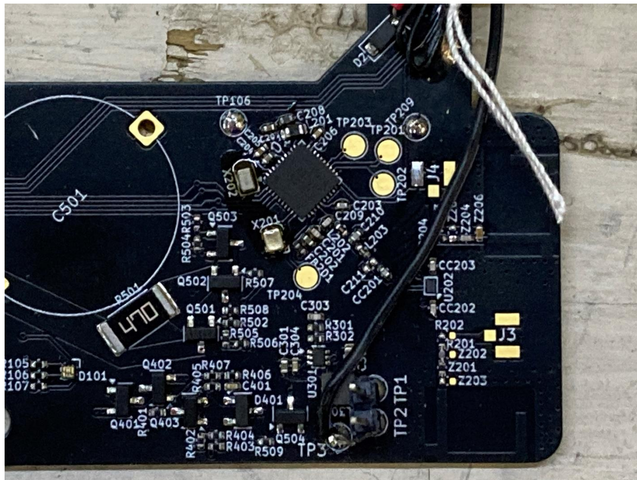
Figure 5. 2.4 GHz Thread Radio- Close up
