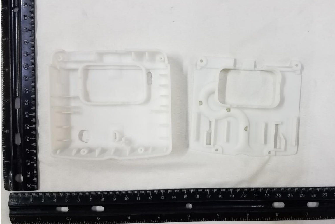
Figure 6. Enclosure with Main PCB Removed
