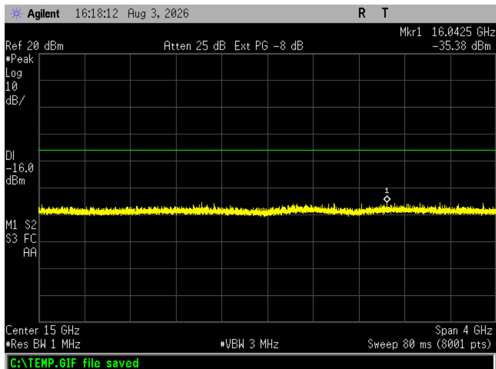
Figure 26. Antenna Conducted Emissions, Channel 39, 13 – 17 GHz
