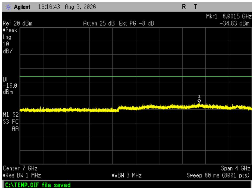
Figure 24. Antenna Conducted Emissions, Channel 39, 5 – 9 GHz
