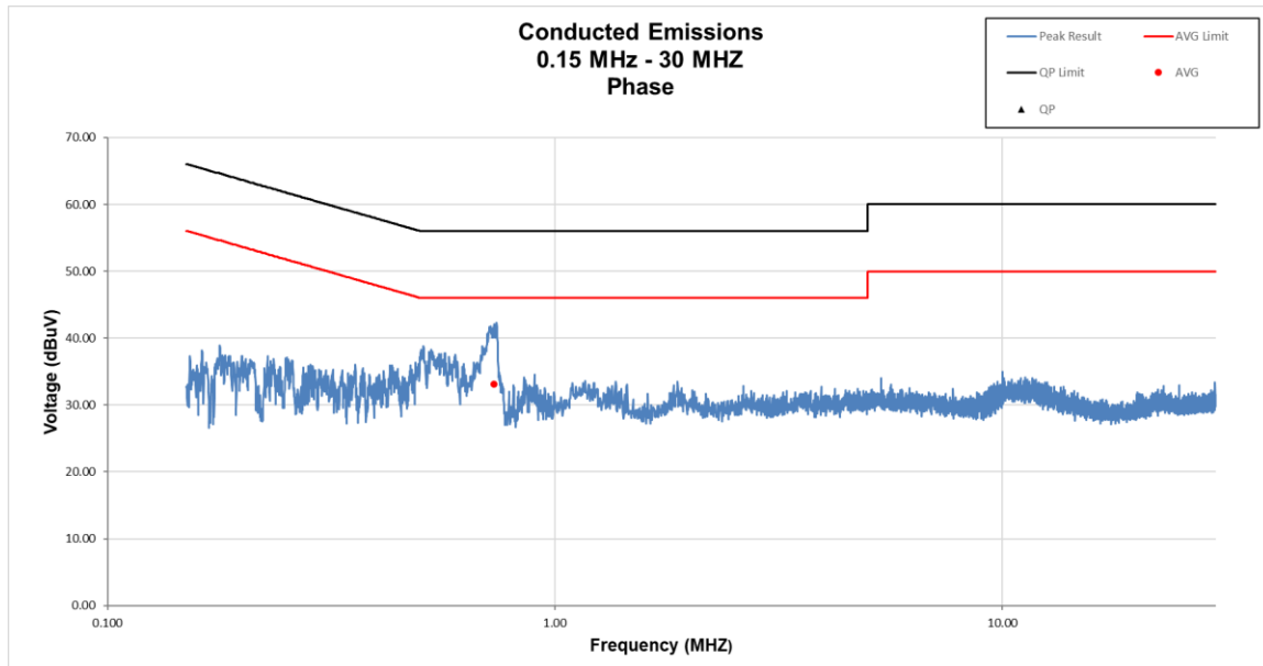
Figure 46. Conducted Emissions, Phase
