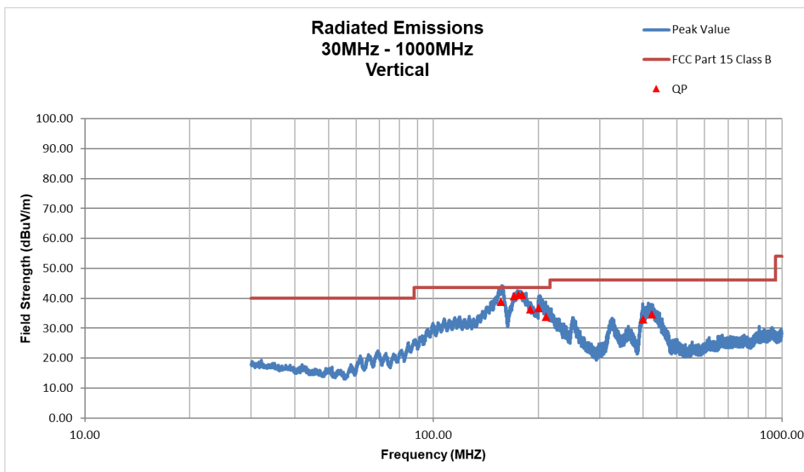
Figure 49. Radiated Spurious Emissions, 30 – 1000 MHz, Vertical
