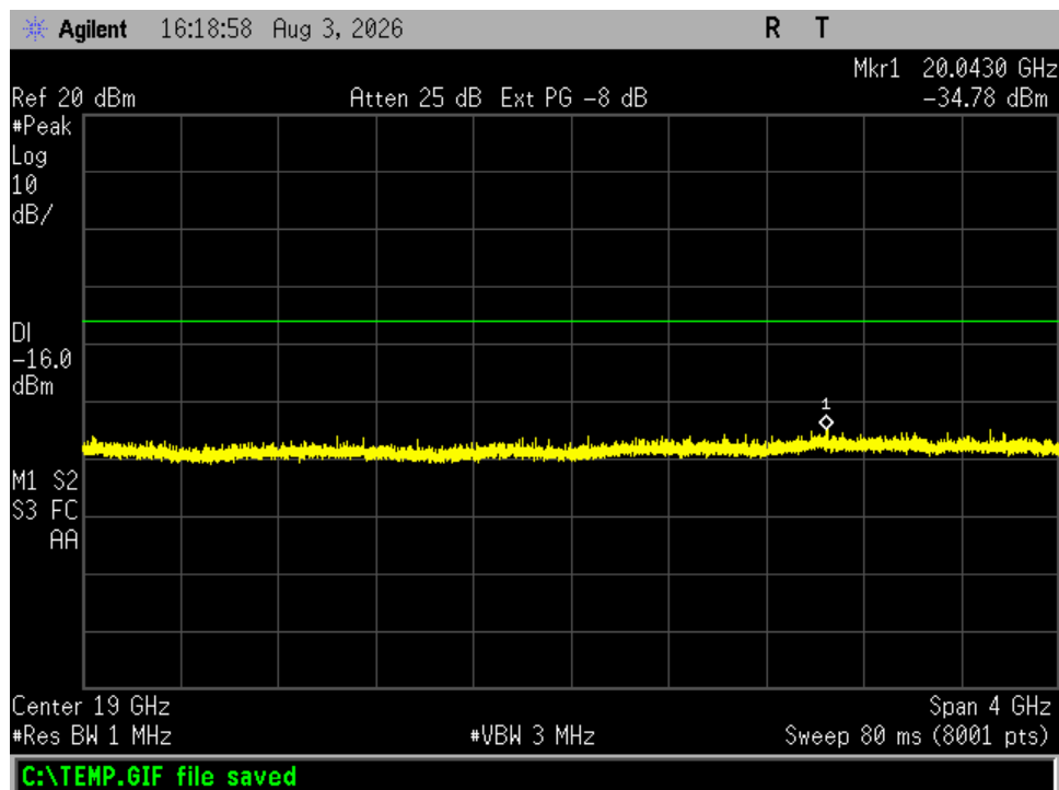
Figure 27. Antenna Conducted Emissions, Channel 39, 17 – 21 GHz
