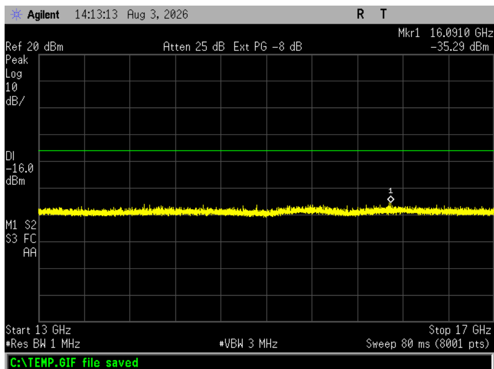
Figure 17. Antenna Conducted Emissions, Channel 24, 13 – 17 GHz
