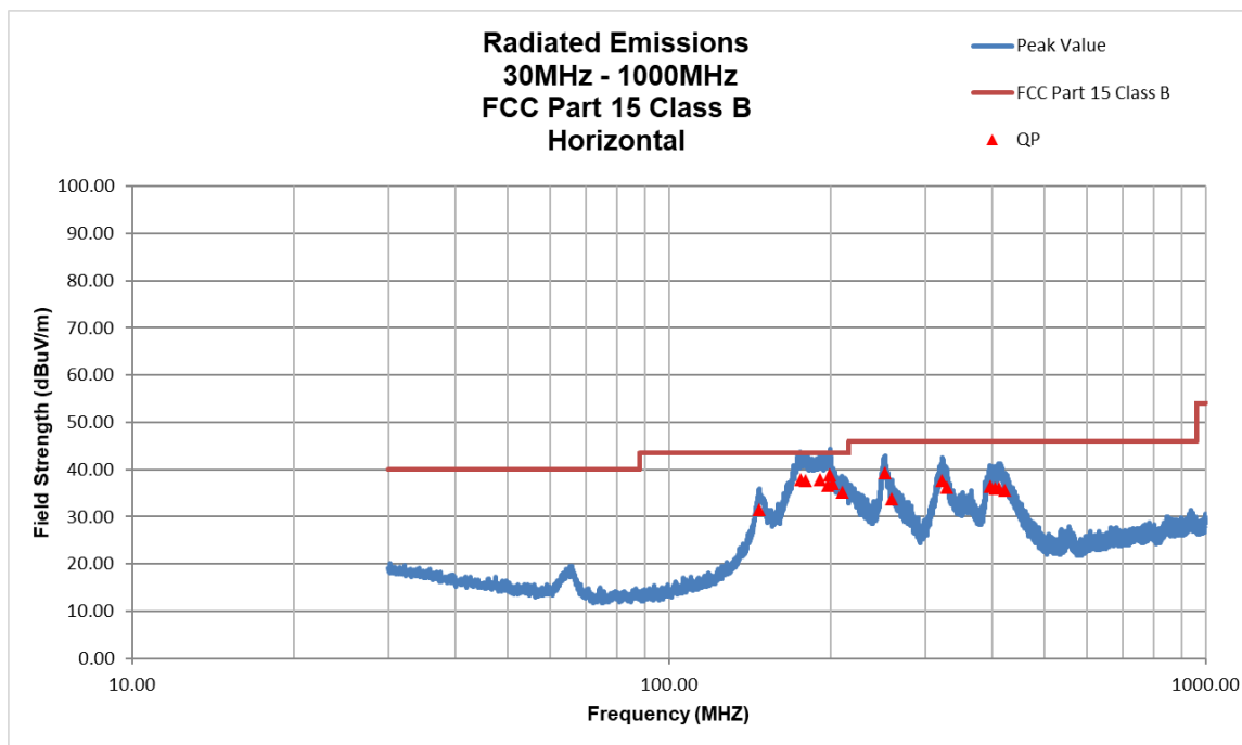
Figure 48. Radiated Spurious Emissions, 30 – 1000 MHz, Horizontal
