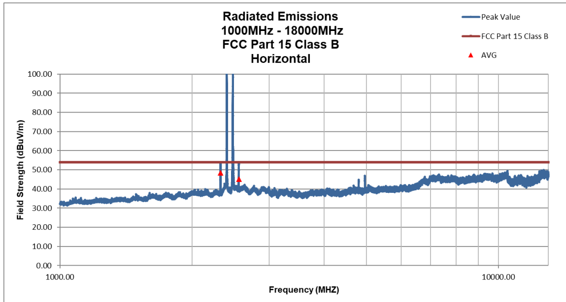
Figure 50. Radiated Spurious Emissions, 1 – 18 GHz, Horizontal
