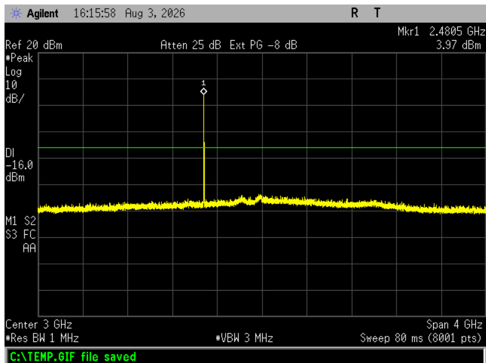
Figure 23. Antenna Conducted Emissions, Channel 39, 1 – 5 GHz
