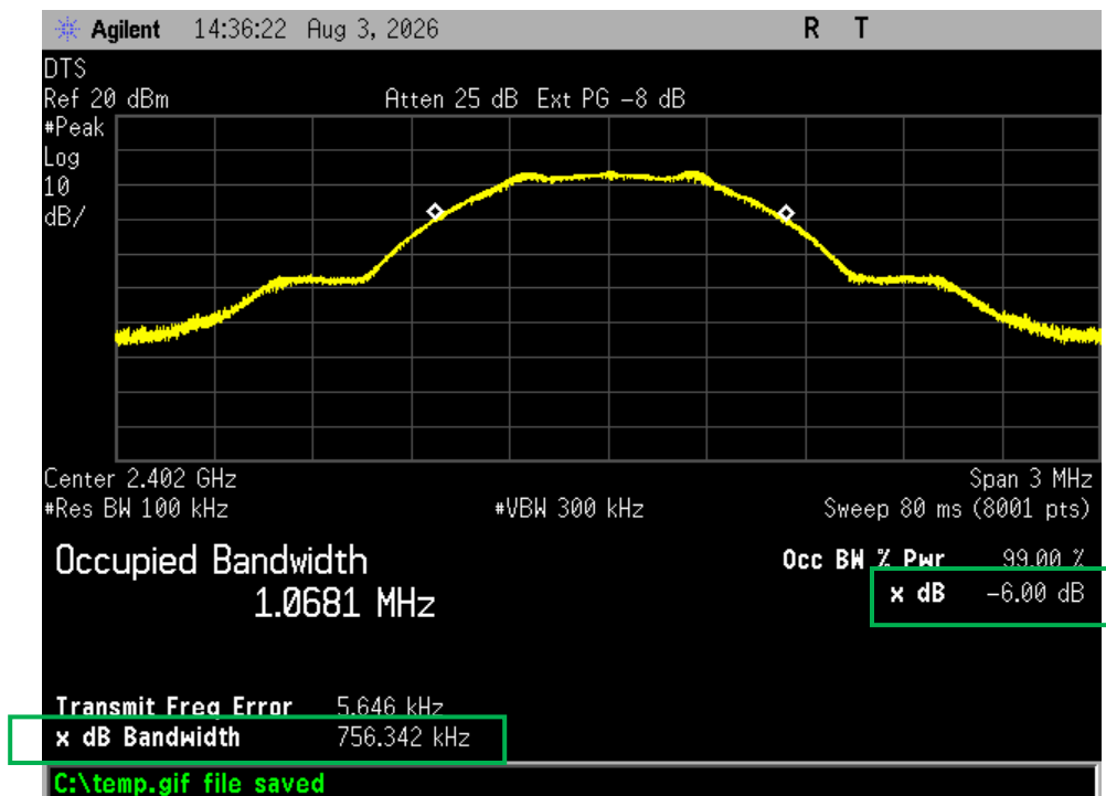
Figure 37. 6 dB Bandwidth Low Channel
