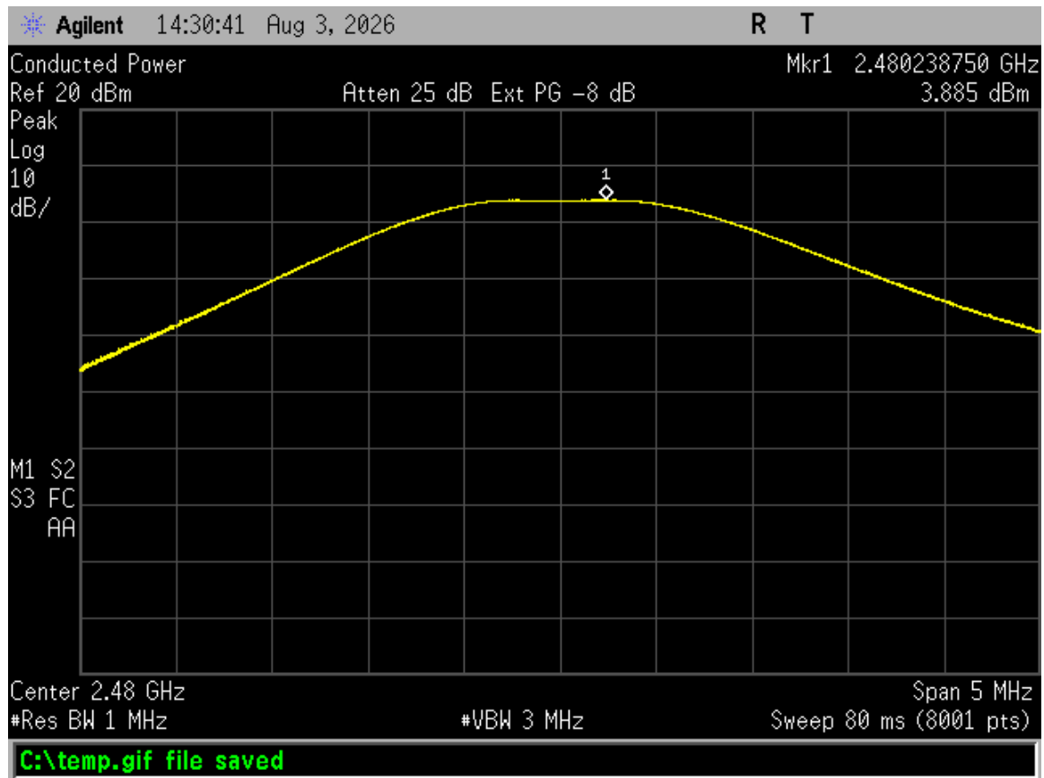
Figure 42. Peak Antenna Conducted Output Power, High Channel
