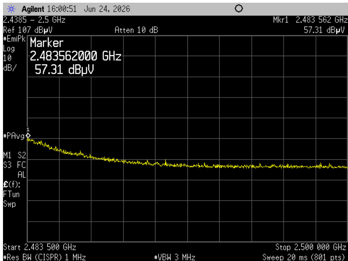
Figure 33. High Channel Restricted Band, Antenna 1 – Peak
