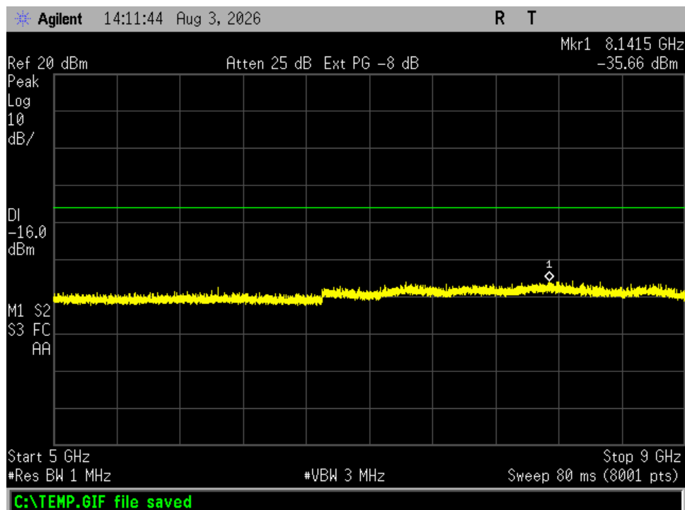
Figure 6. Antenna Conducted Emissions, Channel 0, 5 – 9 GHz
