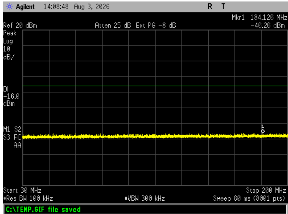
Figure 20. Antenna Conducted Emissions, Channel 39, 30-200 MHz
