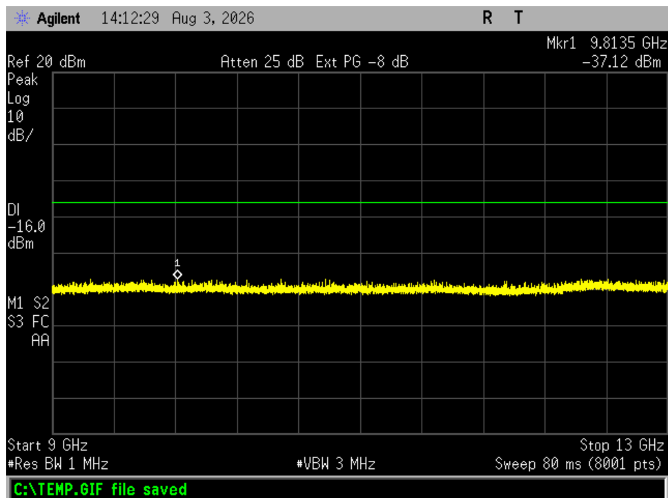
Figure 7. Antenna Conducted Emissions, Channel 0, 9 – 13 GHz
