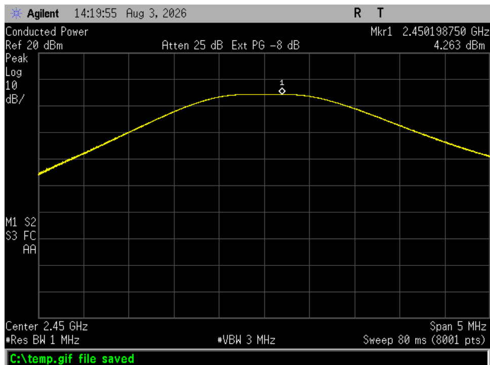
Figure 41. Peak Antenna Conducted Output Power, Mid Channel
