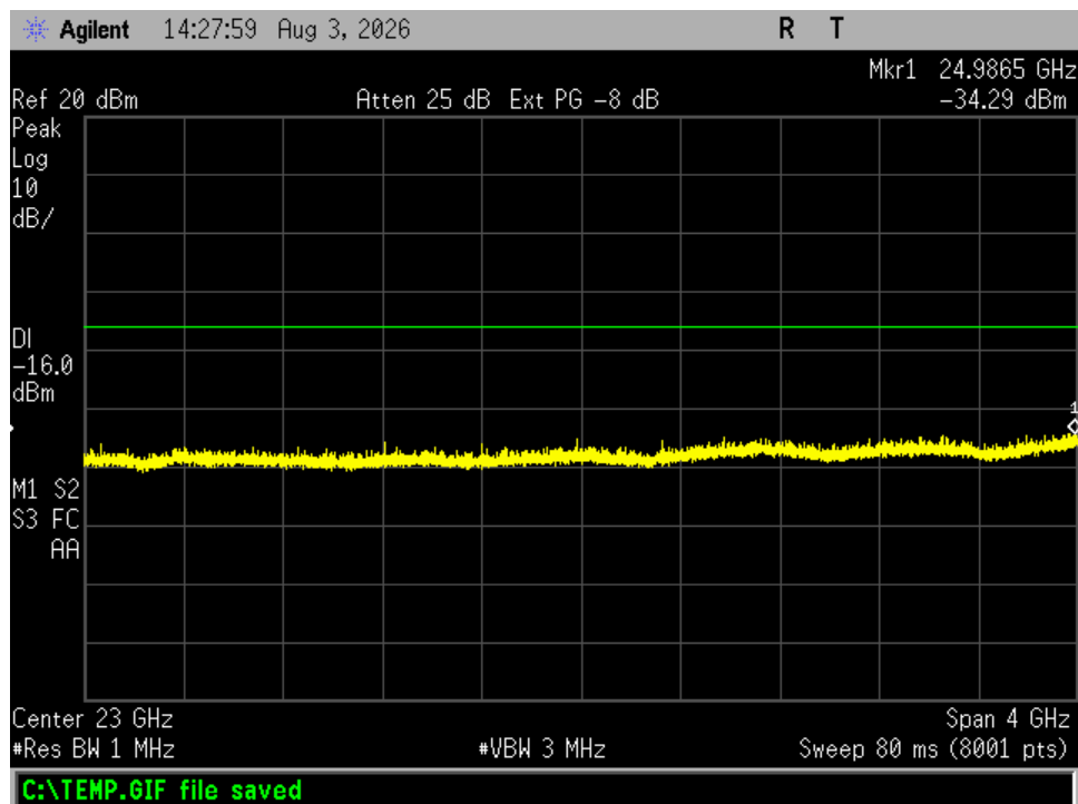
Figure 19. Antenna Conducted Emissions, Channel 24, 21 – 25 GHz
