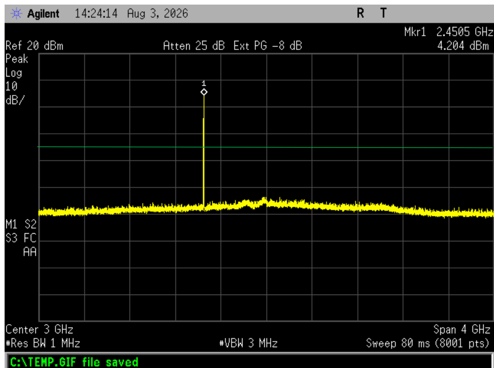
Figure 14. Antenna Conducted Emissions, Channel 24, 1 – 5 GHz
