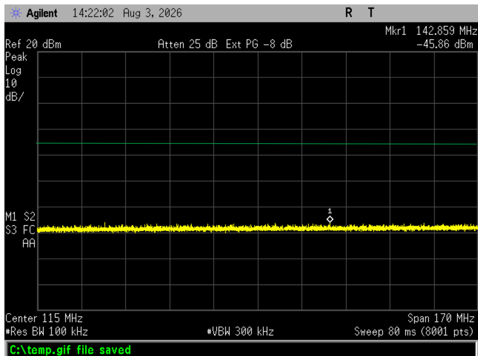
Figure 11. Antenna Conducted Emissions, Channel 24, 30-200 MHz
