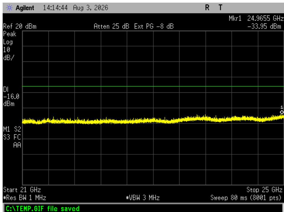
Figure 10. Antenna Conducted Emissions, Channel 0, 21 – 25 GHz
