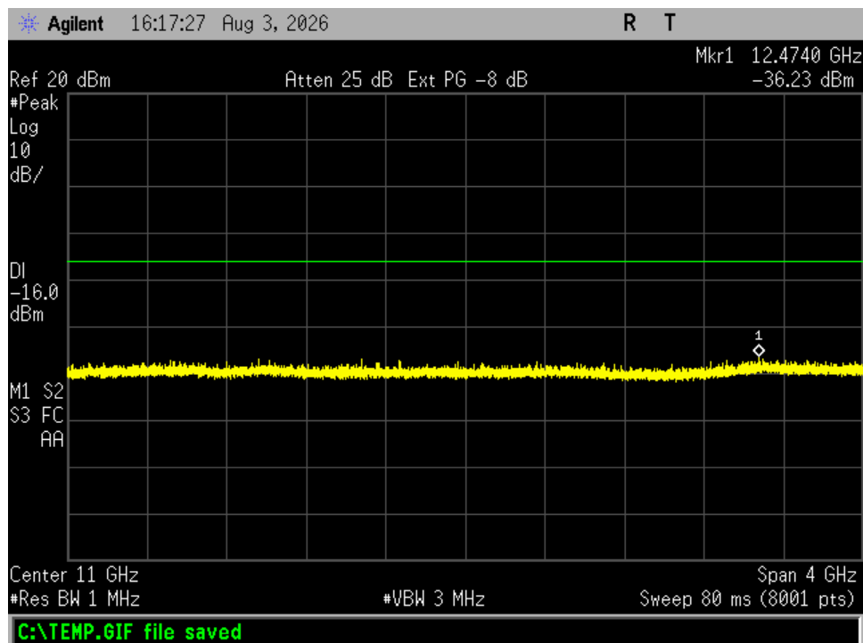
Figure 25. Antenna Conducted Emissions, Channel 39, 9 – 13 GHz
