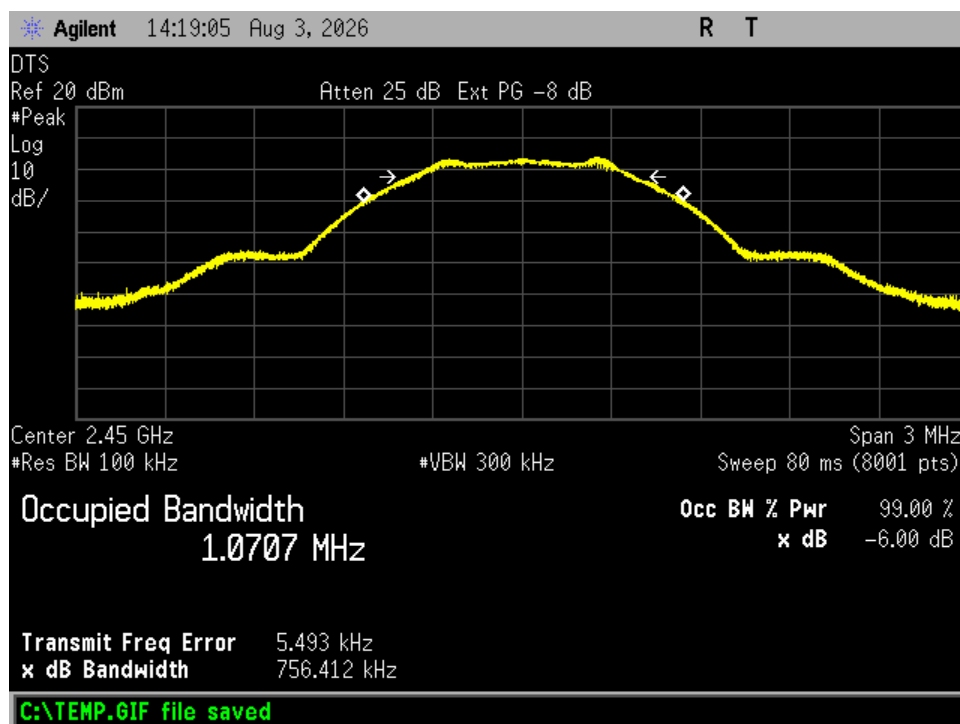
Figure 38. 6 dB Bandwidth Mid Channel
