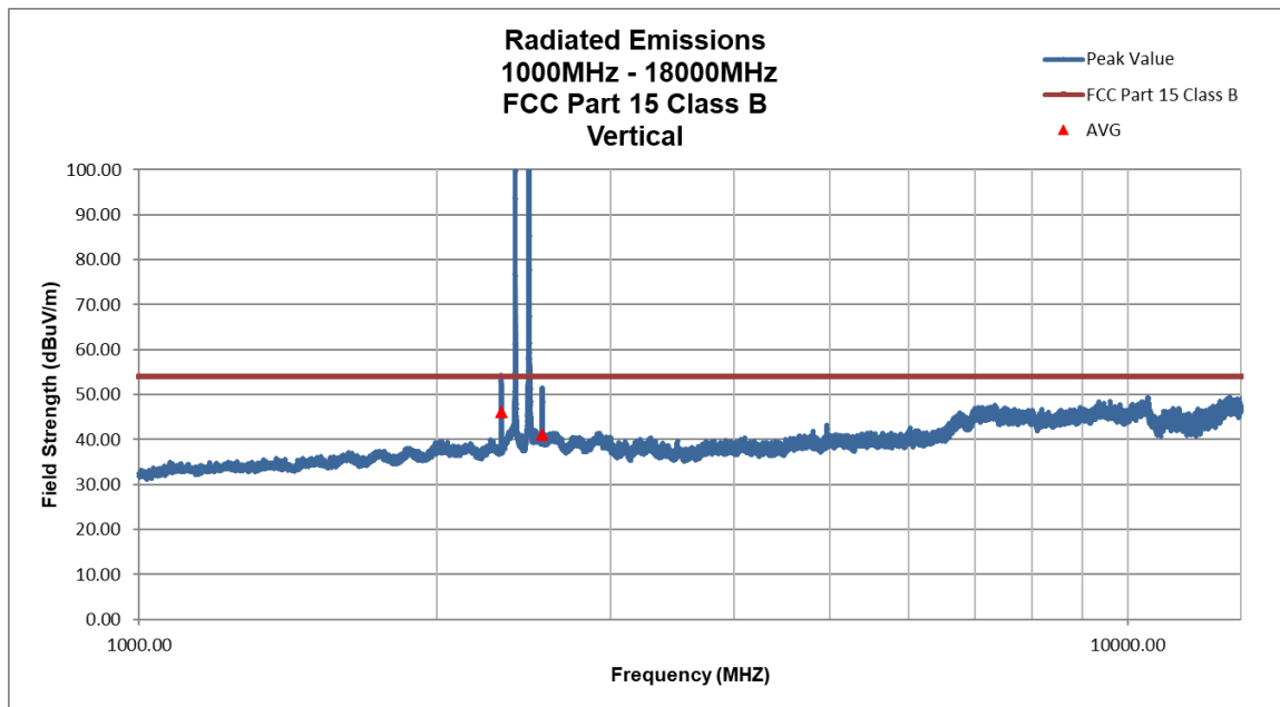
Figure 51. Radiated Spurious Emissions, 1 – 18 GHz, Vertical
