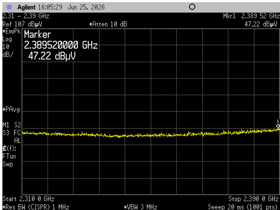
Figure 31. Low Channel Restricted Band Antenna 2 – Peak
