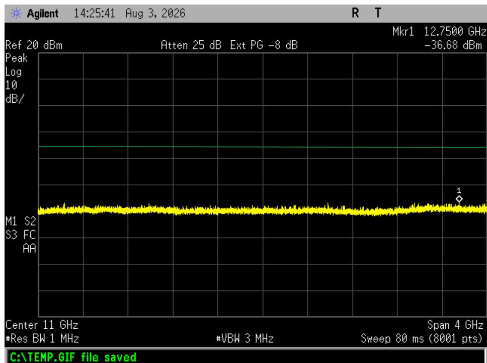
Figure 16. Antenna Conducted Emissions, Channel 24, 9 – 13 GHz
