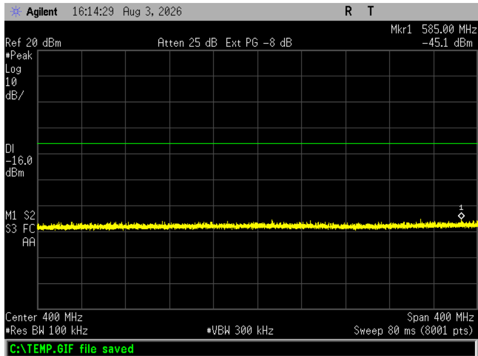
Figure 21. Antenna Conducted Emissions, Channel 39, 200-600 MHz
