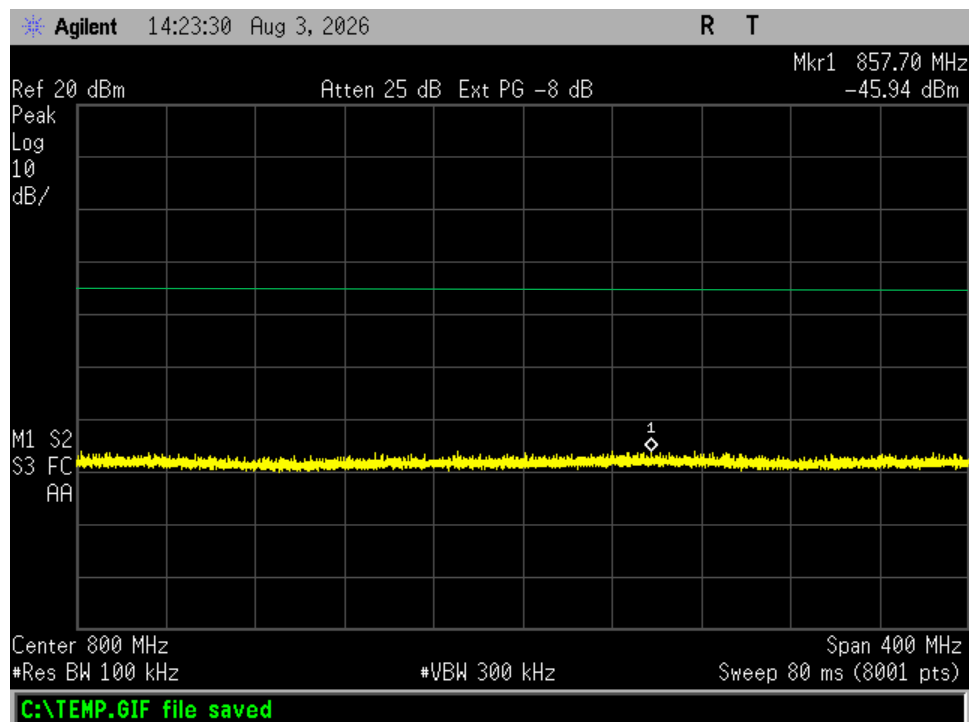
Figure 13. Antenna Conducted Emissions, Channel 24, 600-1000 MHz
