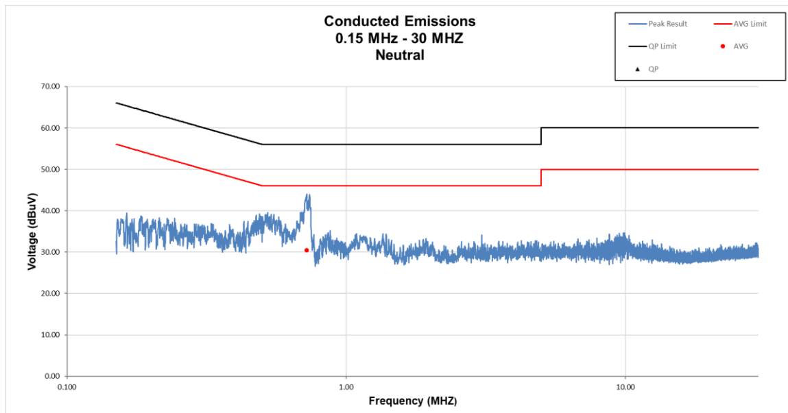
Figure 47. Conducted Emissions, Neutral
