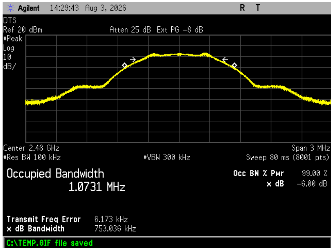
Figure 39. 6 dB Bandwidth High Channel
