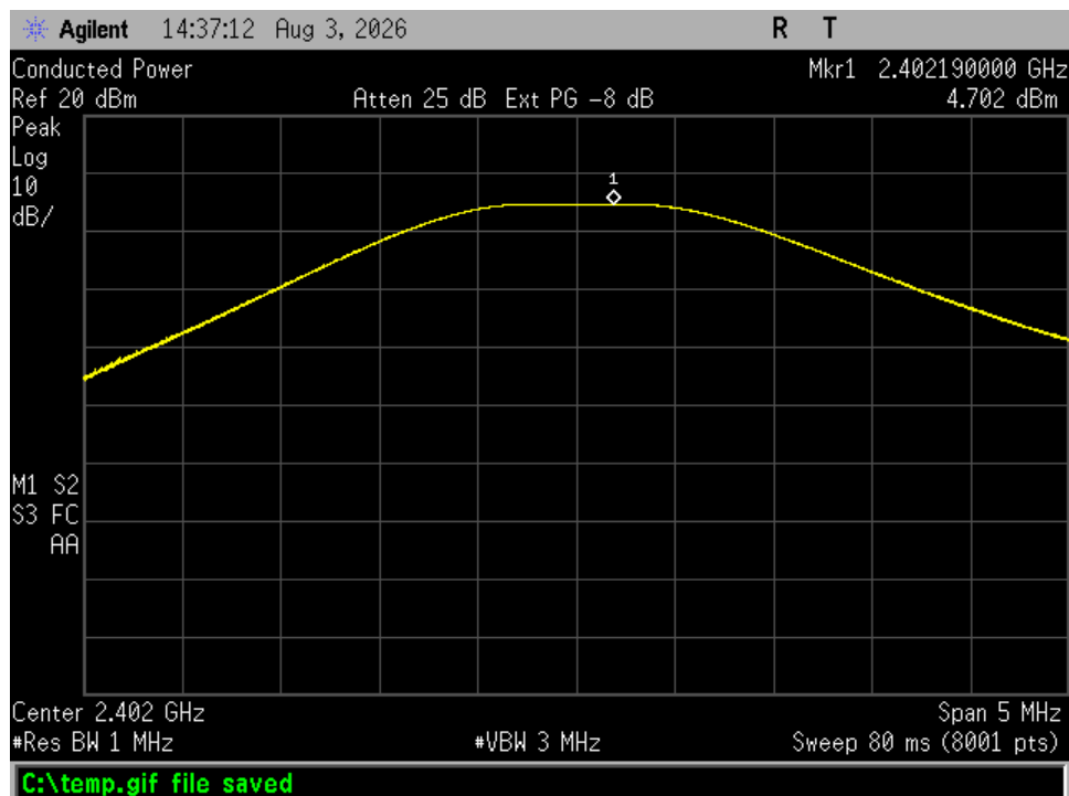
Figure 40. Peak Antenna Conducted Output Power, Low Channel
