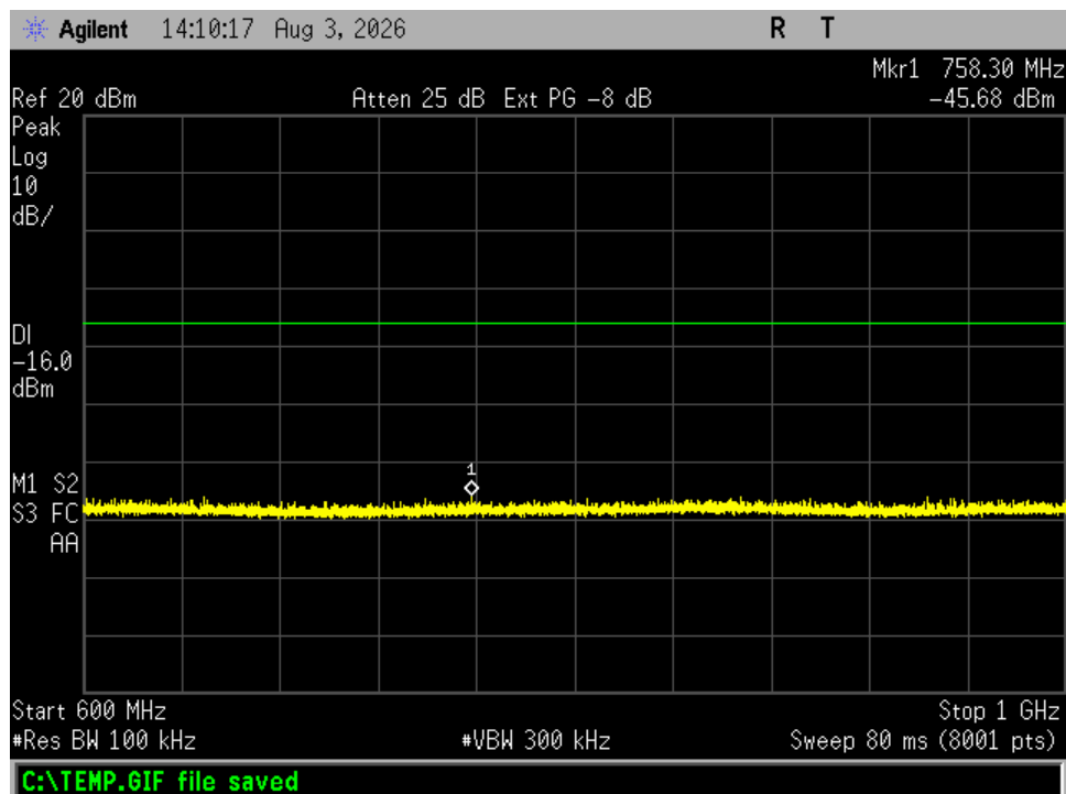
Figure 4. Antenna Conducted Emissions, Channel 0, 600-1000 MHz
