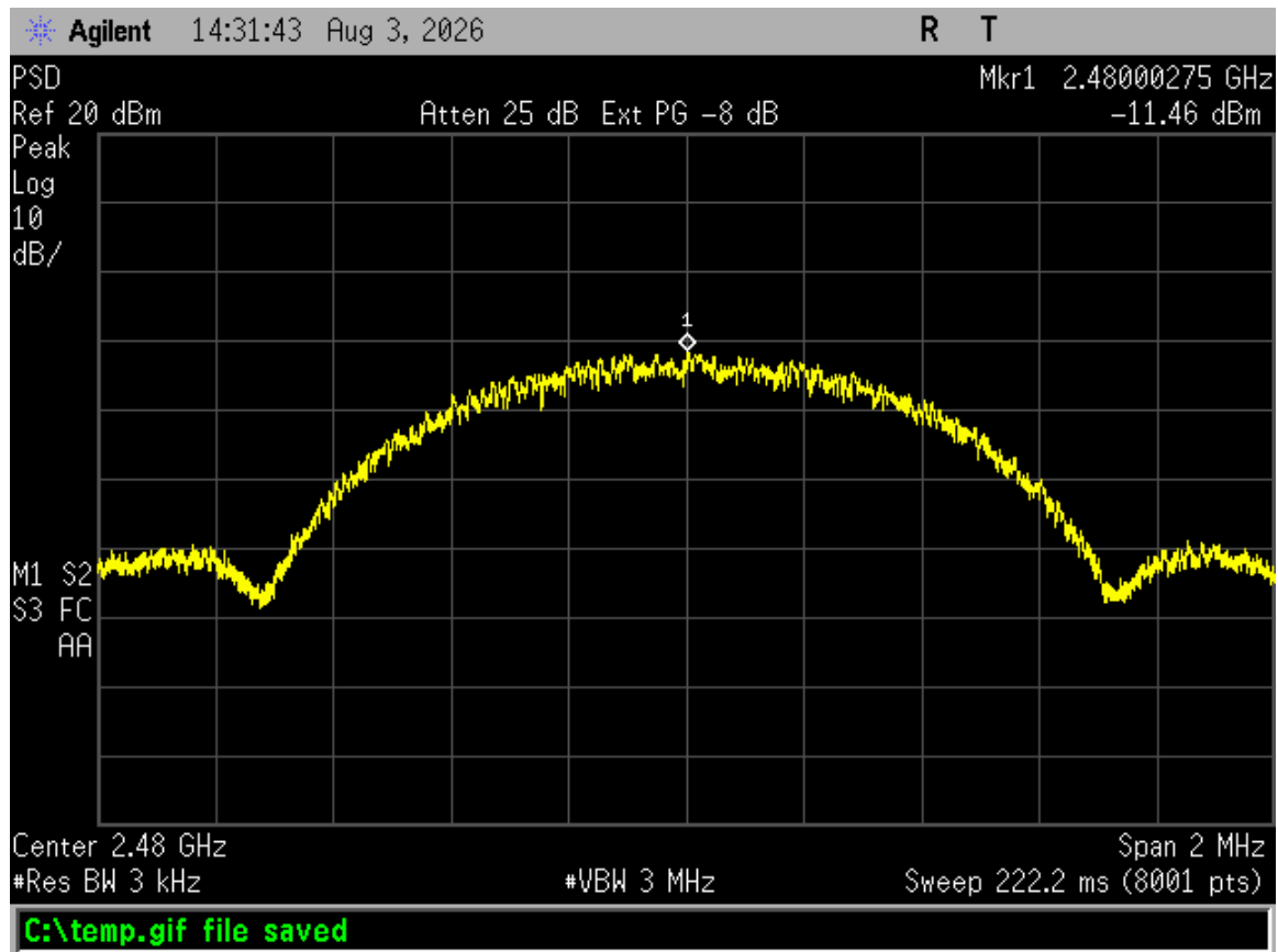
Figure 45. Power Spectral Density, High Channel
