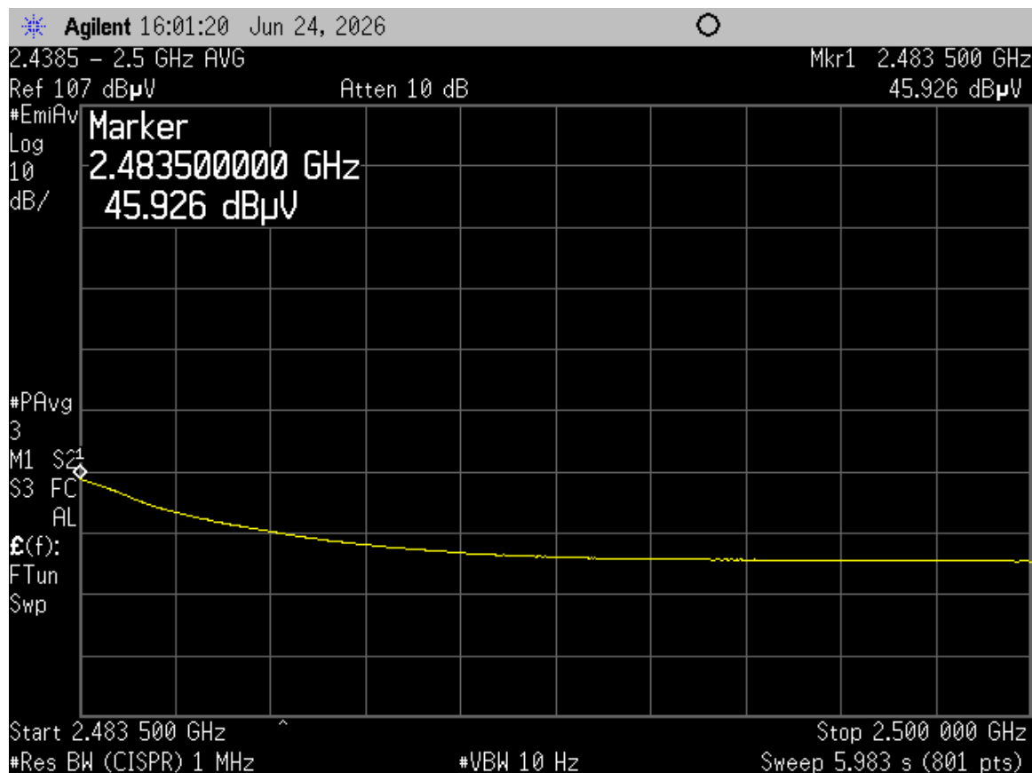
Figure 34. High Channel Restricted Band, Antenna 1 – Average
