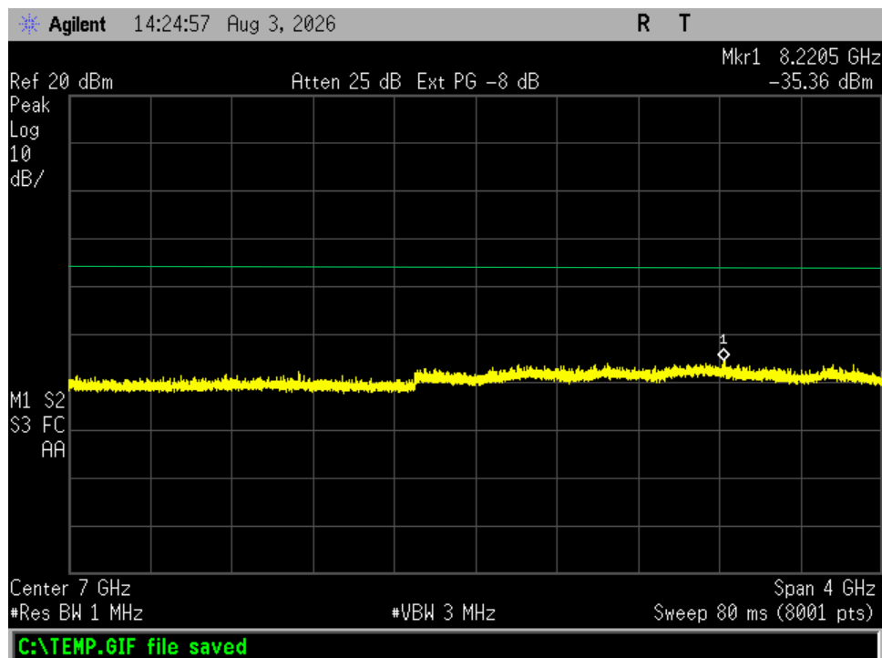
Figure 15. Antenna Conducted Emissions, Channel 24, 5 – 9 GHz
