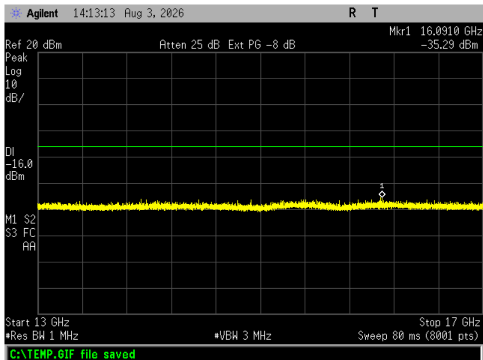
Figure 8. Antenna Conducted Emissions, Channel 0, 13 – 17 GHz
