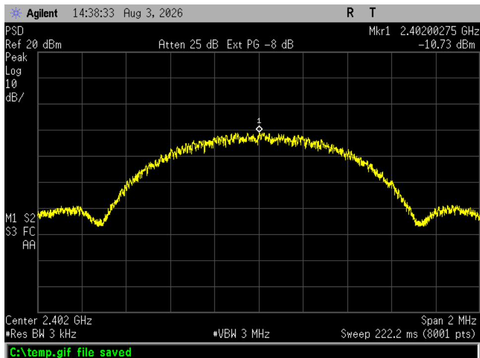
Figure 43. Power Spectral Density, Low Channel
