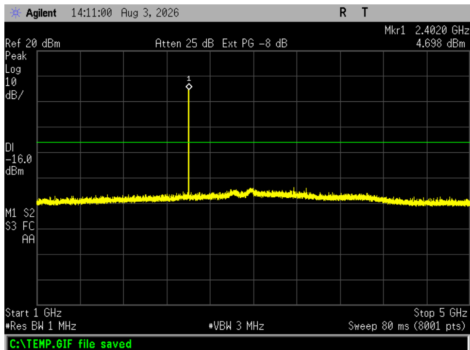
Figure 5. Antenna Conducted Emissions, Channel 0, 1 – 5 GHz
