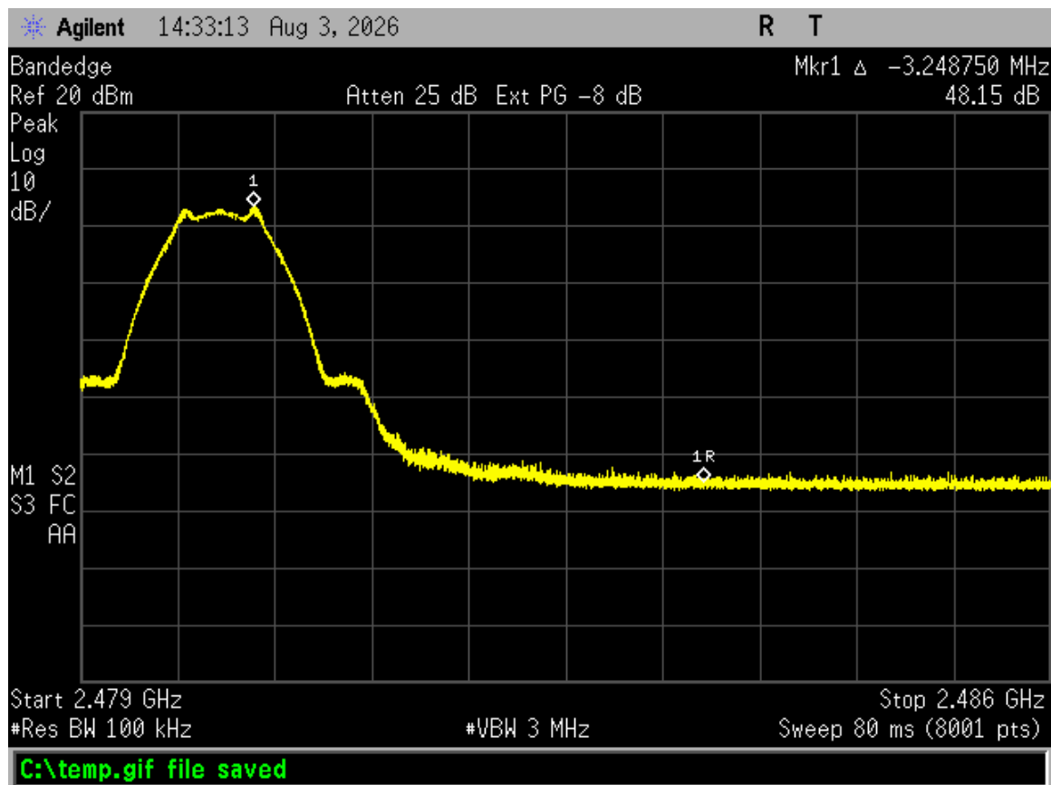
Figure 32. Band Edge Compliance – High Channel Delta - Peak
