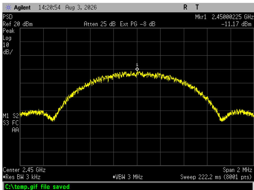
Figure 44. Power Spectral Density, Mid Channel
