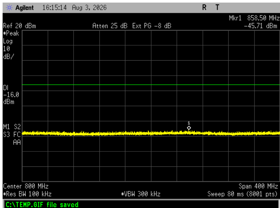
Figure 22. Antenna Conducted Emissions, Channel 39, 600-1000 MHz
