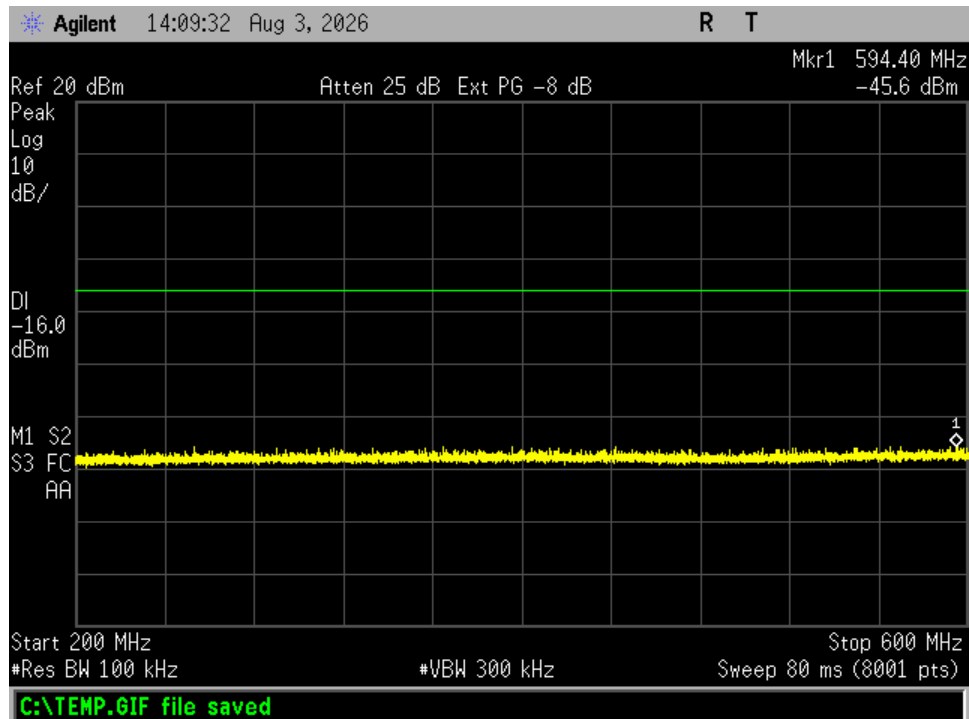
Figure 3. Antenna Conducted Emissions, Channel 0, 200-600 MHz
