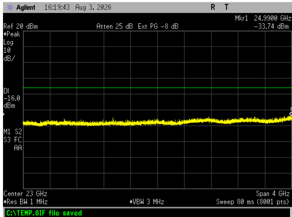
Figure 28. Antenna Conducted Emissions, Channel 39, 21 – 25 GHz
