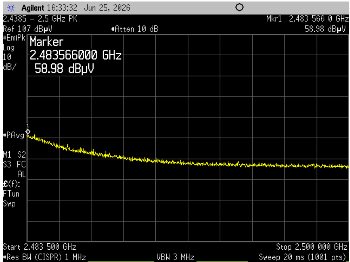
Figure 35. High Channel Restricted Band, Antenna 2 – Peak
