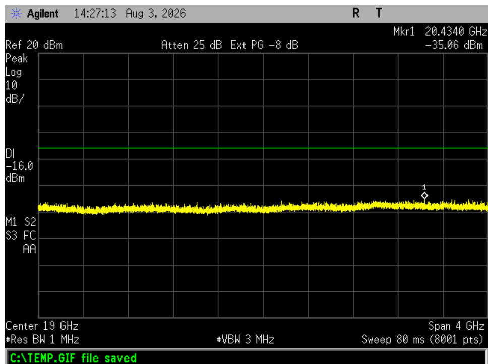
Figure 18. Antenna Conducted Emissions, Channel 24, 17 – 21 GHz
