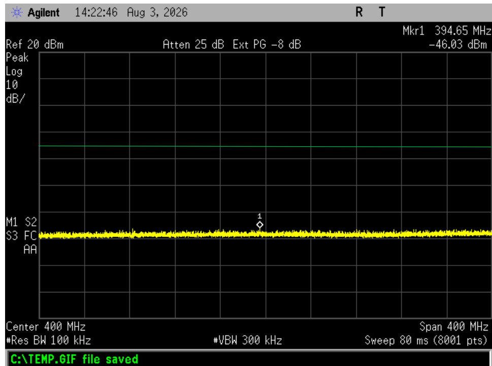
Figure 12. Antenna Conducted Emissions, Channel 24, 200-600 MHz
