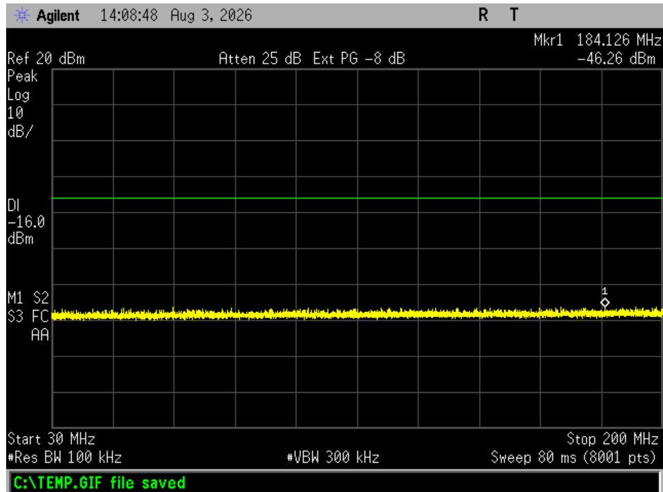
Figure 2. Antenna Conducted Emissions, Channel 0, 30-200 MHz
