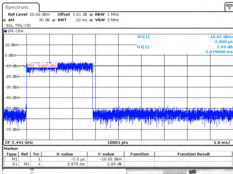
Dwell NVNT 2-DH5 2441MHz Ant1
