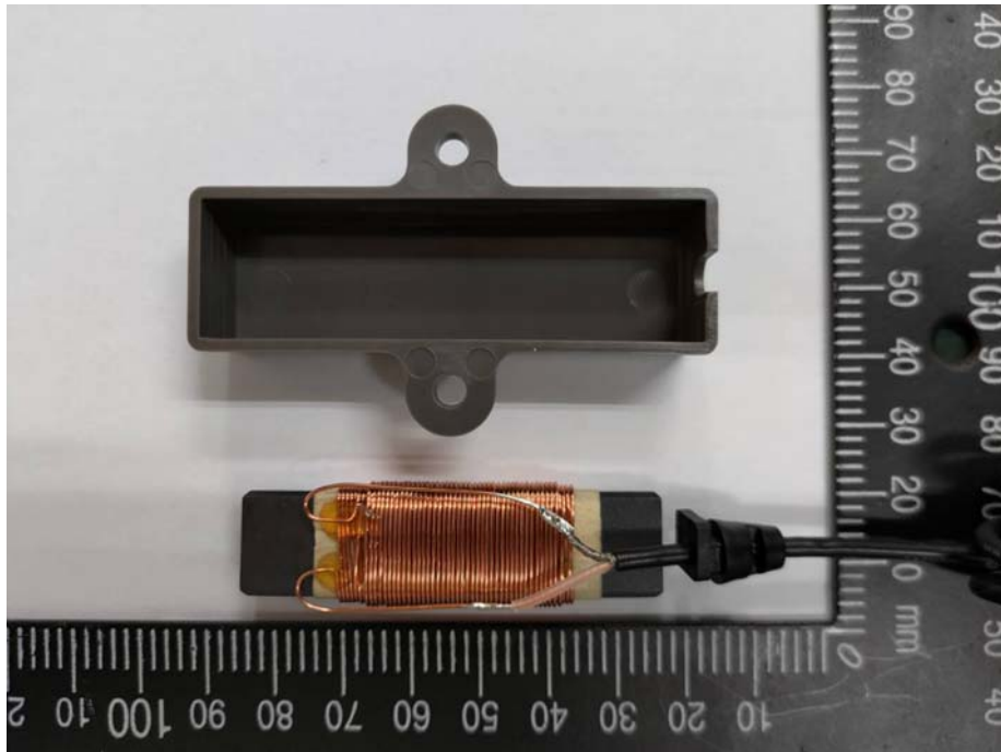
Inside view of the Rectangular housing and Coil Antenna
