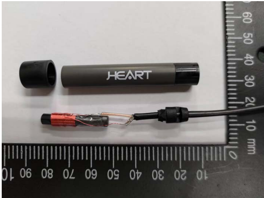
Inside view of the Stick housing and Coil Antenna
