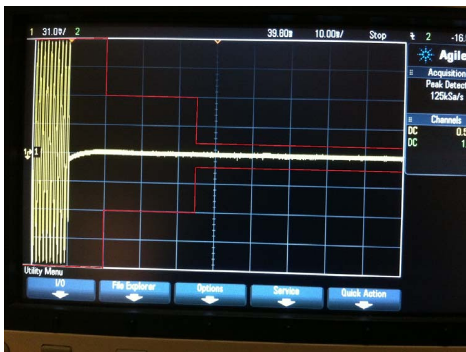
Response For Transmit Initiation – Limits Superimposed in Red
