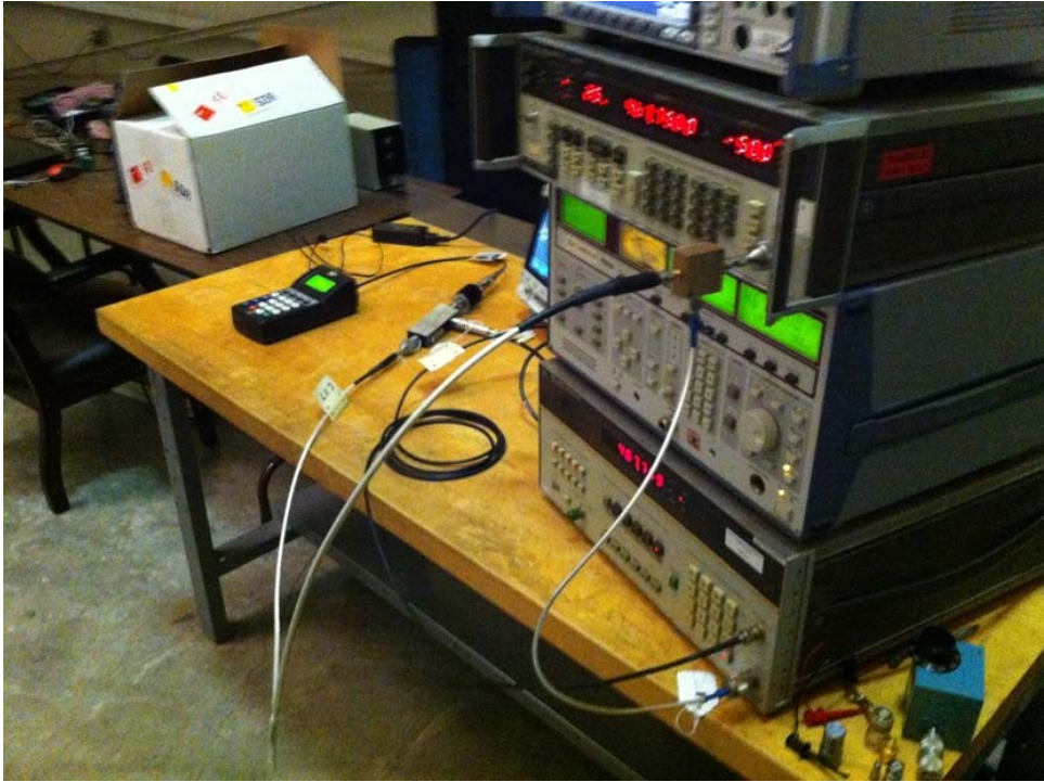
Transmit Transient
