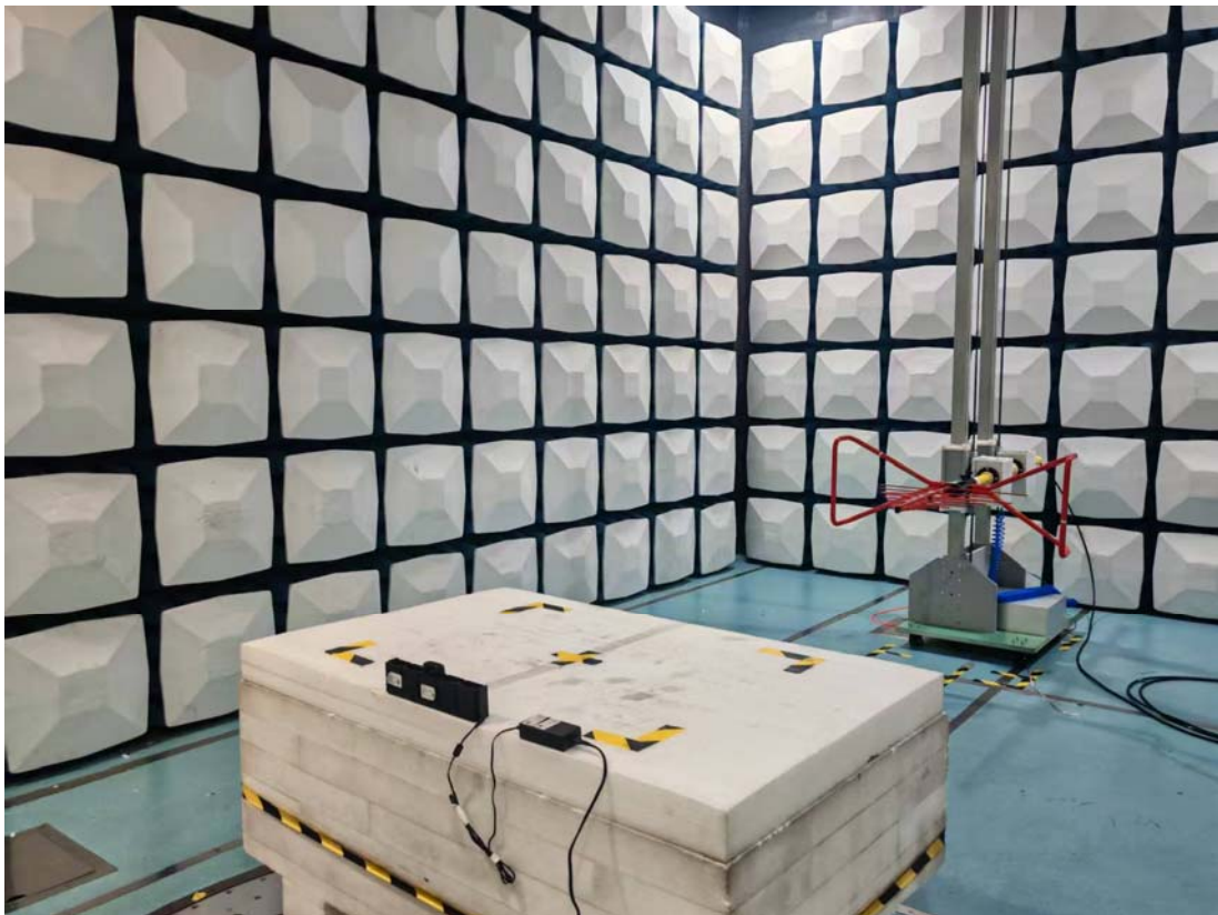
Radiated Emission 30M-1GHz Rear View M1
