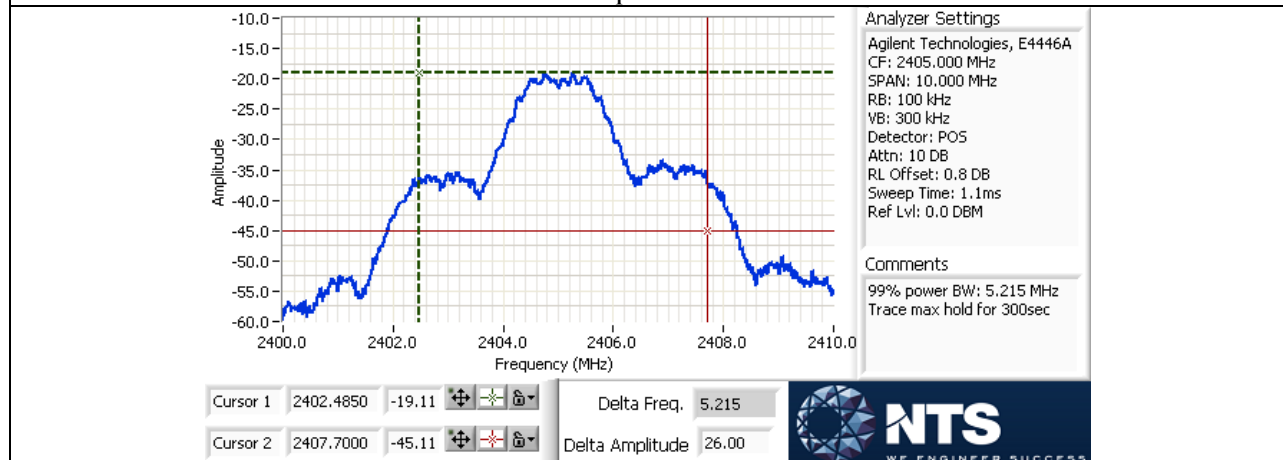
99% Occupied Bandwidth
