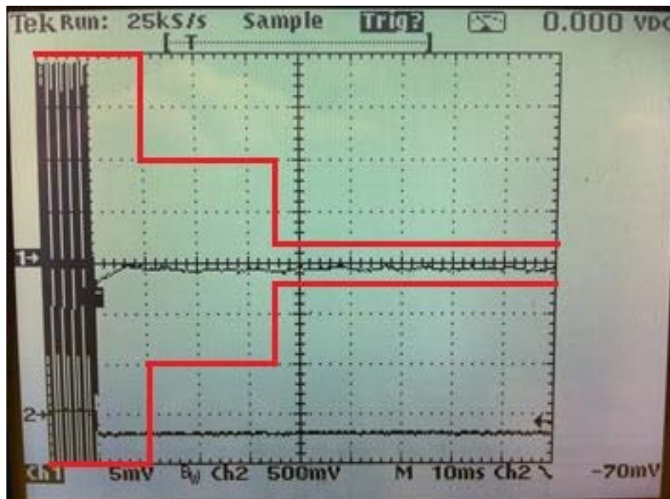
High Channel; Response For Transmit Initiation – Limits Superimposed in Red
