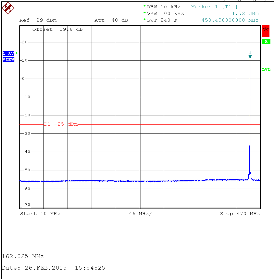
Mid Channel Spurious Conducted, Span: 10 MHz to Fundamental (Fundamental visible on right edge of plot area.) (Red line at -25 dBm, limit is 0.7 dB lower at -25.7 dBm.)
