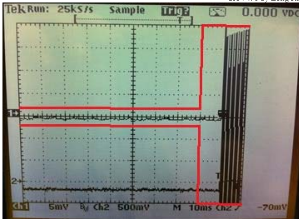
Mid Channel; Response For Transmit Cessation – Limits Superimposed in Red
