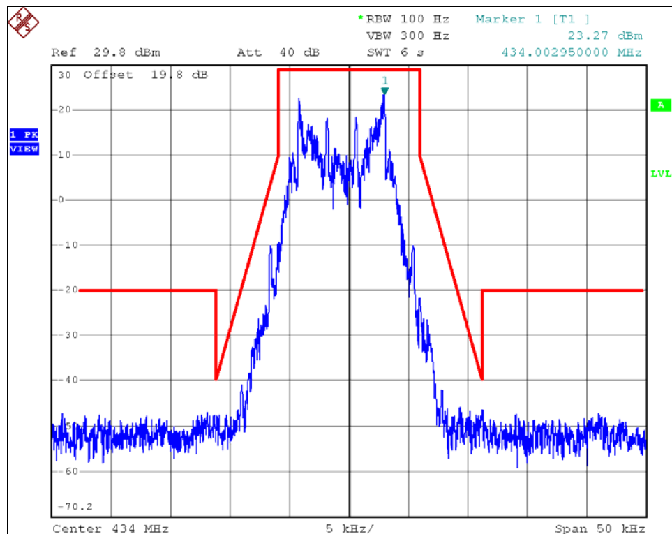
Low Channel; Modulated Emission with Superimposed Mask D
