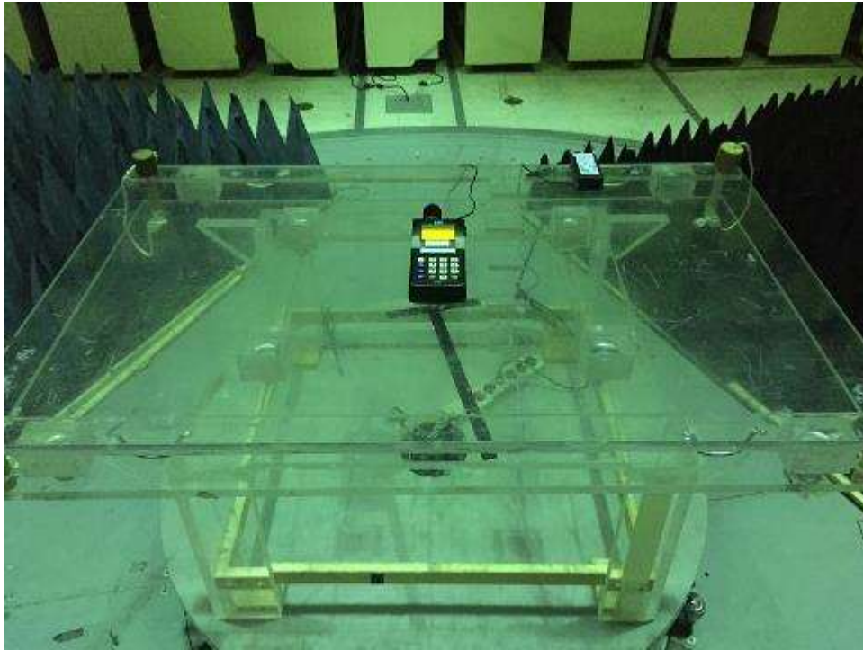
Radiated Emission, up to 1 GHz, Front
