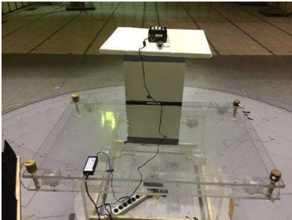
Radiated Emission, up to 5 GHz, Back
