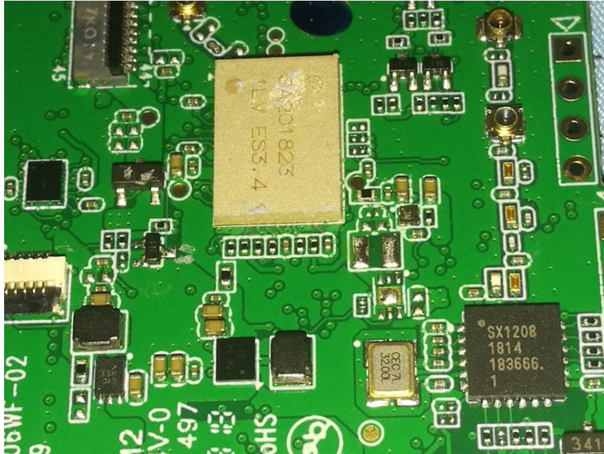
EUT – Main Chip View 5
