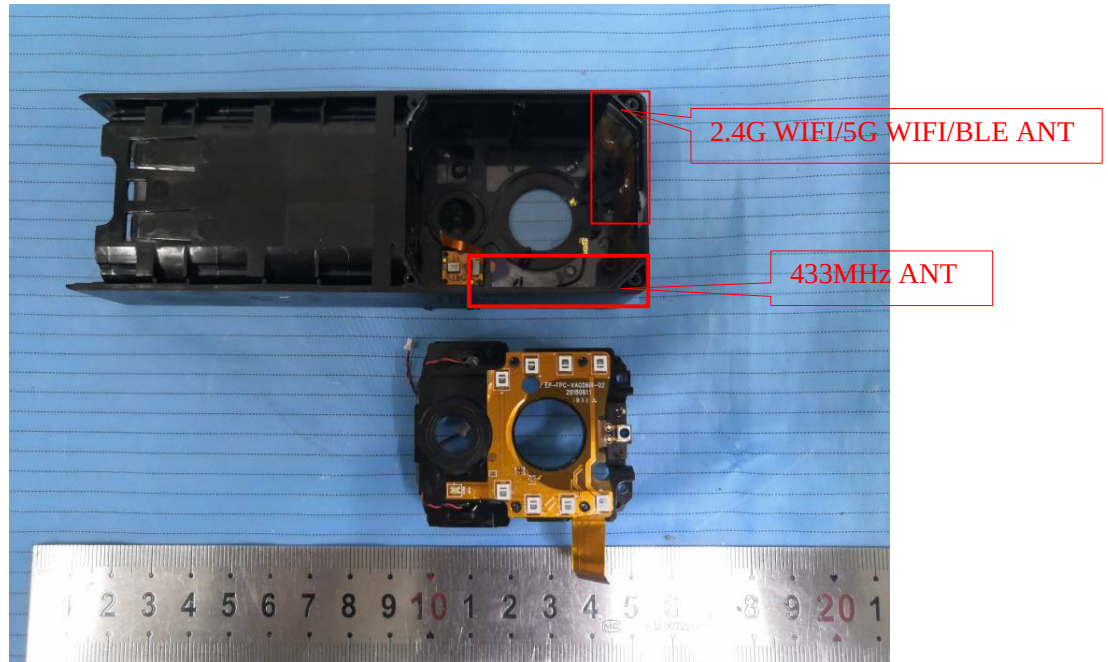
EUT – Cover off View 9
