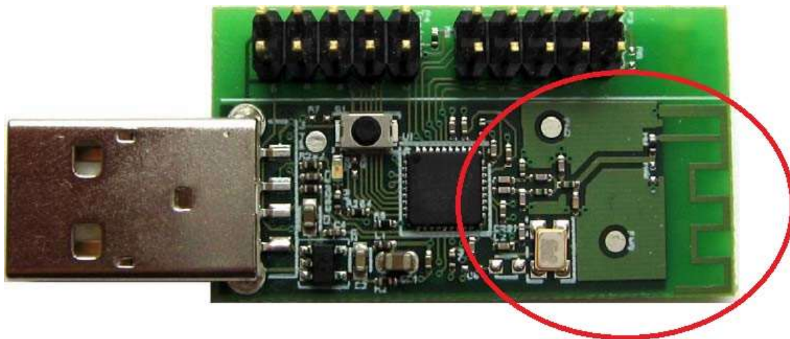
Texas Instruments USB Dongle Reference Design (RF Section Circled)
