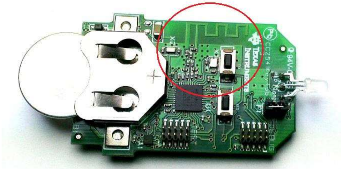
Texas Instruments Keyfob reference design (RF Section Circled)
