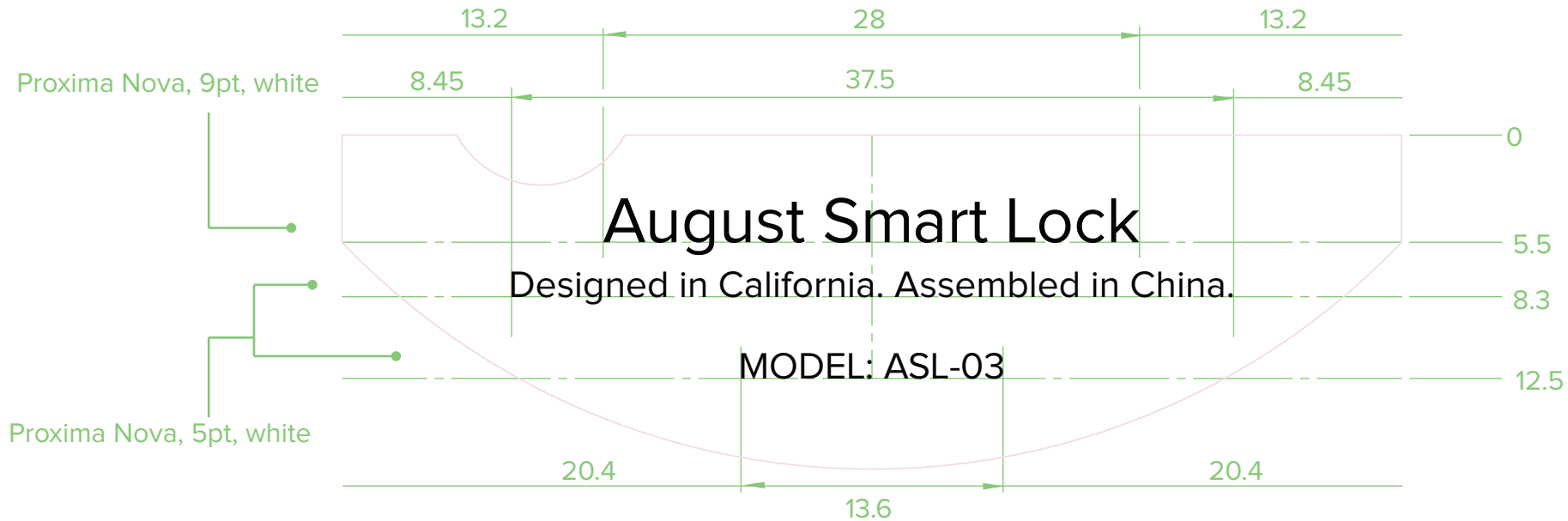
ARTWORK LAYOUT, SCALE 3:1
